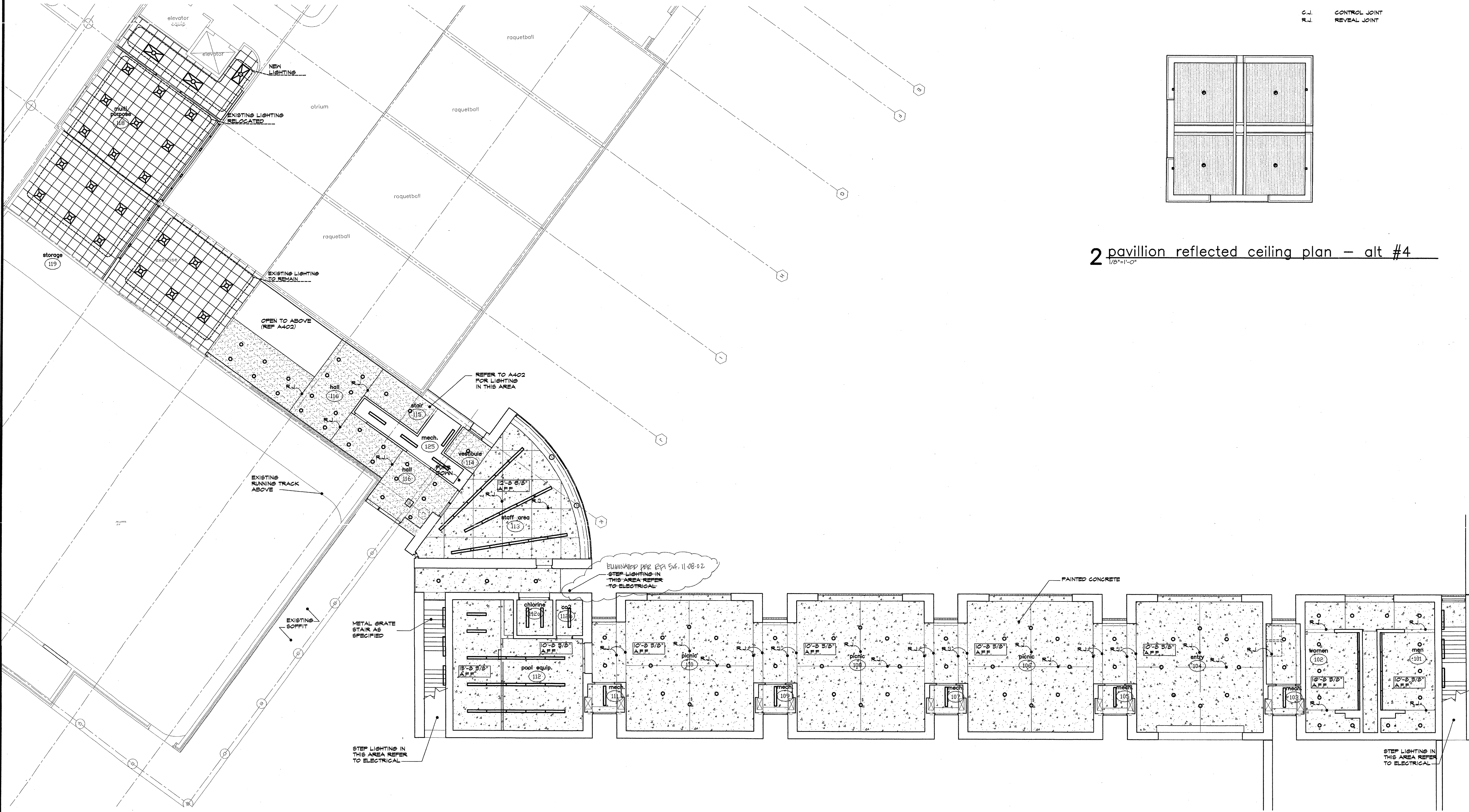
1 lower level reflected ceiling plan 1/8"=1'-0"
