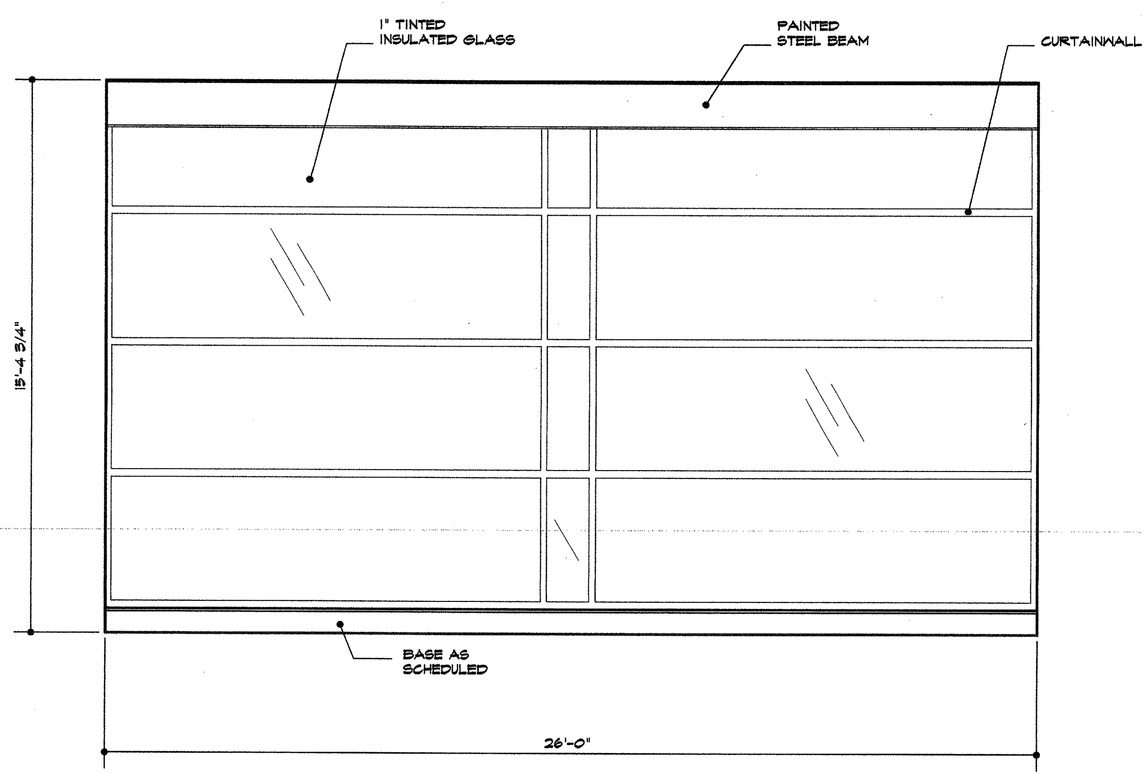
7 interior elevation 3/8"=1'-0"
