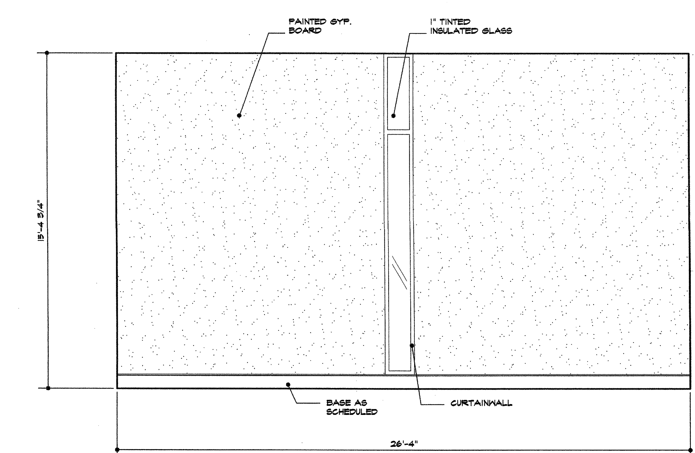
3 interior elevation - rm. #211 3/8"=1'-0"
