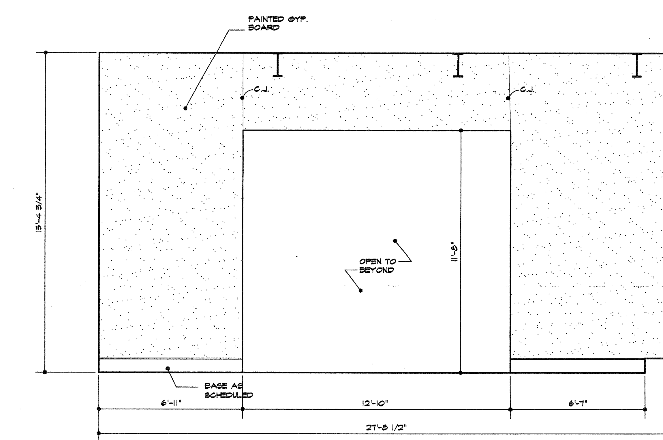
6 interior elevation 3/8"=1'-0"
