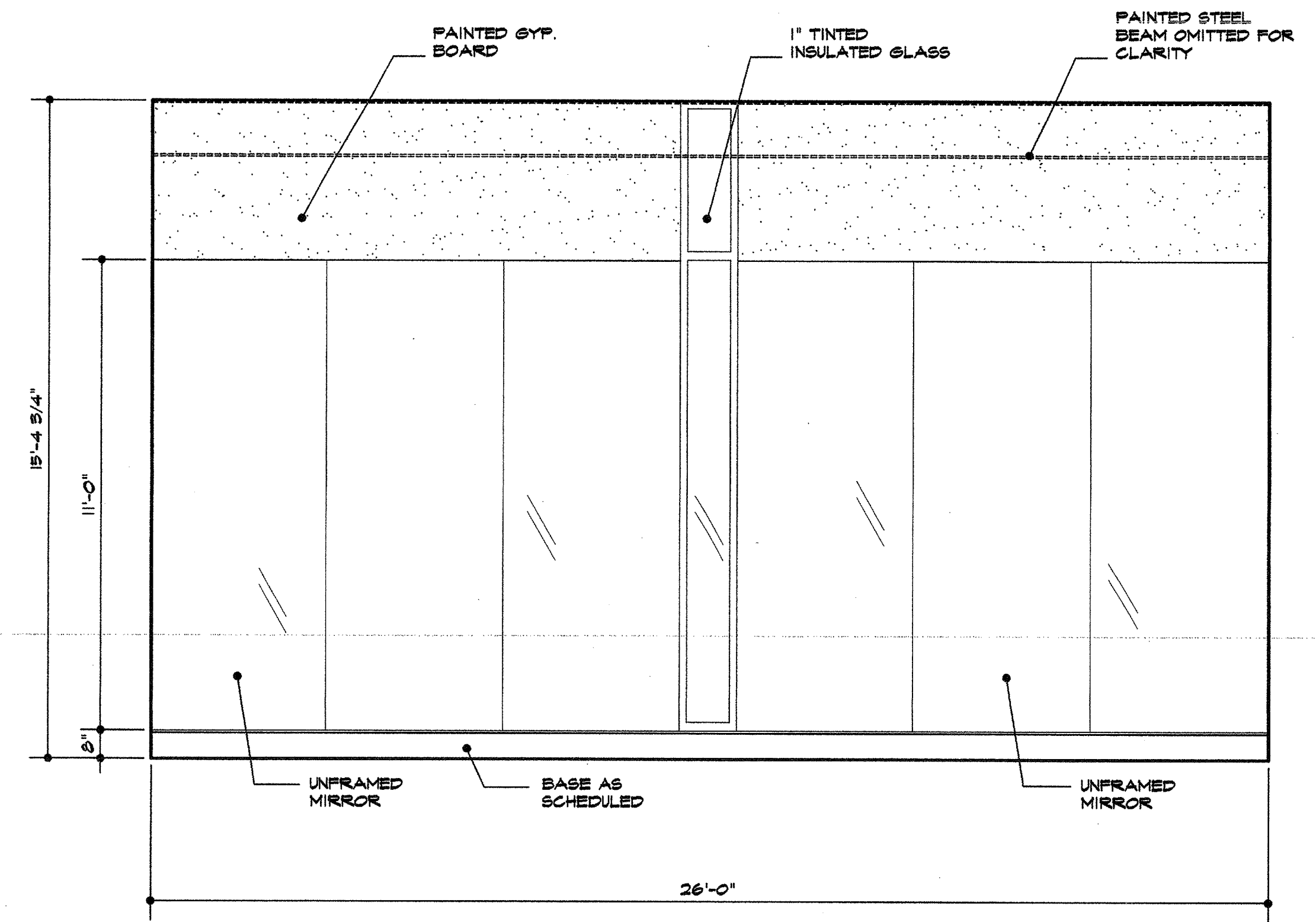
8 interior elevation 3/8"=1'-0"
