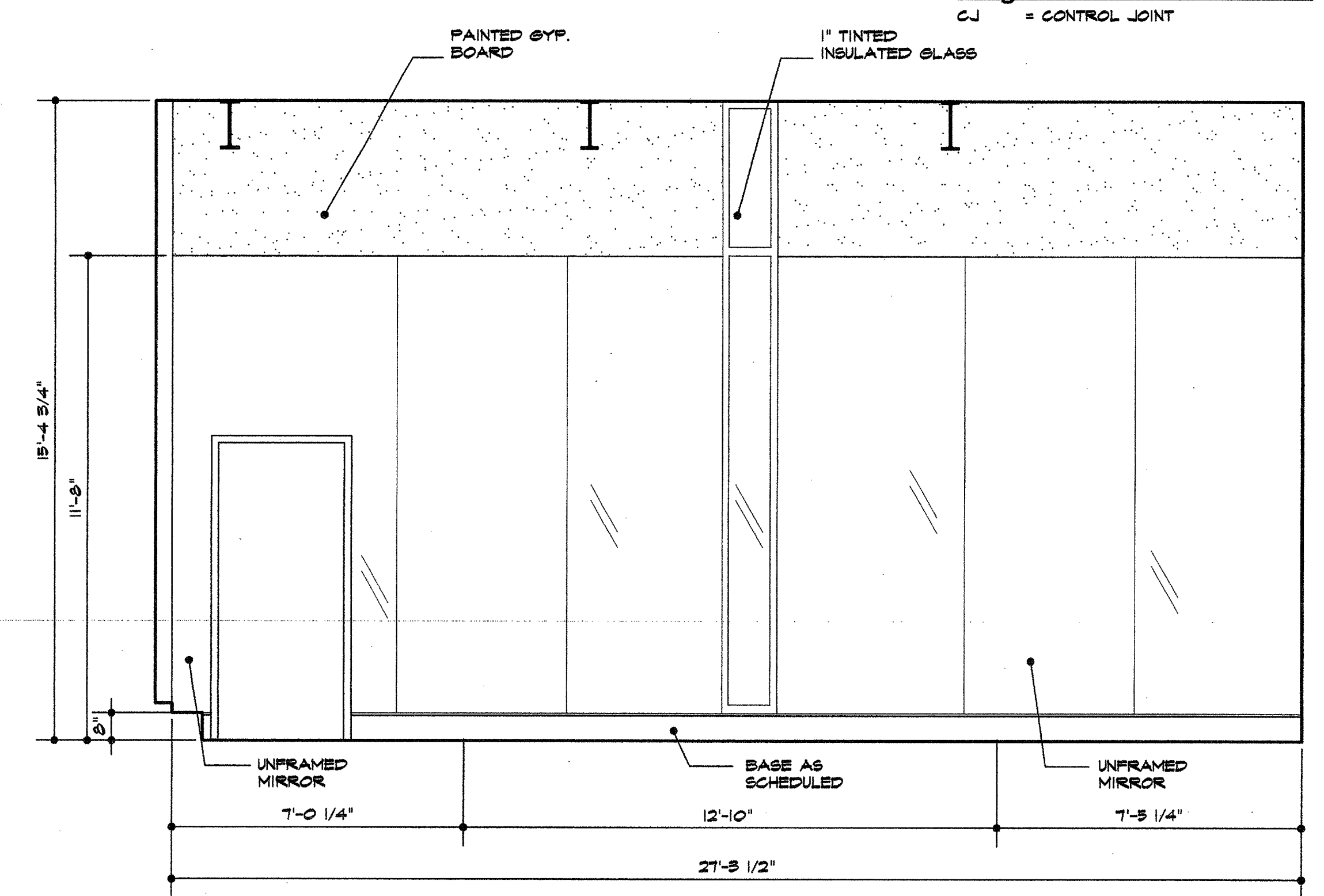
9 interior elevation - rm. #201 3/8"=1'-0"
