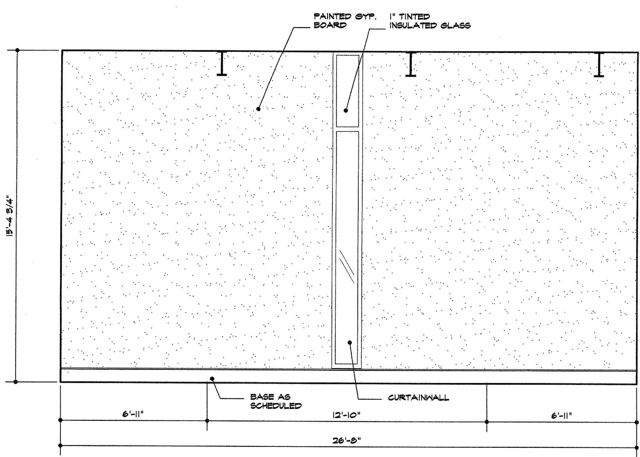
4 interior elevation - rm. #211 3/8"=1'-0"
