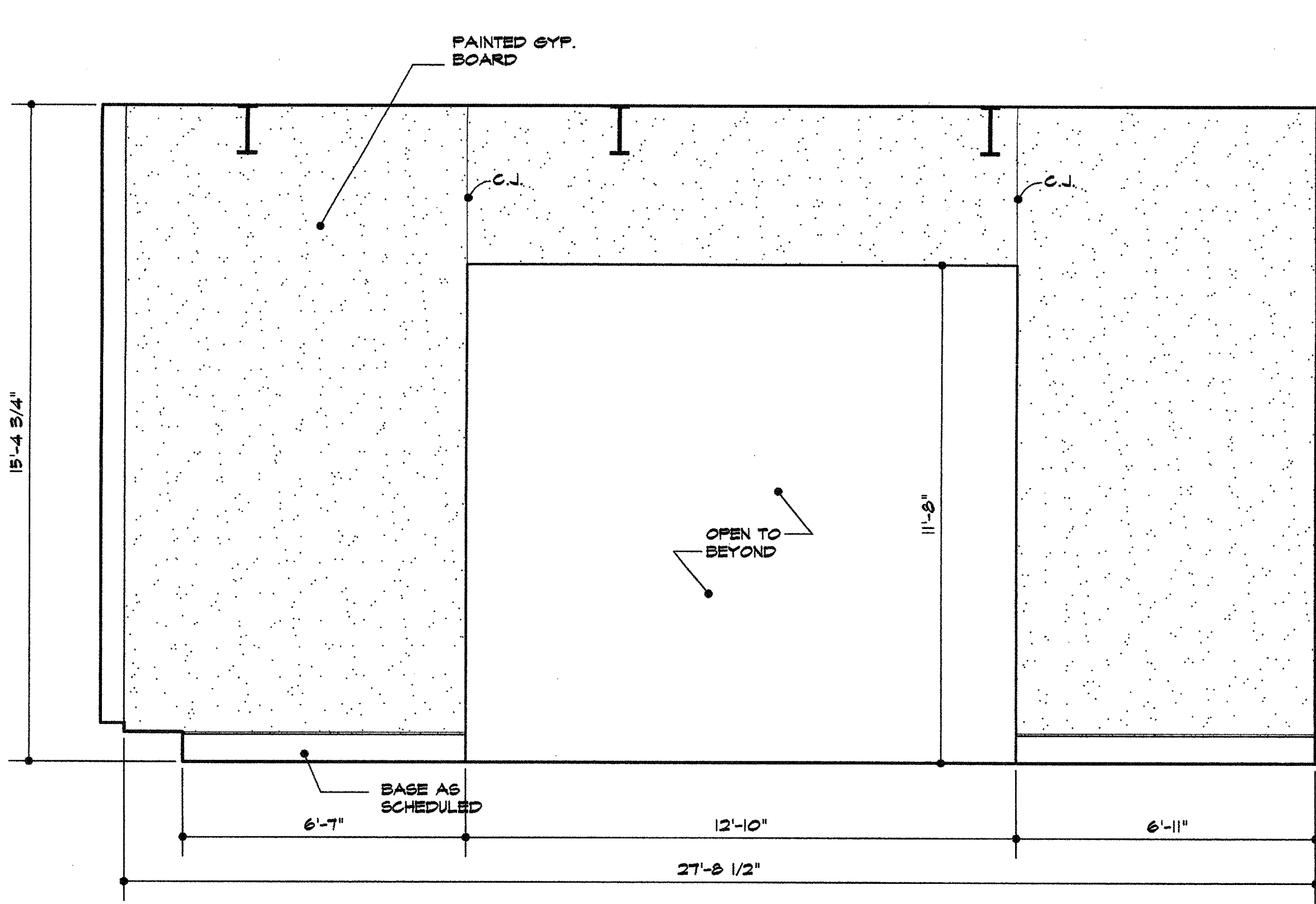
5 interior elevation 3/8"=1'-0"
