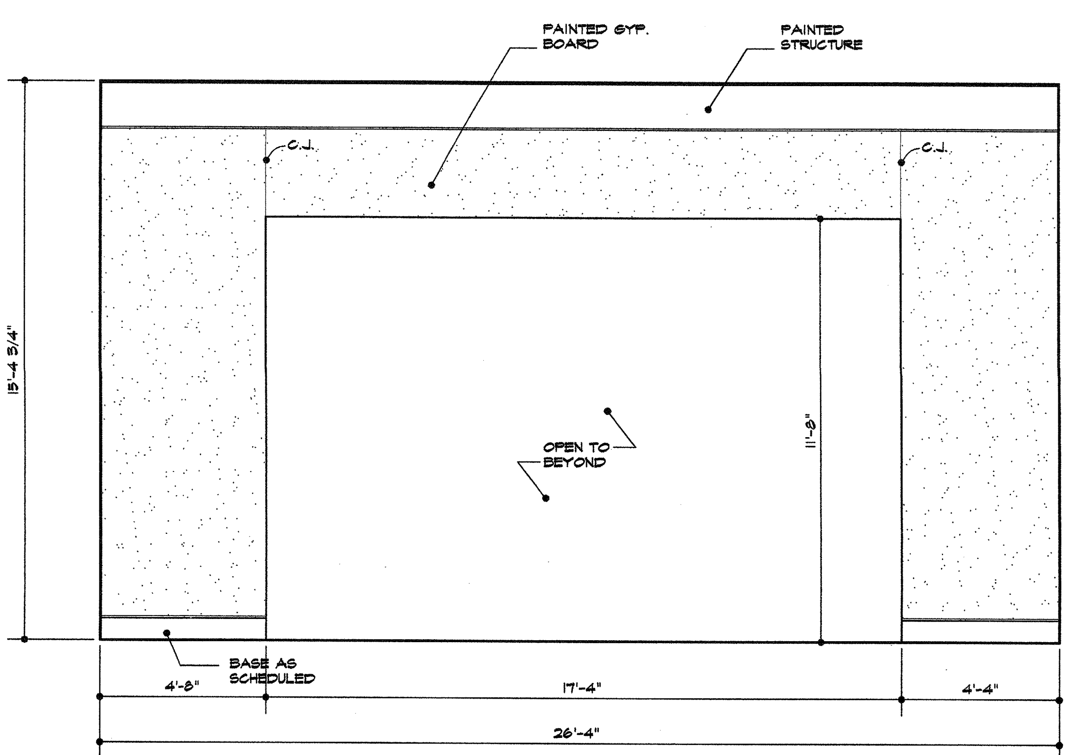
1 interior elevation - rm. #211 3/8"=1'-0"
