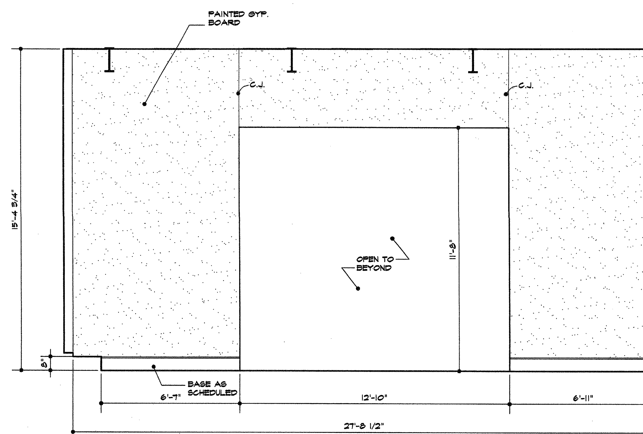
2 interior elevation - rm. #211 3/8"=1'-0"
