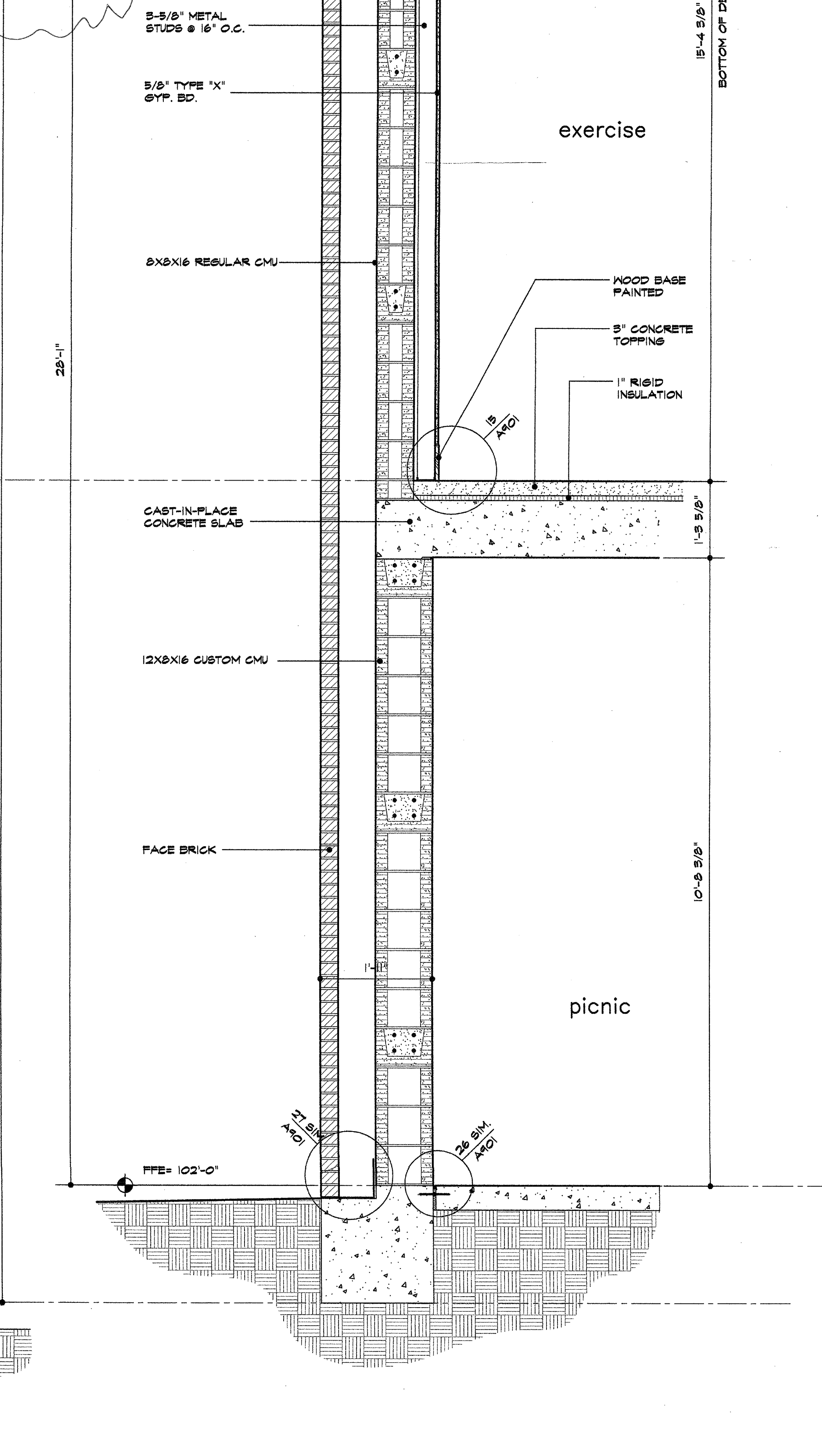
3 wall section 3/4"=1'-0"
