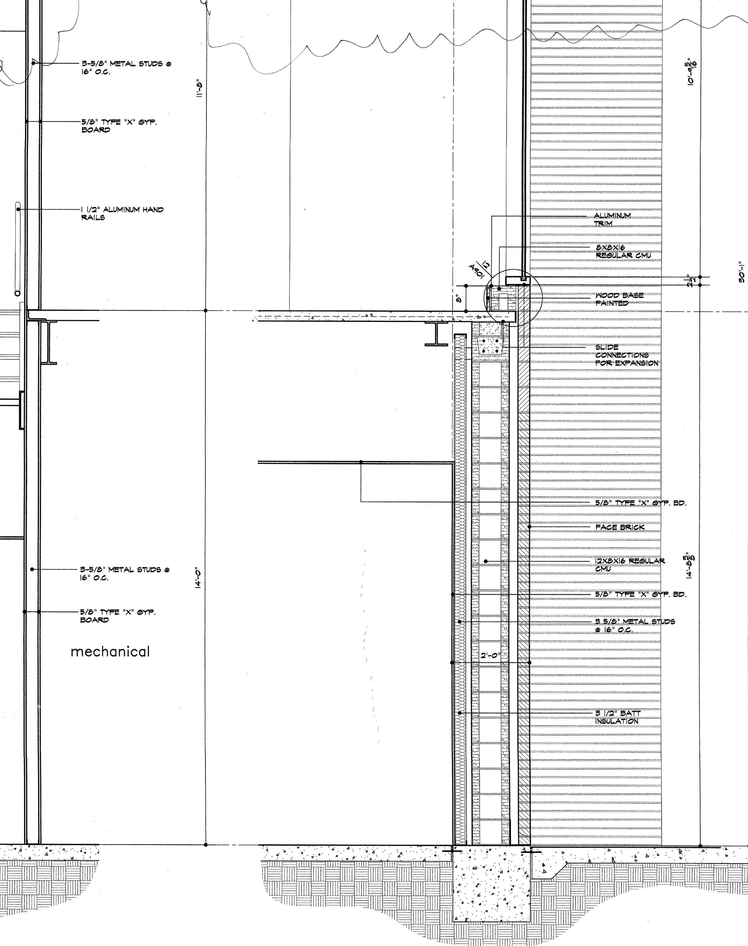
2 wall section 3/4"=1'-0"
