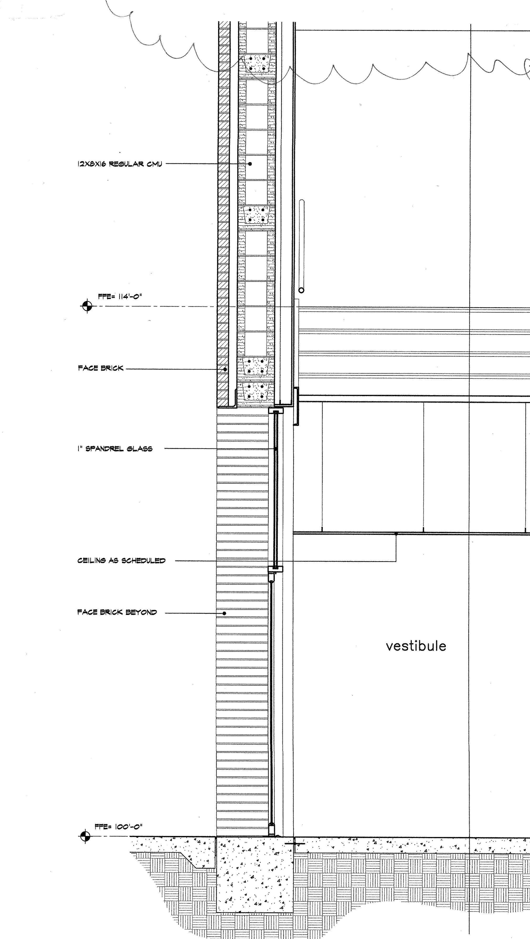
1 wall section 3/4"=1'-0"
