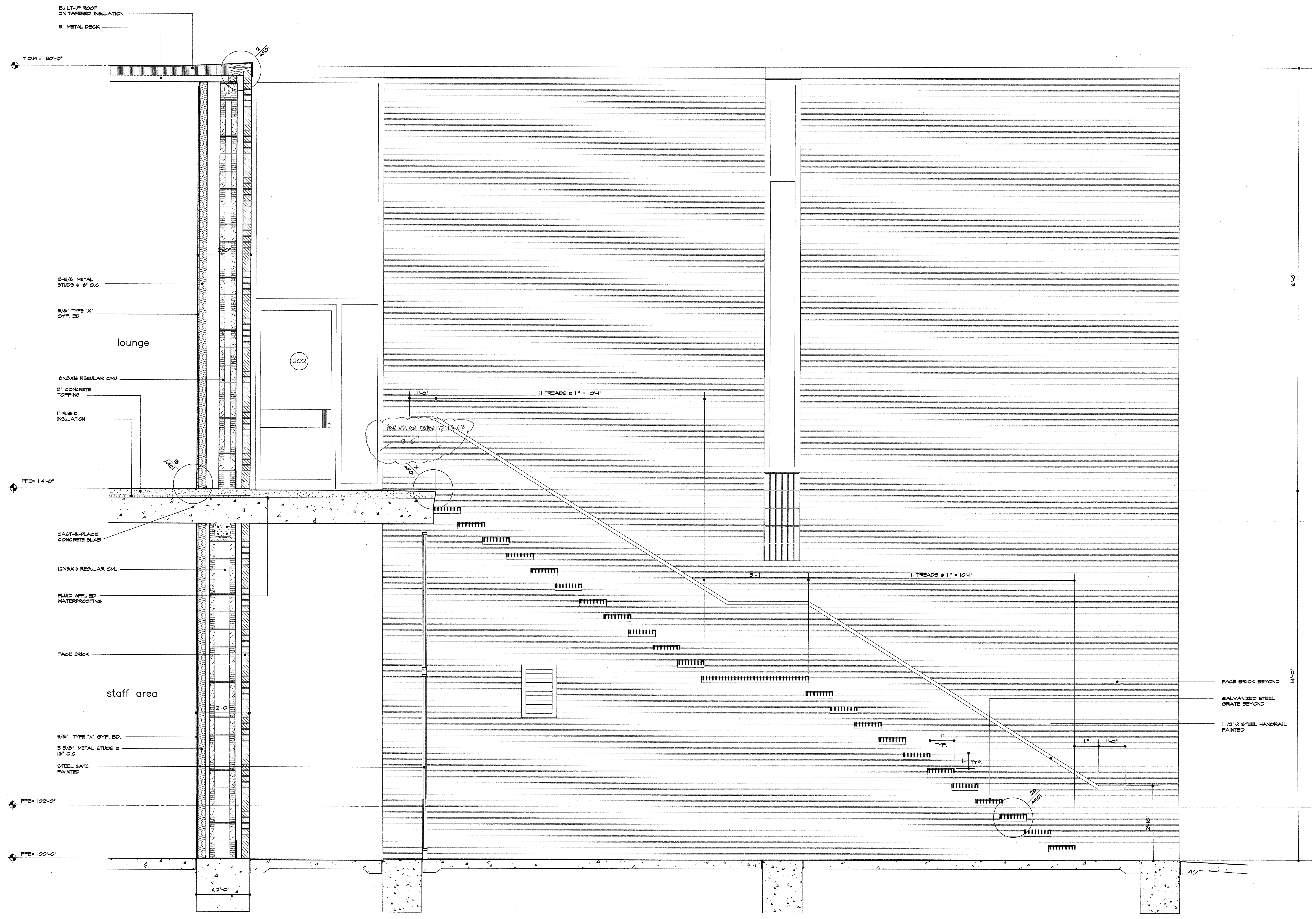
1 wall section 3/4"=1'-0"
