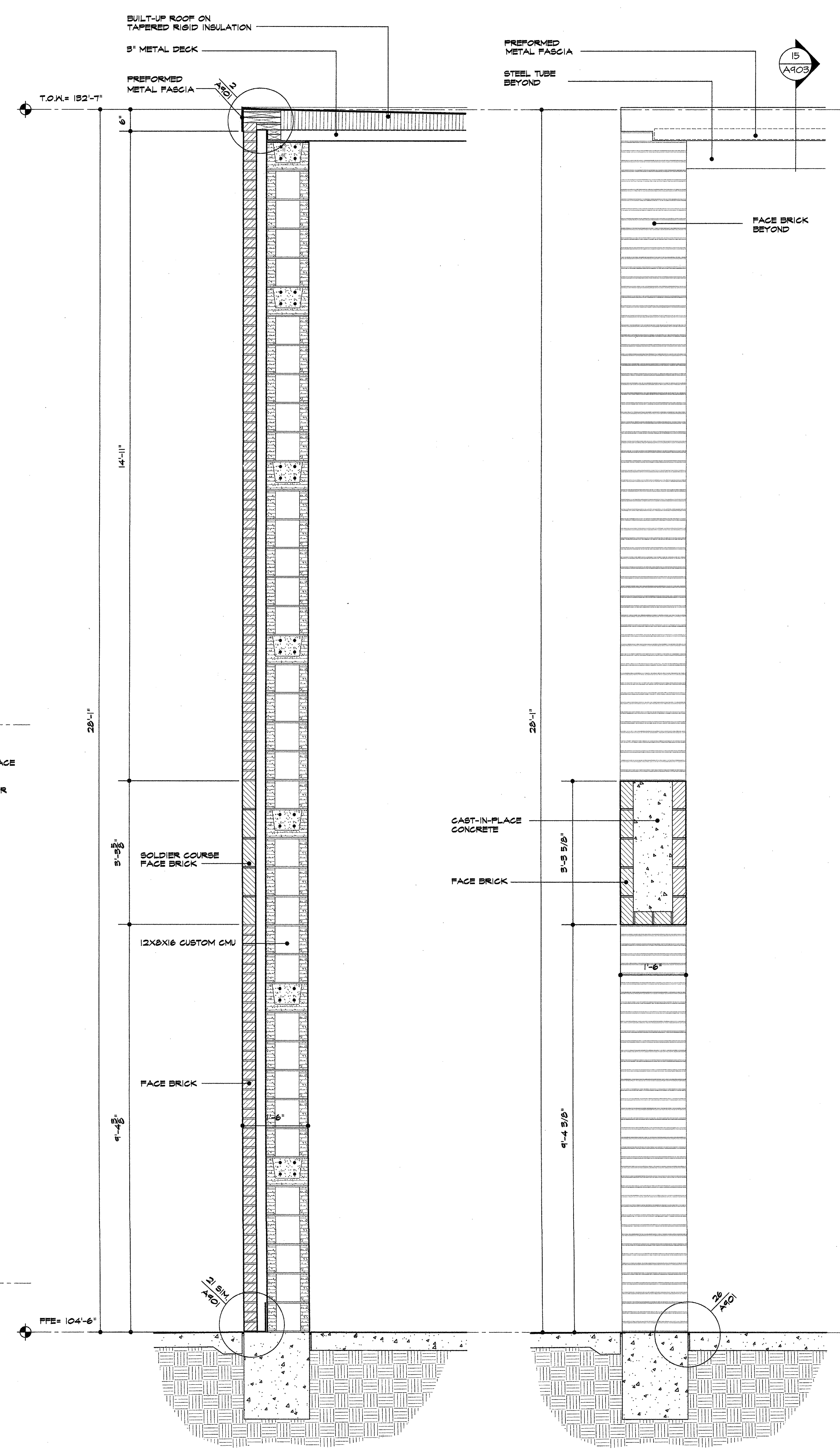
3 wall section 3/4"=1'-0"
