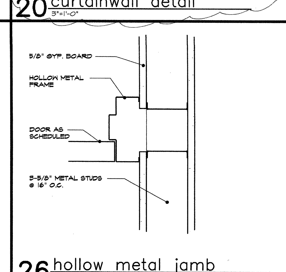
20 curtainwall detail 3/4" x 1"
