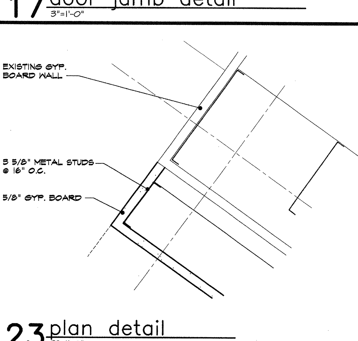
17 door jamb detail 3/4" x 1"
