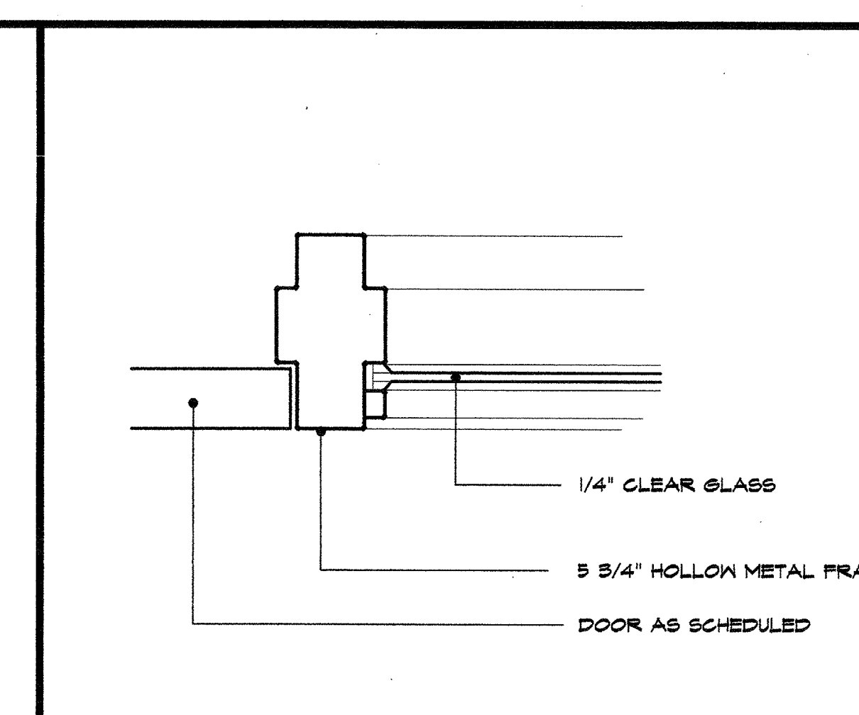
4 door jamb detail 3/4" x 1"
