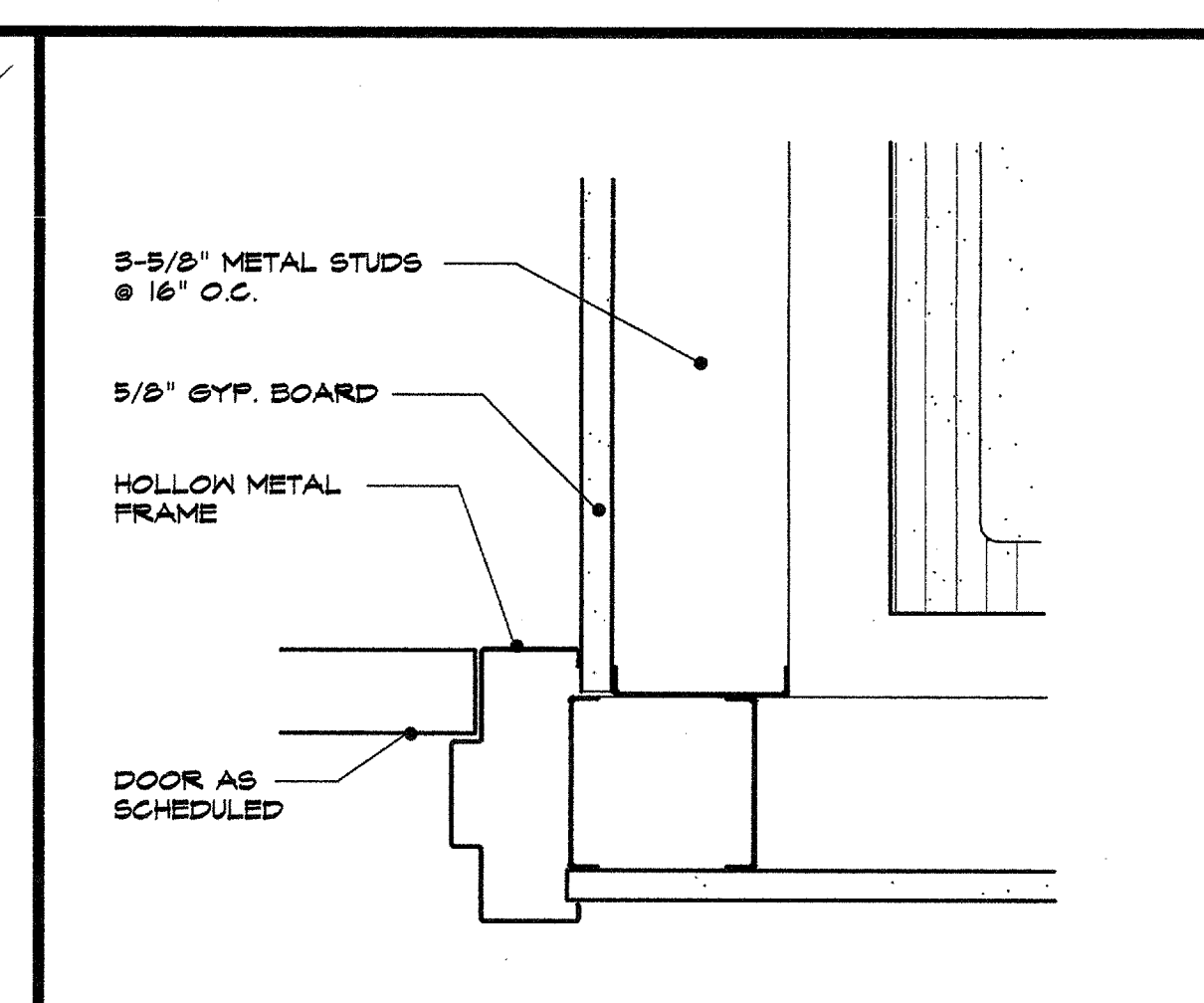
3 door jamb detail 3/4" x 1"
