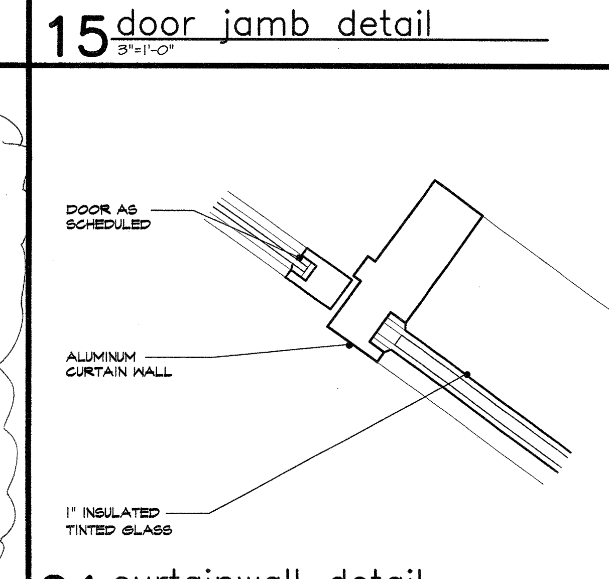
15 door jamb detail 3/4" x 1"
