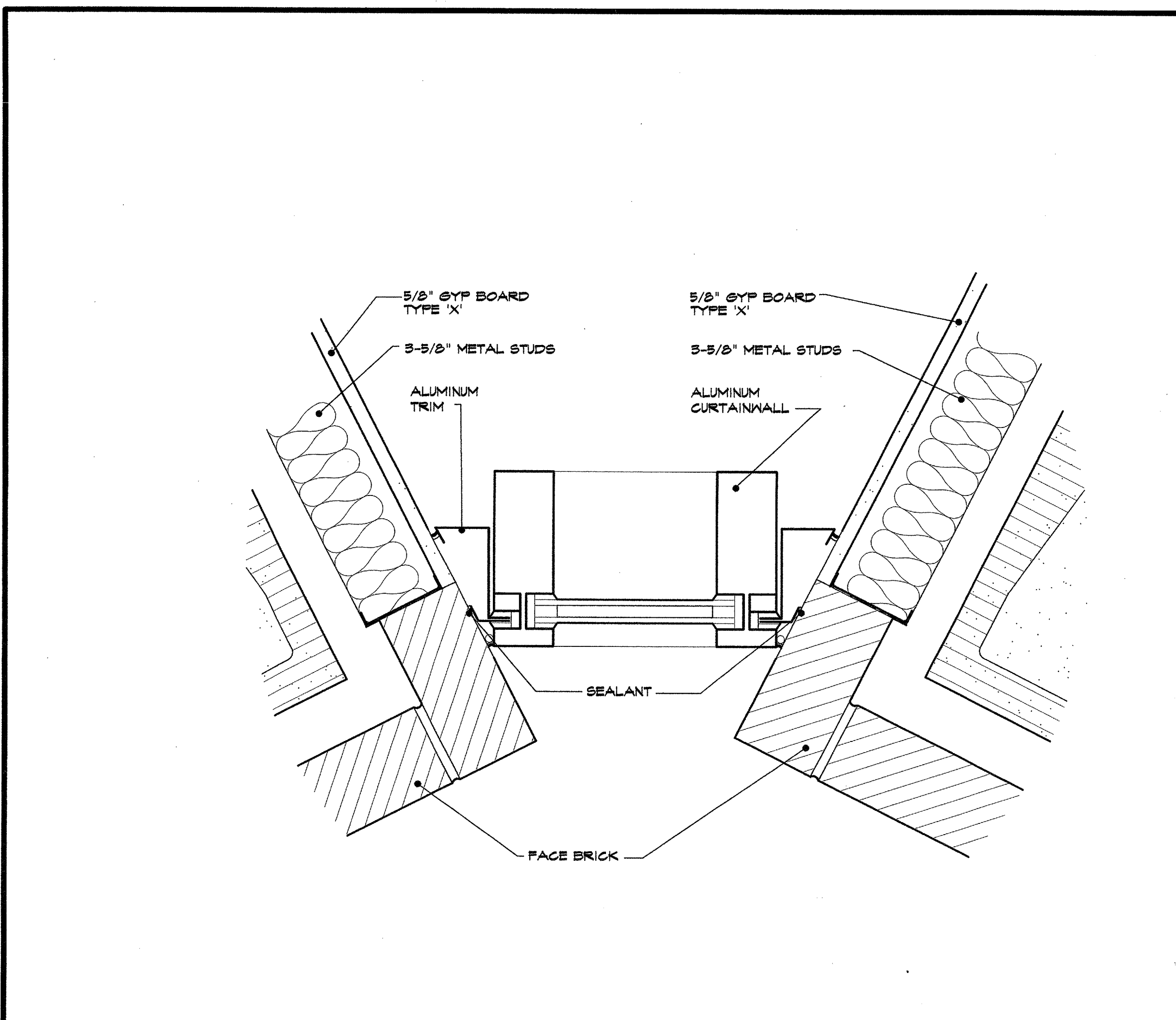
1 curtainwall jamb detail 3/4" x 1"
