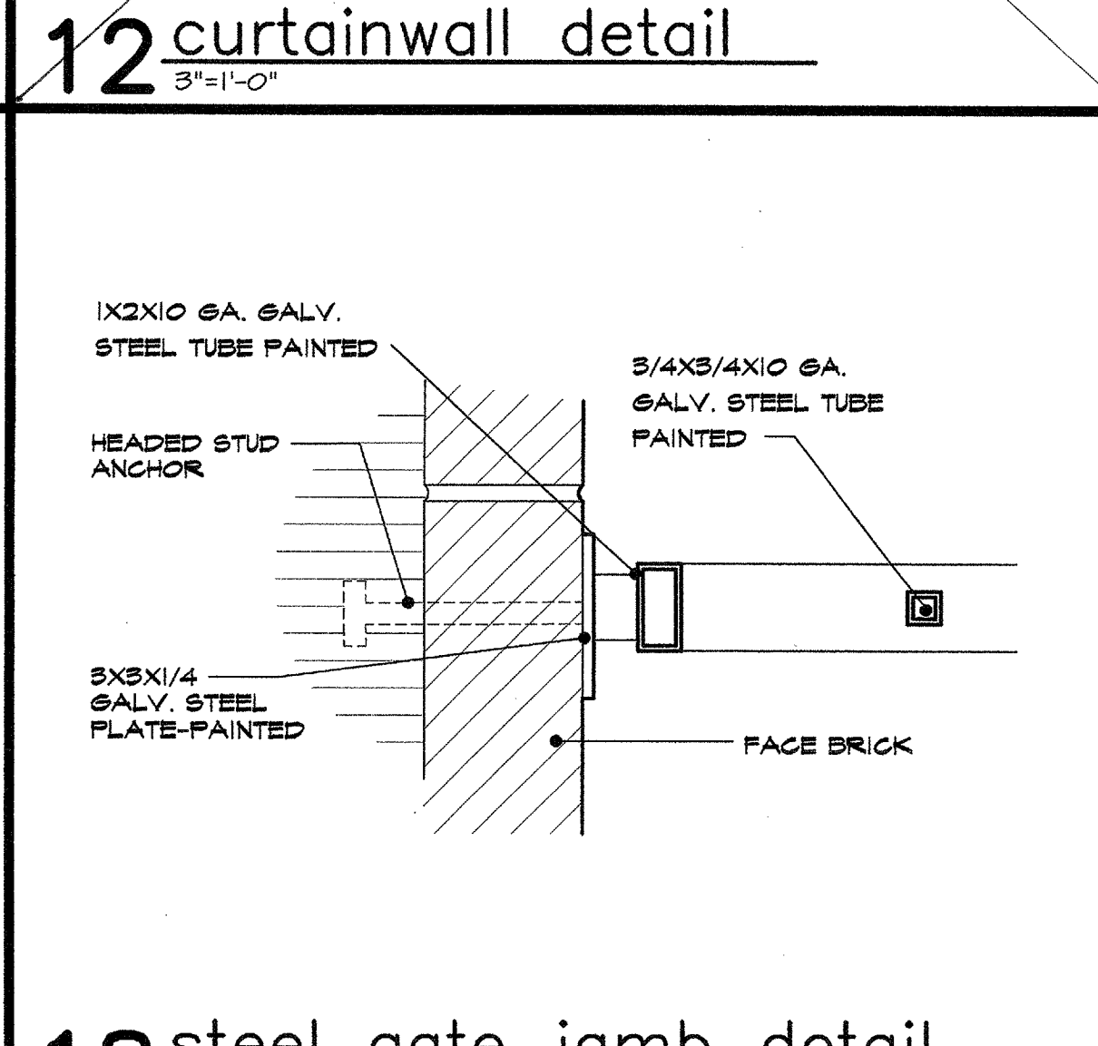
12 curtainwall detail 3/4" x 1"
