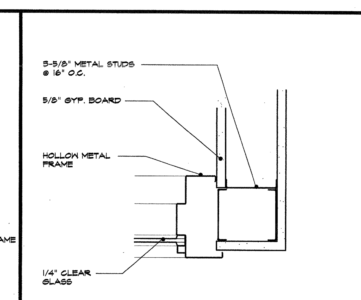
5 hollow metal jamb 3/4" x 1"
