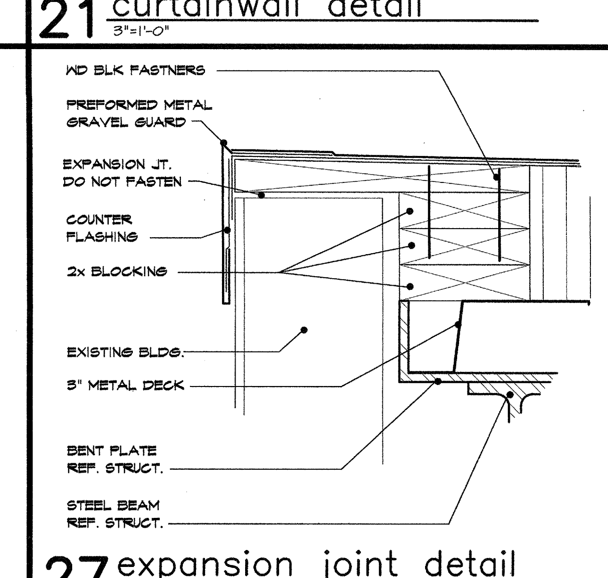
21 curtainwall detail 3/4" x 1"
