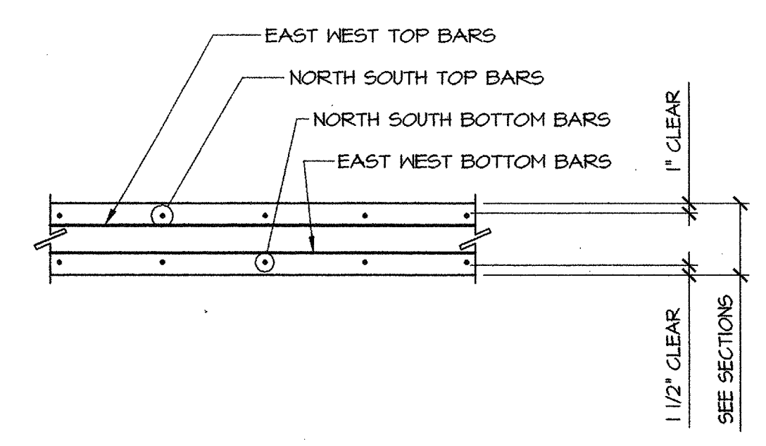
TYPICAL BAR PLACEMENT
