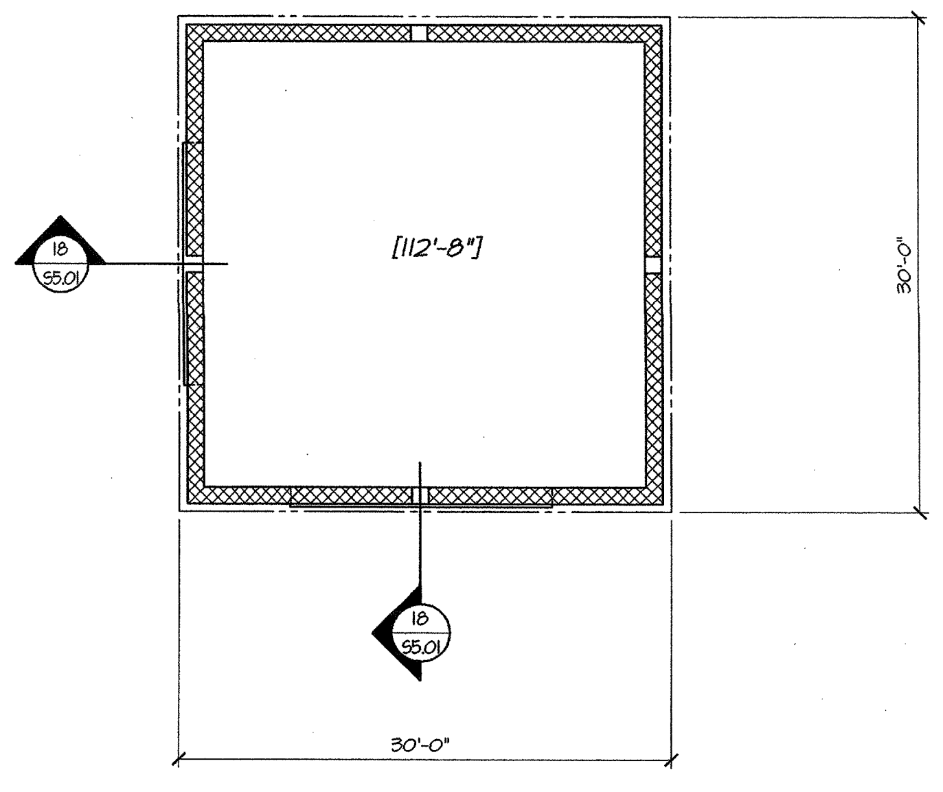
02 NORTH PAVILLION INTERMEDIATE FRAMING PLAN 1/8"=1'-0"
