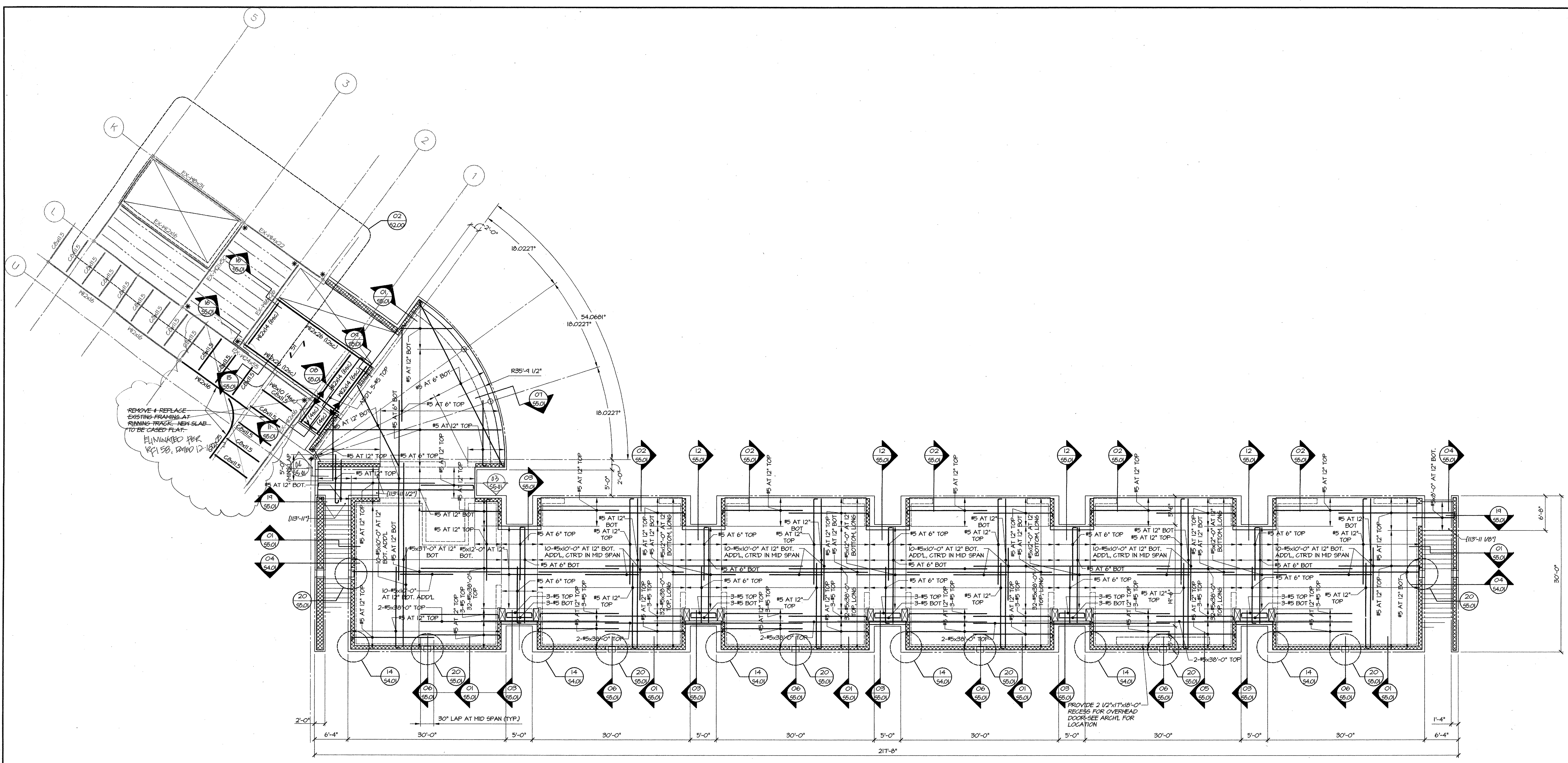
PLAN NORTH 01 SECOND FLOOR FRAMING PLAN 1/8"=1'-0"
