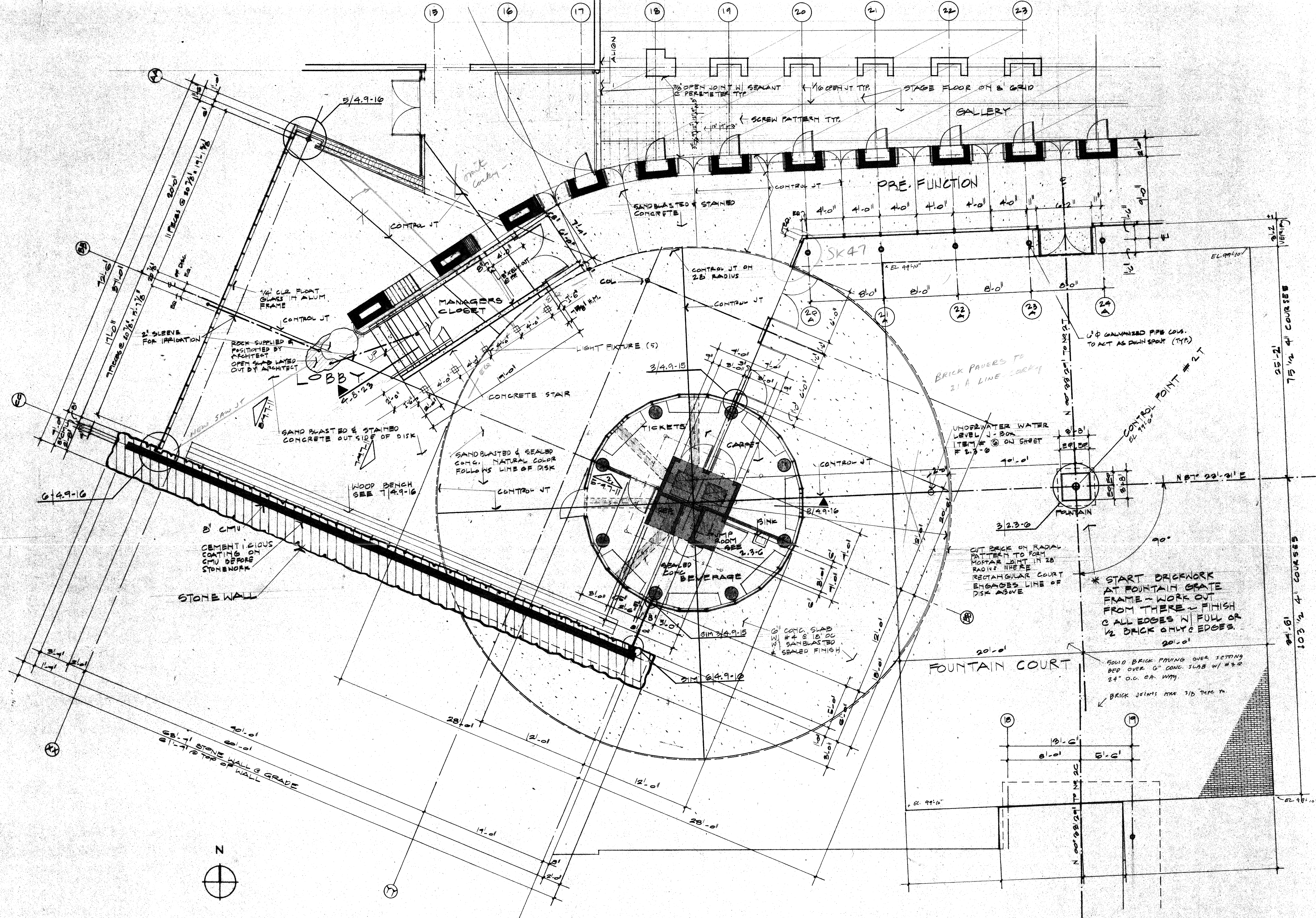
1 ENLARGED LEVEL ONE FLOOR PLAN
