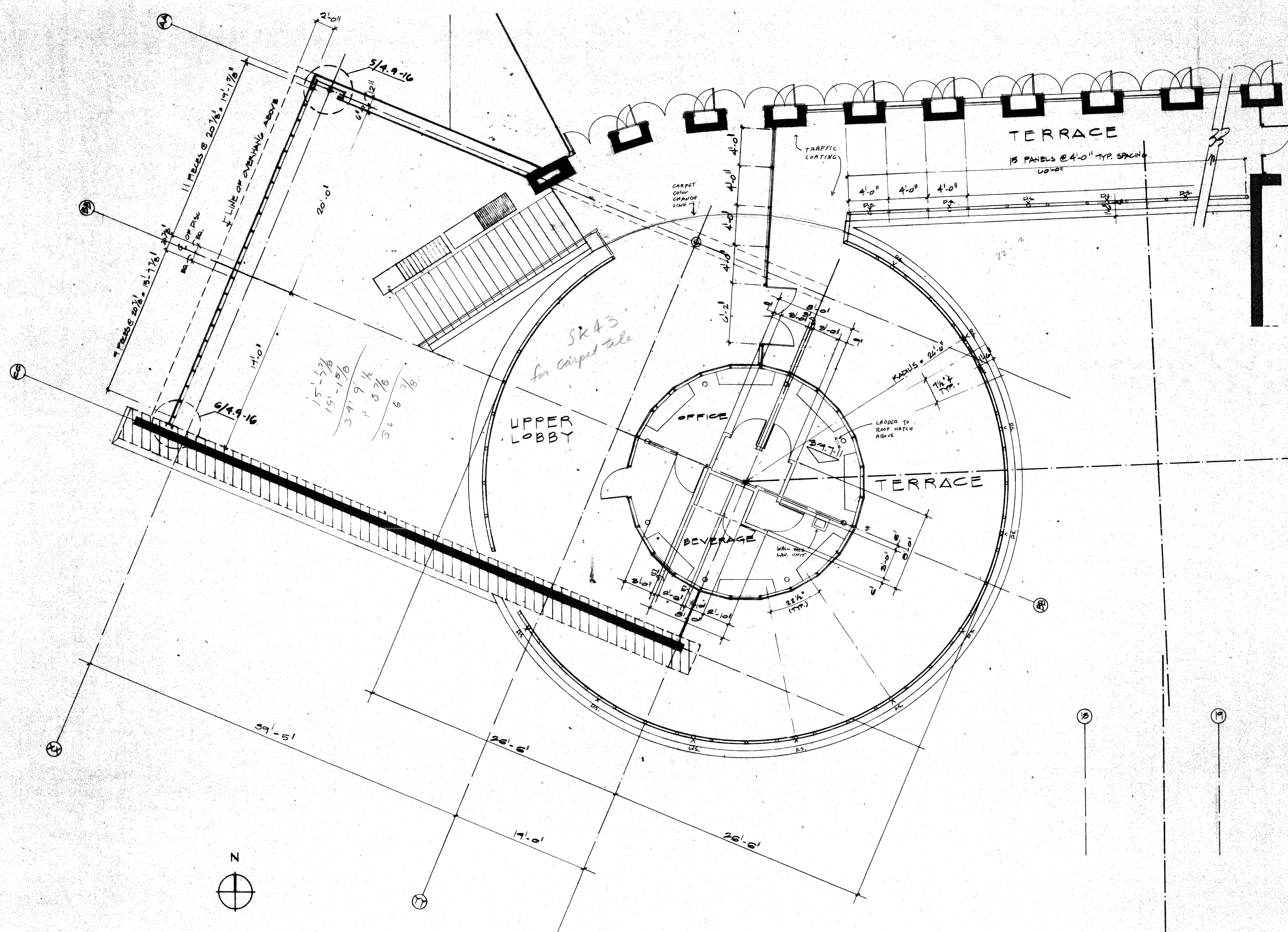
1 ENLARGED LEVEL TWO FLOOR PLAN 1/2" = 1'-0"
