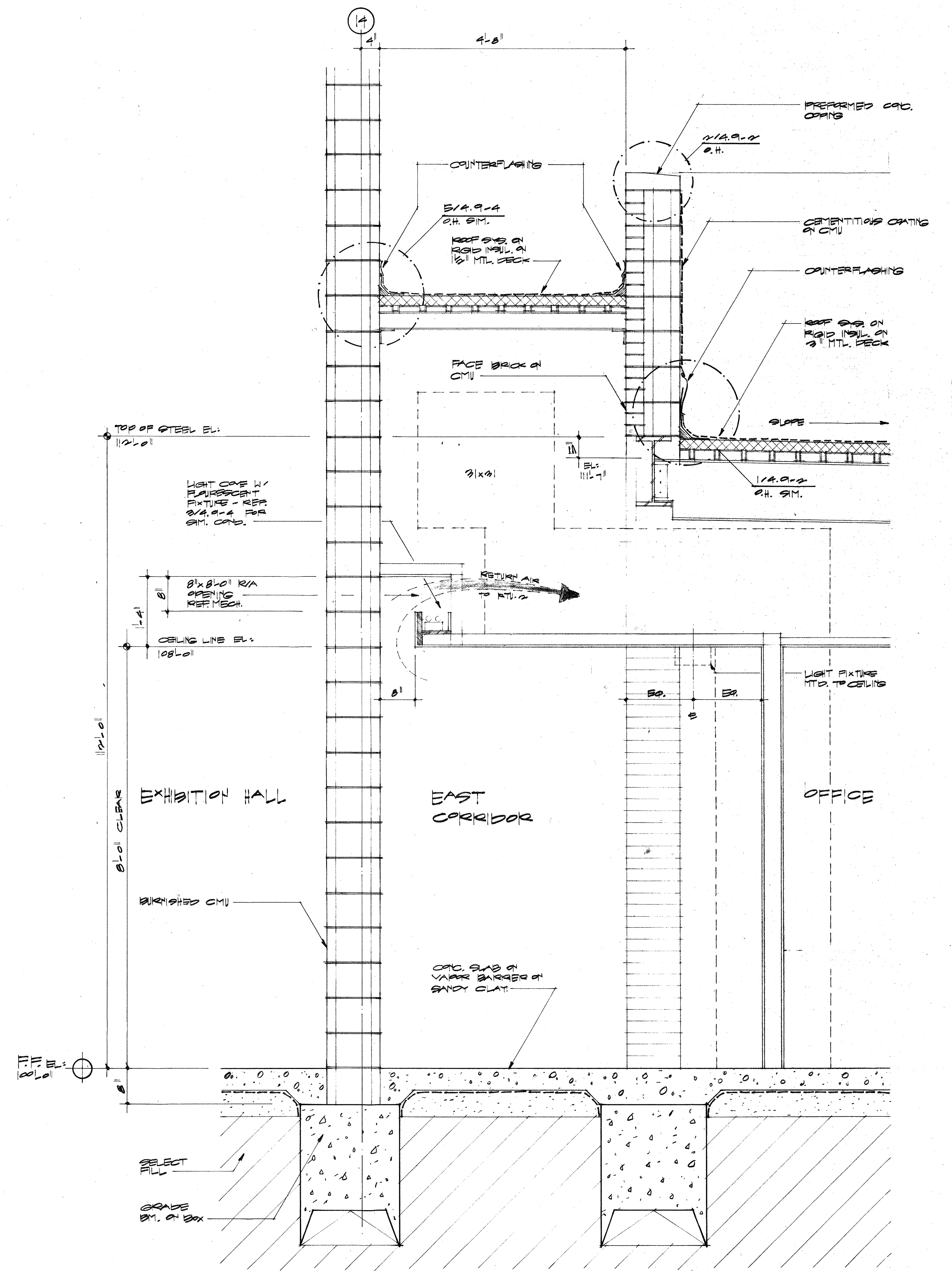
1 DETAIL 1/2" = 1'-0"
