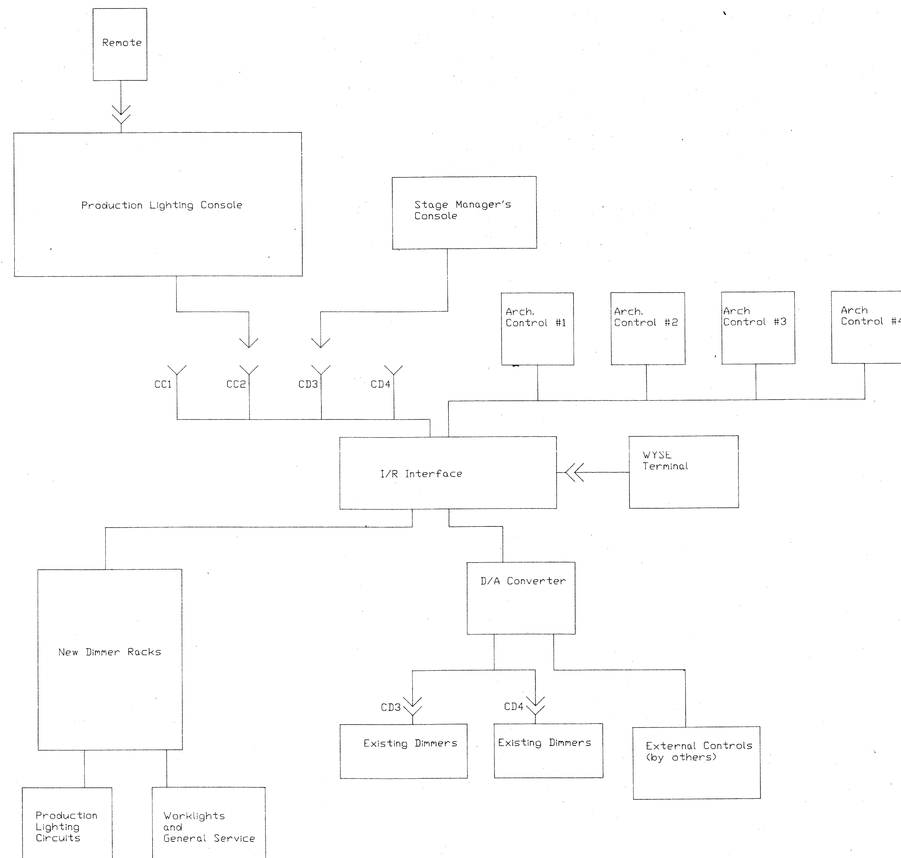
1 Lighting Control Riser
