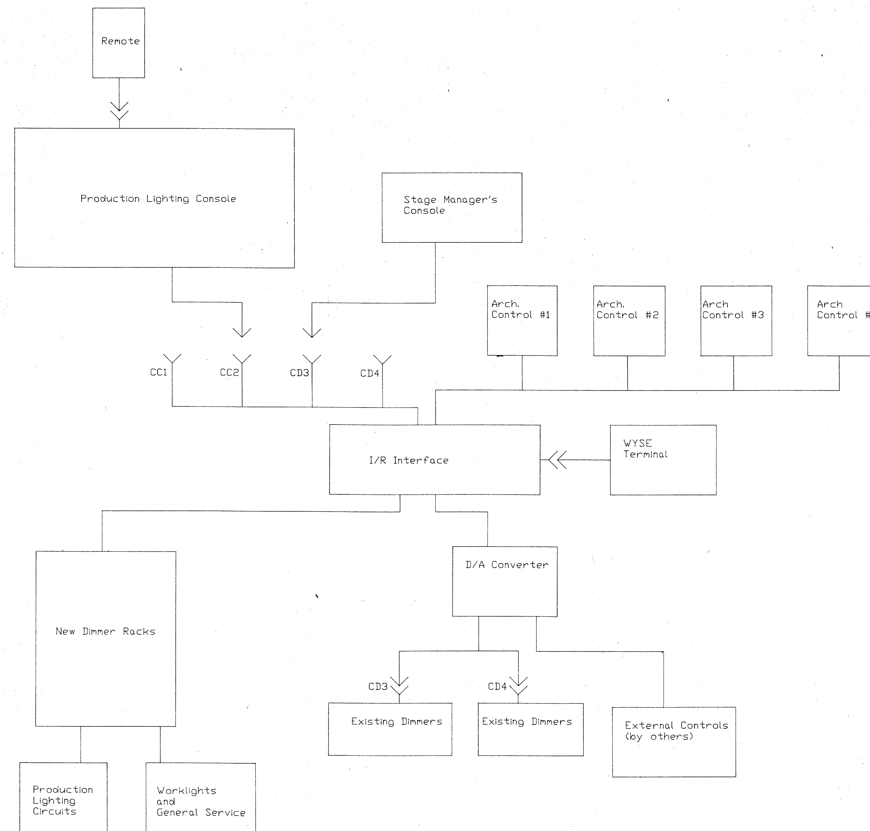
① Lighting Control Riser
