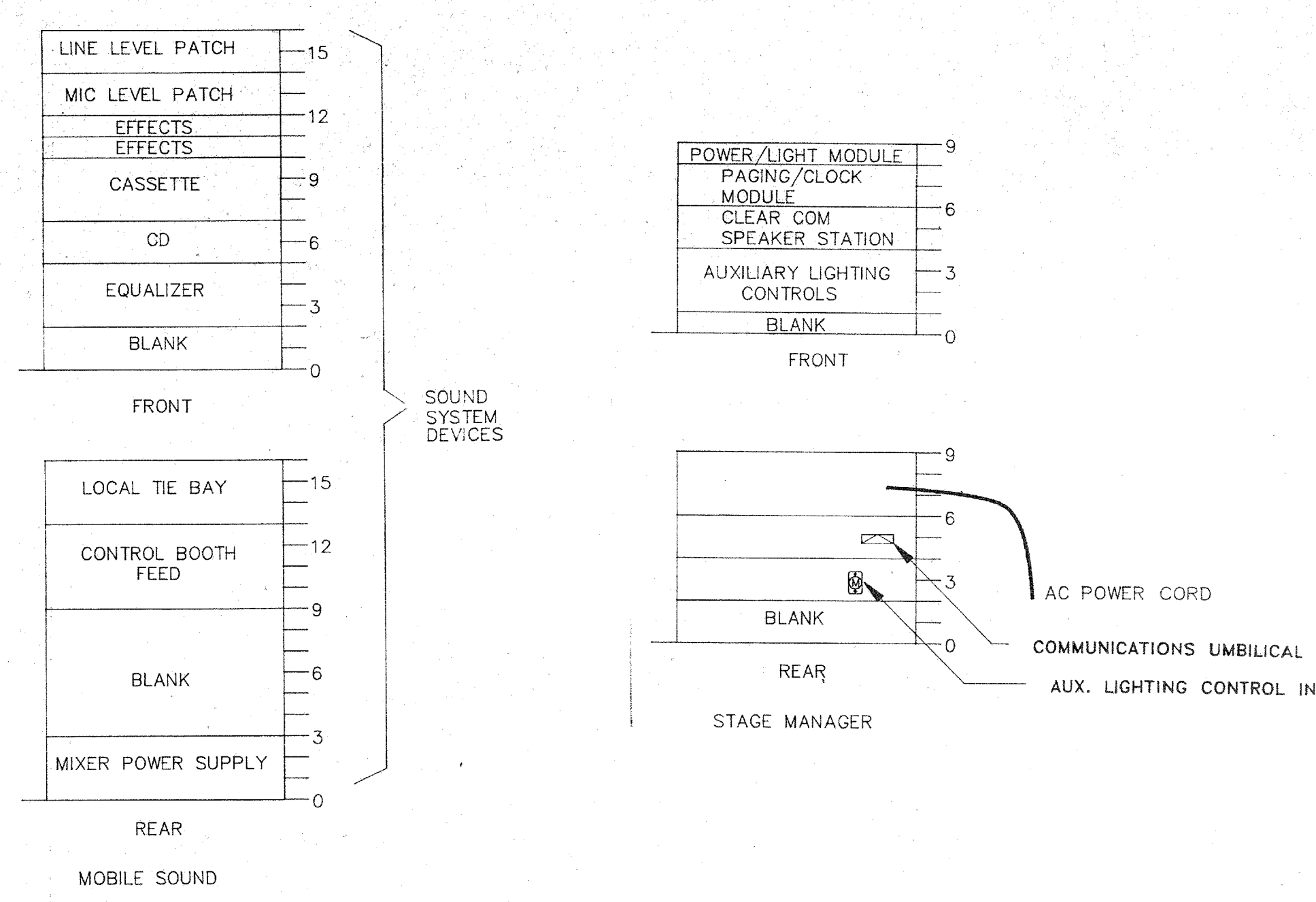
F RACK ELEVATIONS
