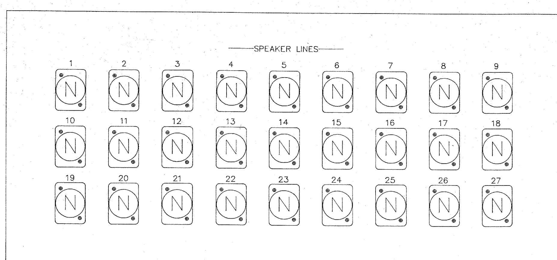
F SPEAKER SECTION - 19" RACK X 5 RACK UNITS
