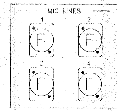
F MIC RECEPT. BACK BOX 2 GANG
