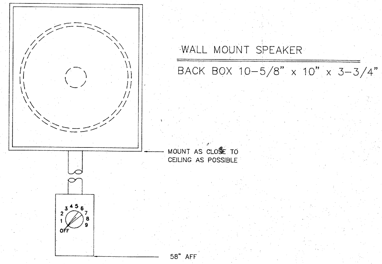
J PAGE SPEAKER WITH VOLUME CONTROL BACK BOX 1 GANG SCALE: 1:4
