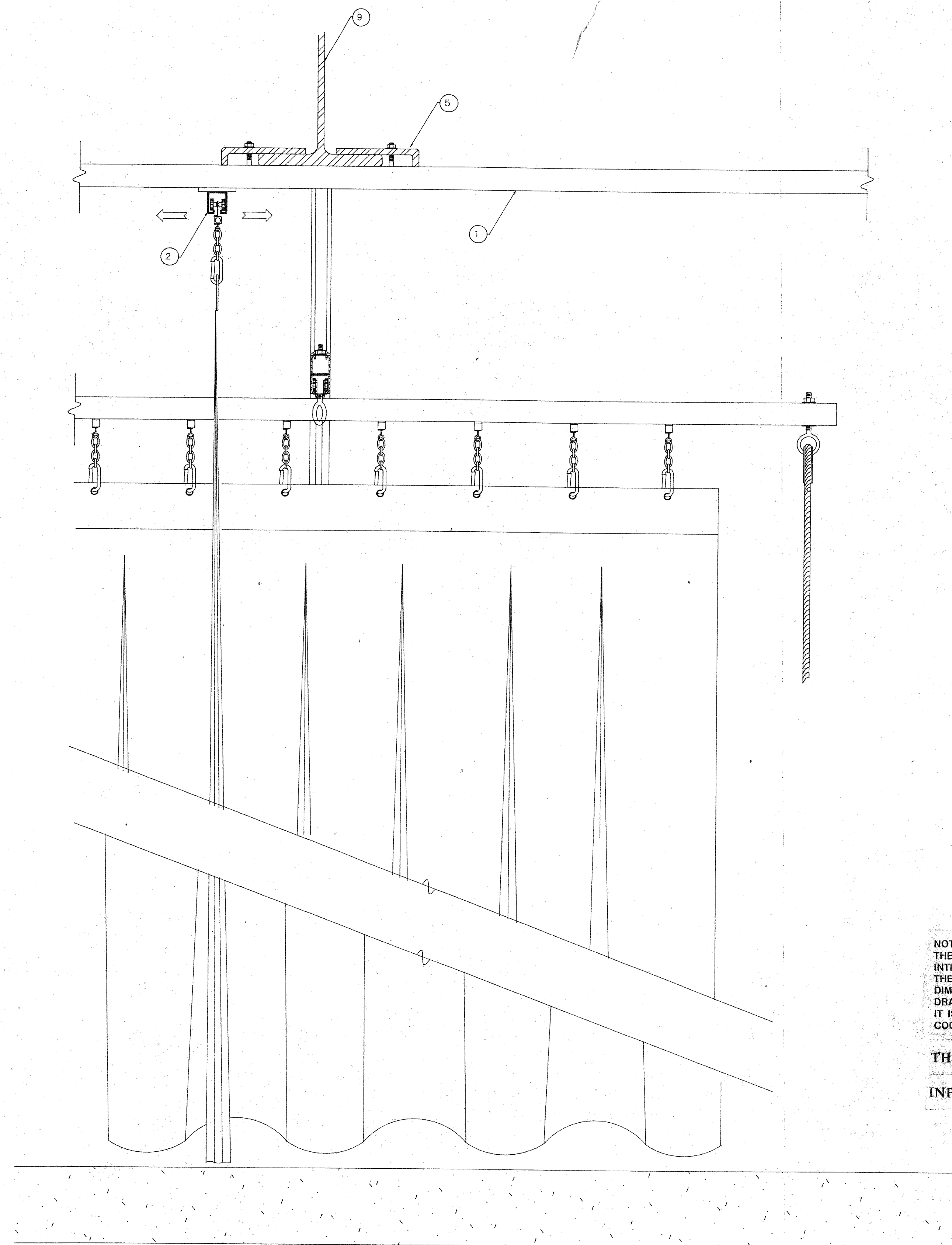
C2 CURTAIN TRACK DETAILS SCALE: 3/4"=1'-0"
