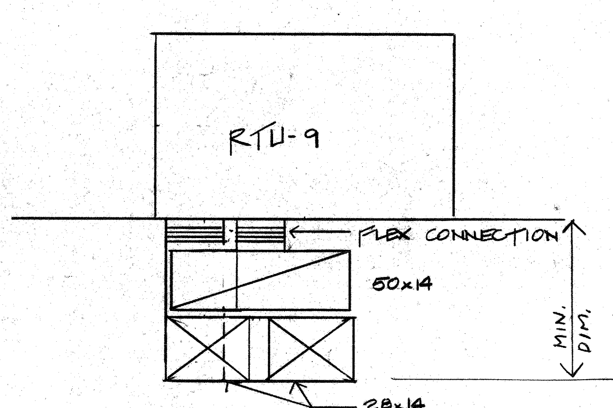
A SECTION NO SCALE
