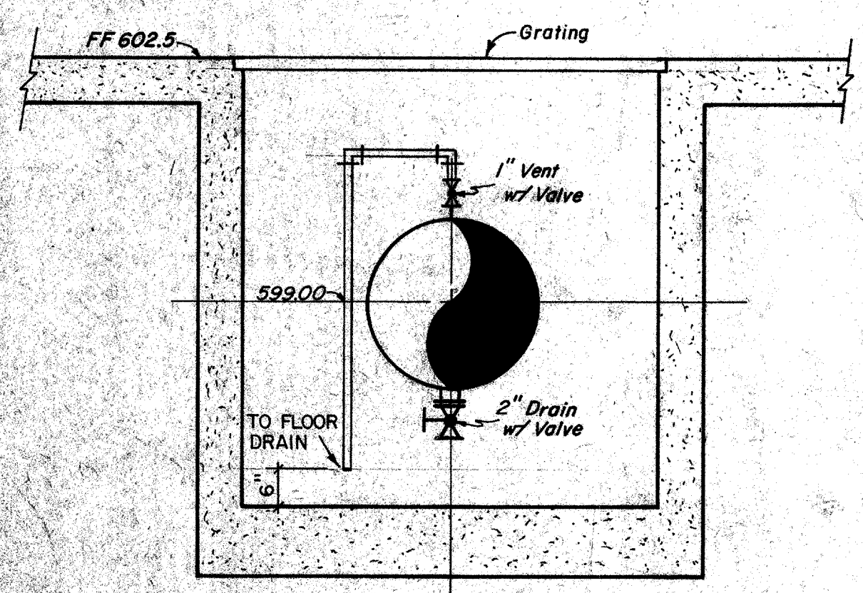
2 SECTION 1/2" = 1'-0"
