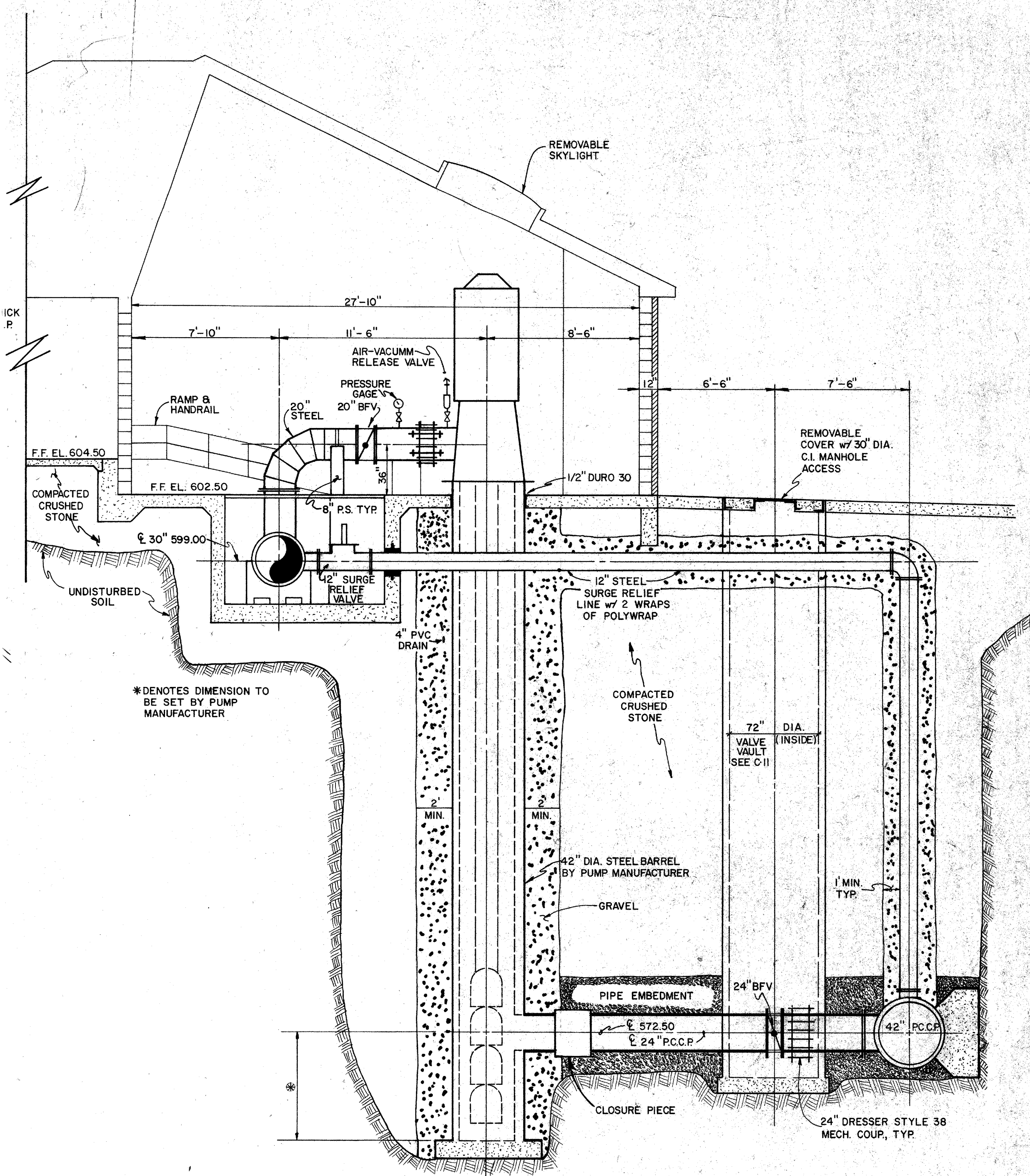
1 SECTION 1/4" = 1'-0"
