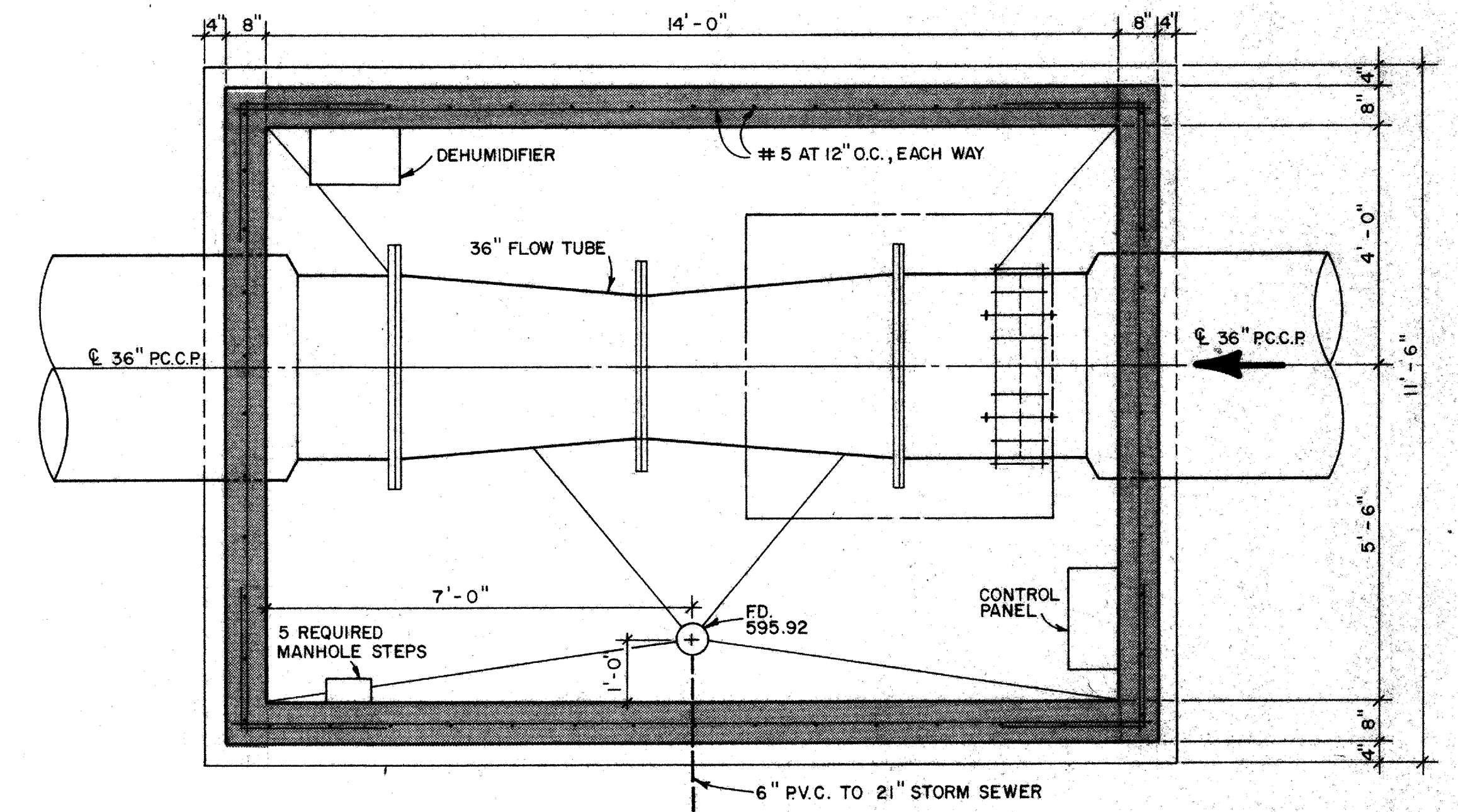
SECTIONAL PLAN SCALE - 1/2" = 1'-0"
