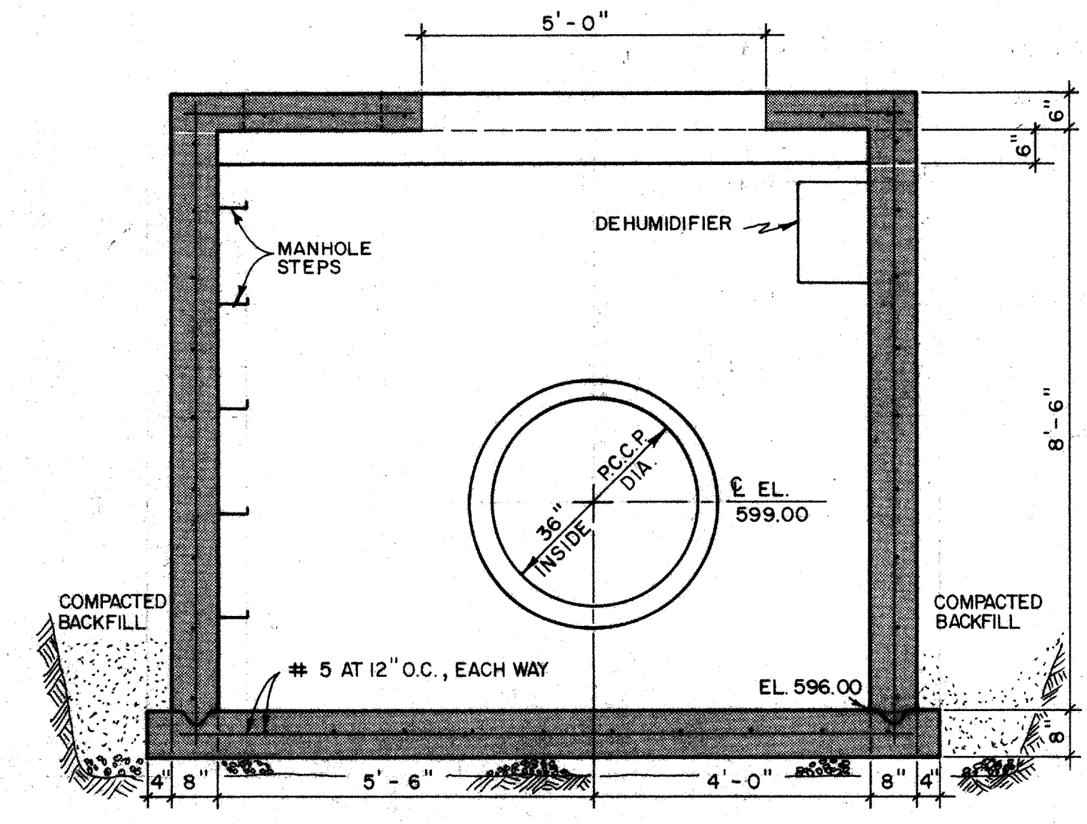
SECTION 2 SCALE - 1/2" = 1'-0"
