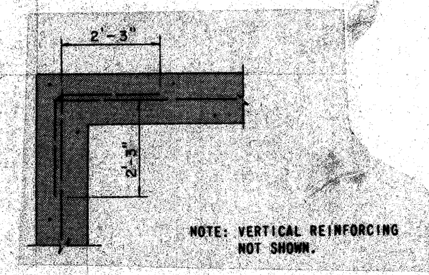
TYPICAL CORNER REINFORCING DETAILS (PLAN VIEW)
