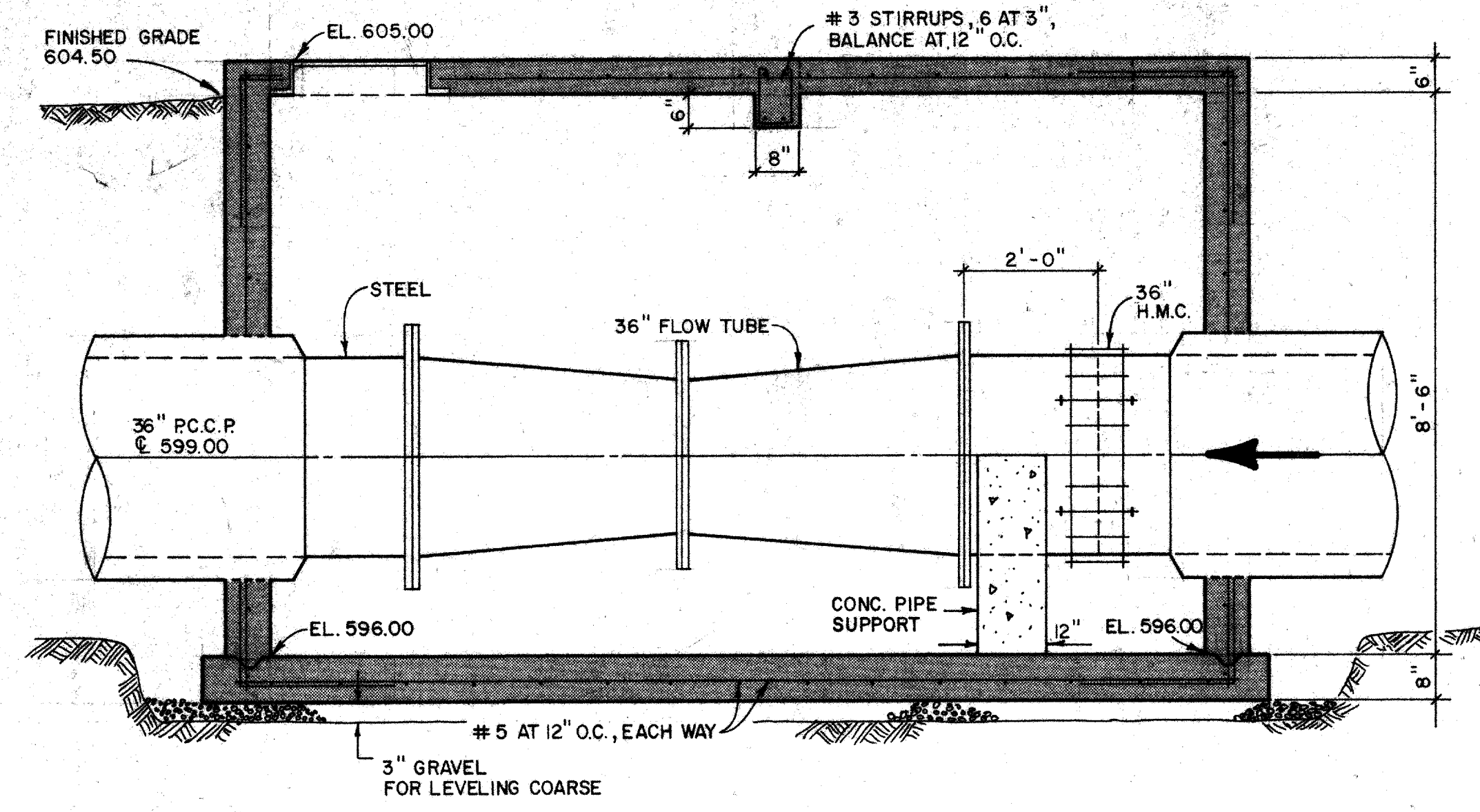
SECTION 1 SCALE - 1/2" = 1'-0"
