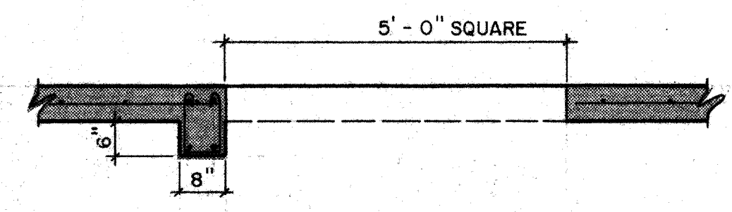
SECTION 3 SCALE - 1/2" = 1'-0"
