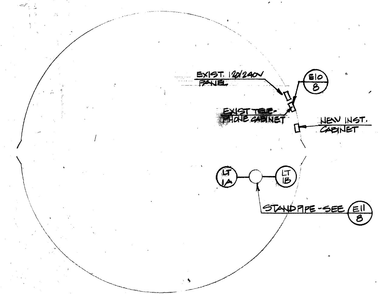
2 ELEVATED TANK PLAN NO SCALE
