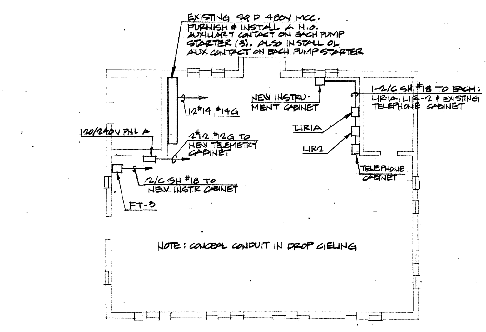
3 SURVEYOR PUMP STATION PLAN NO SCALE
