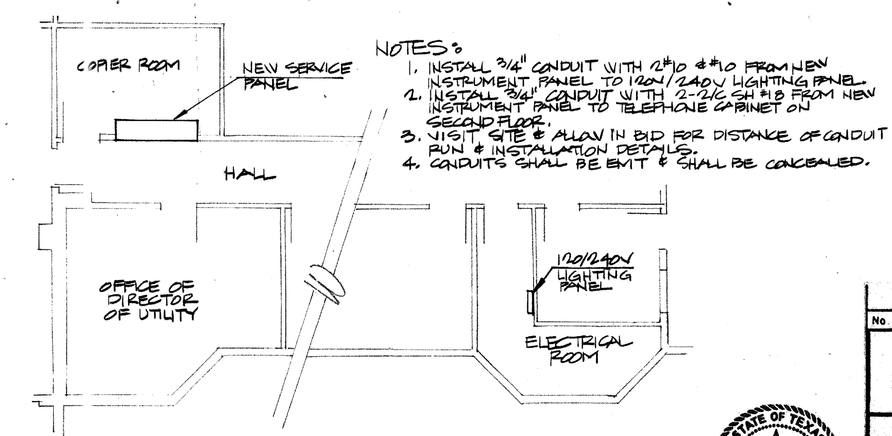
4 SERVICE CENTER PARTIAL PLAN SCALE 1/8" = 1'-0"
