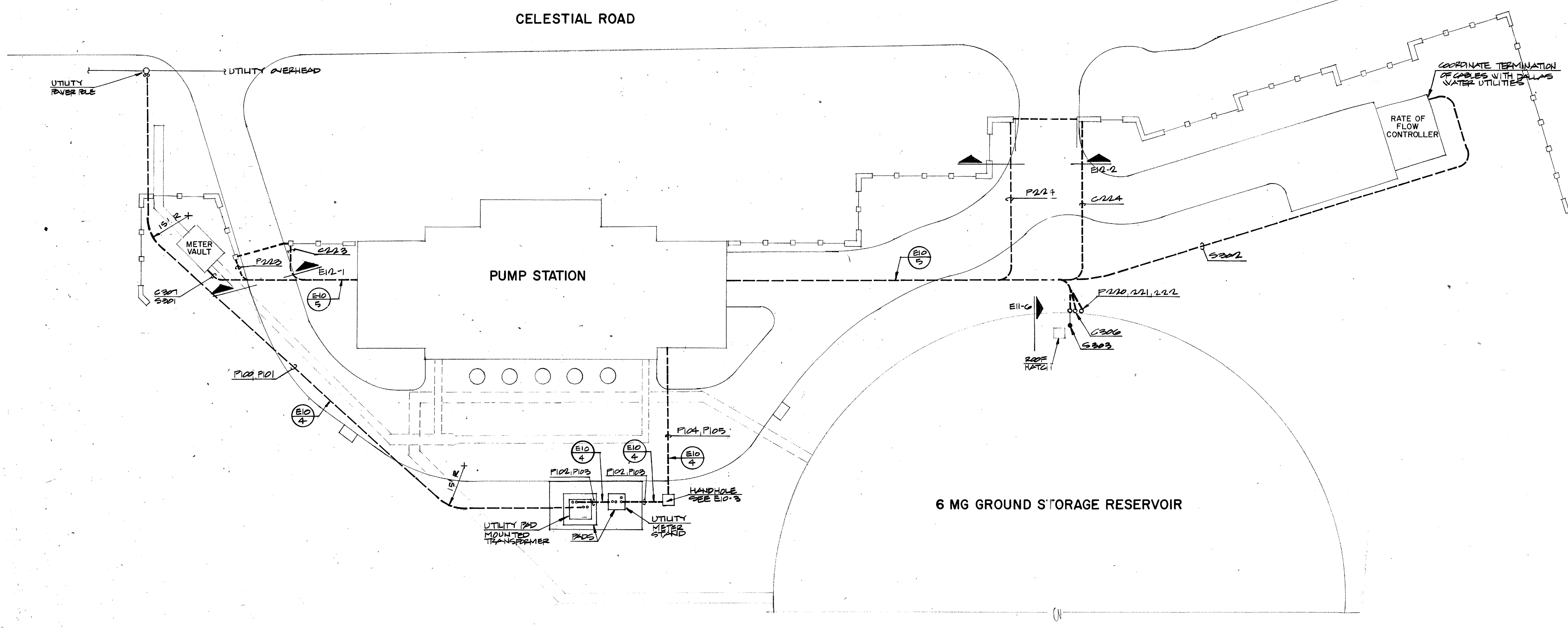
1 SITE PLAN SCALE 1" = 20'
