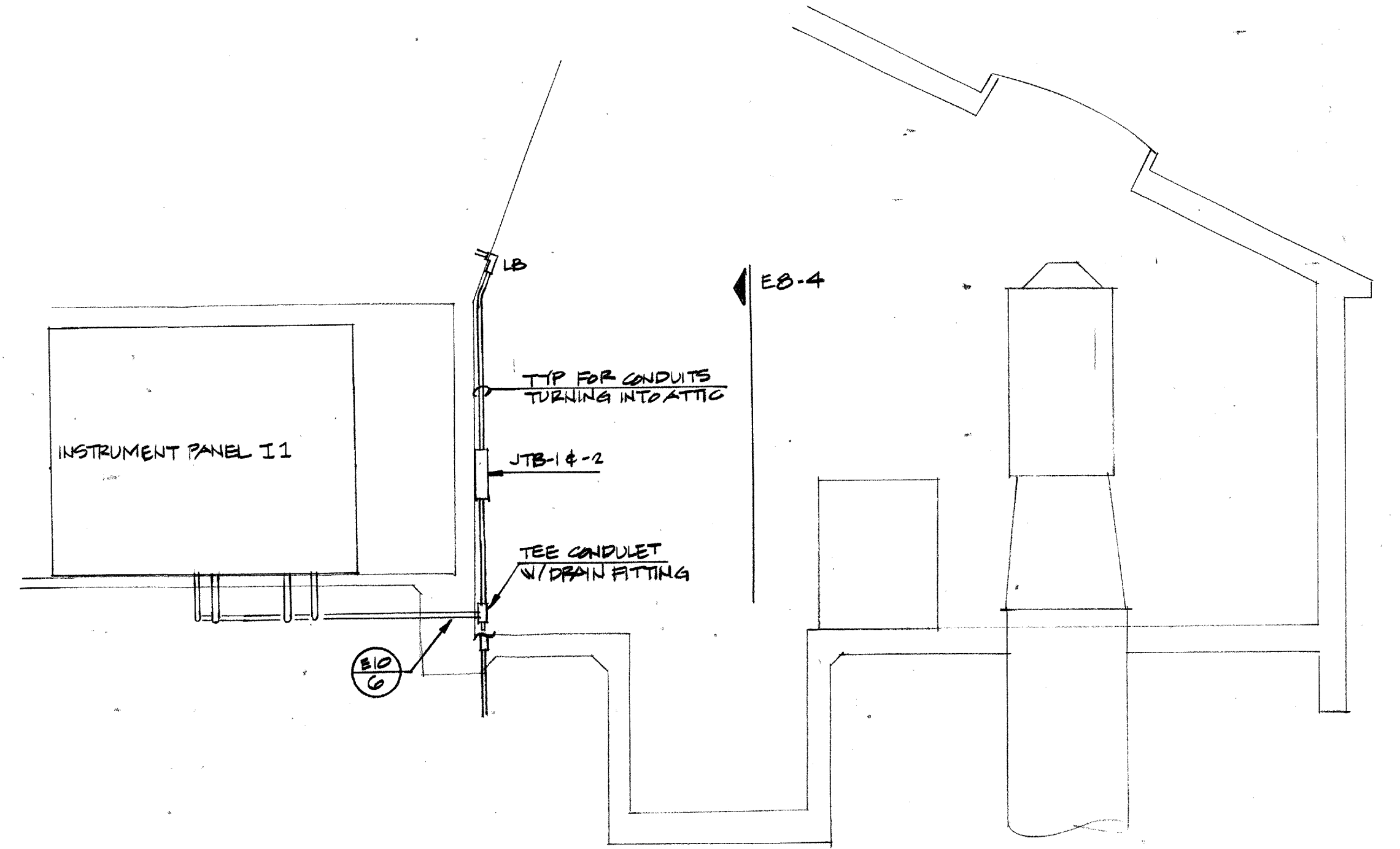
3 SECTION SCALE 1/4"=1'-0"
