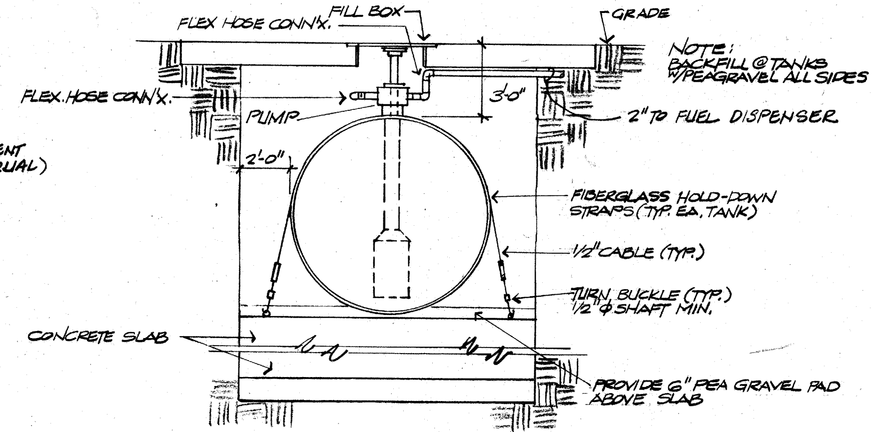
SECTION THRU UNDERGROUND TANK NOT TO SCALE
