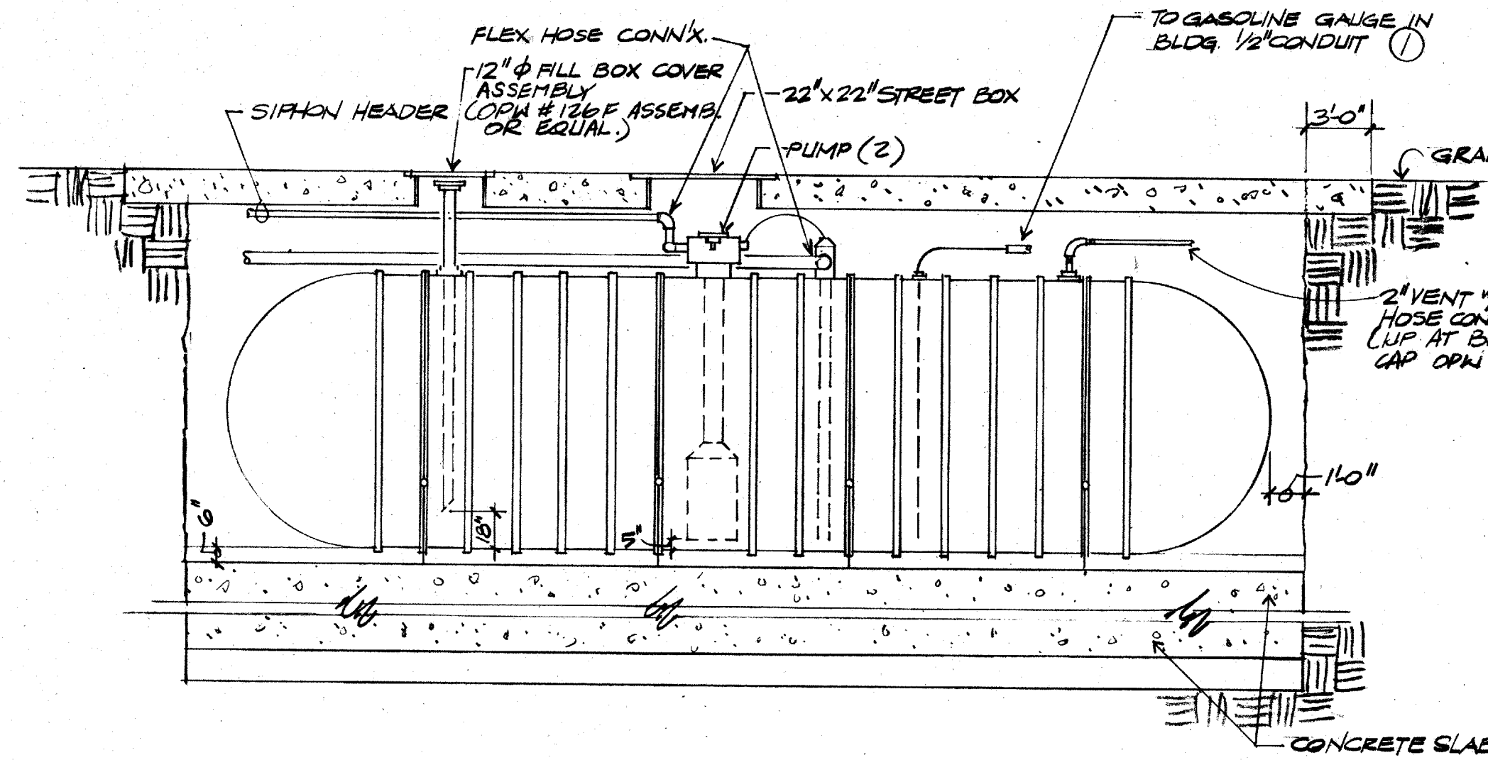
PIPING DIAGRAM THRU UNDERGROUND STORAGE TANK NOT TO SCALE
