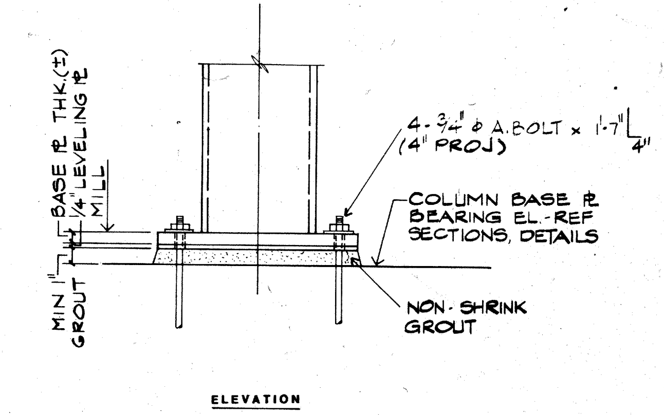
10 TYPICAL COLUMN BASE PLATE NO SCALE 05108A
