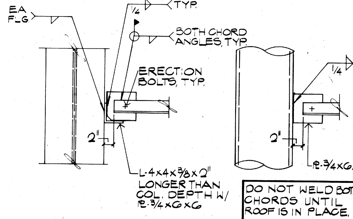
09 TYP. BOT. CHORD CONNECTION NO SCALE 05204
