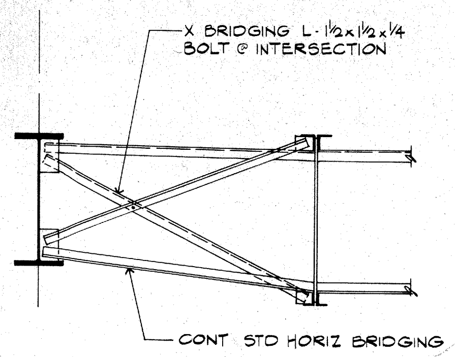
01 TYPICAL BRIDGING CONNECTION NO SCALE 05242
