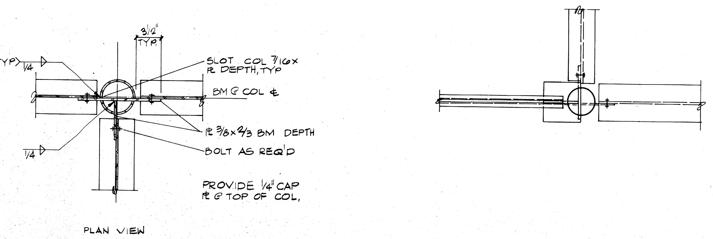
20 TYPICAL BEAM/COL CONNECTION NO SCALE
