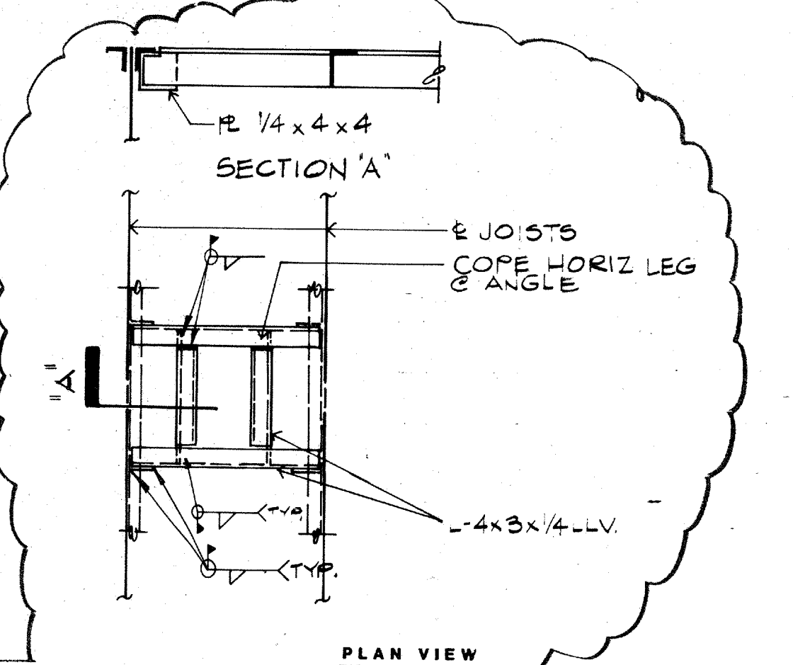
11 ROOF DRAIN FRAME DETAIL NO SCALE 05203
