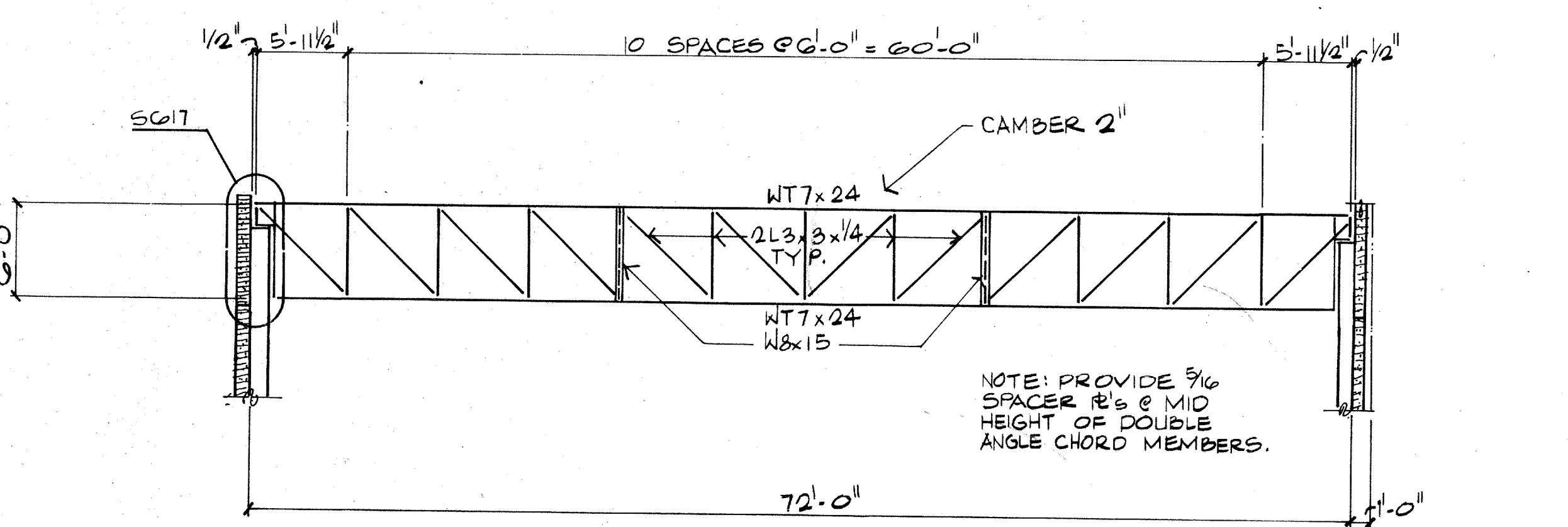
16 TRUSS ELEVATION 1/8\"/>
