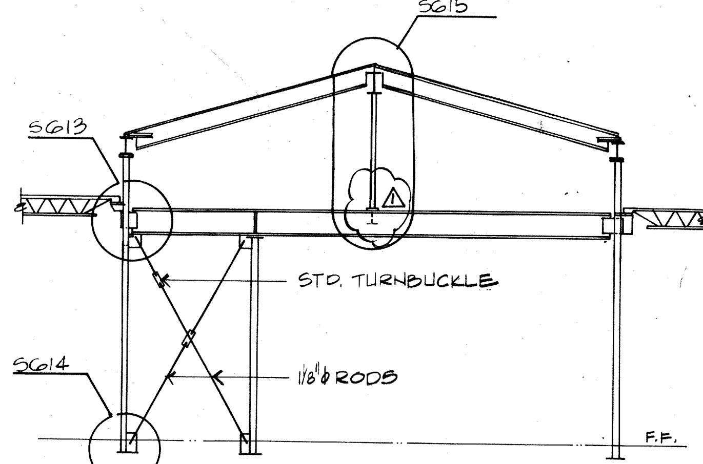
12 X-BRACE ELEVATION 1/4\"/>
