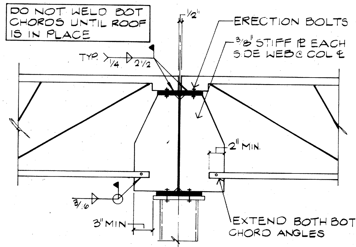
07 TYPICAL JOIST CONNECTION NO SCALE 05224
