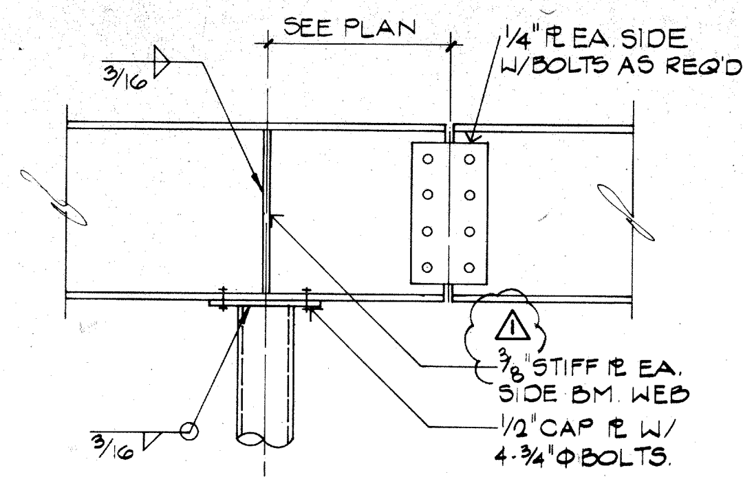
03 TYPICAL STEEL BEAM SPLICE NO SCALE 05109
