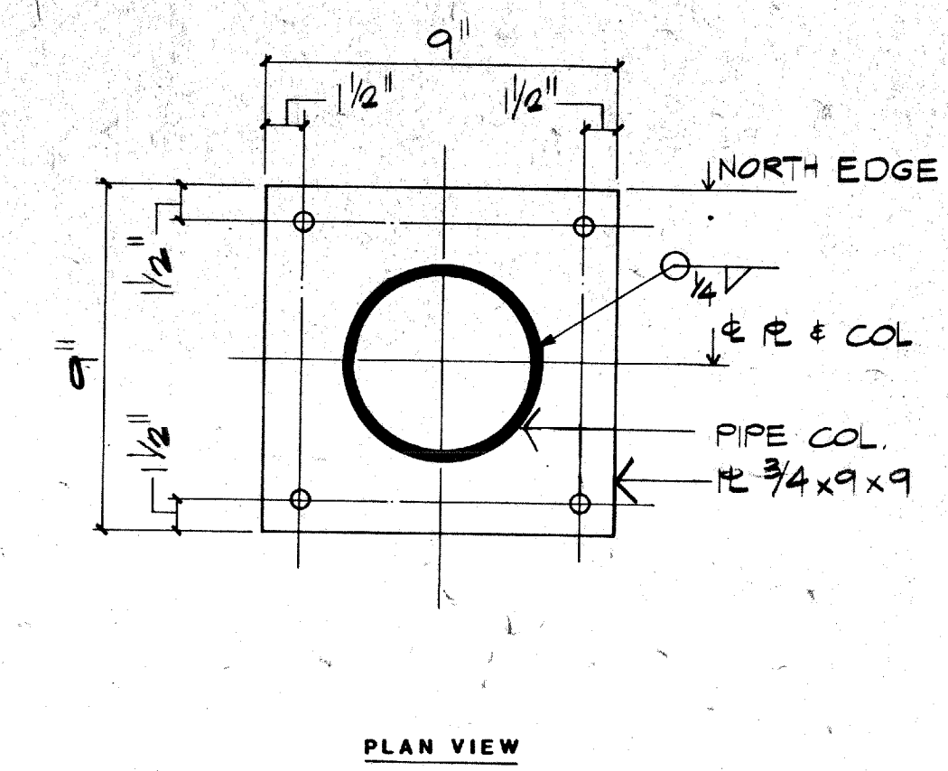
05 TYPICAL COLUMN BASE PLATE NO SCALE 05106
