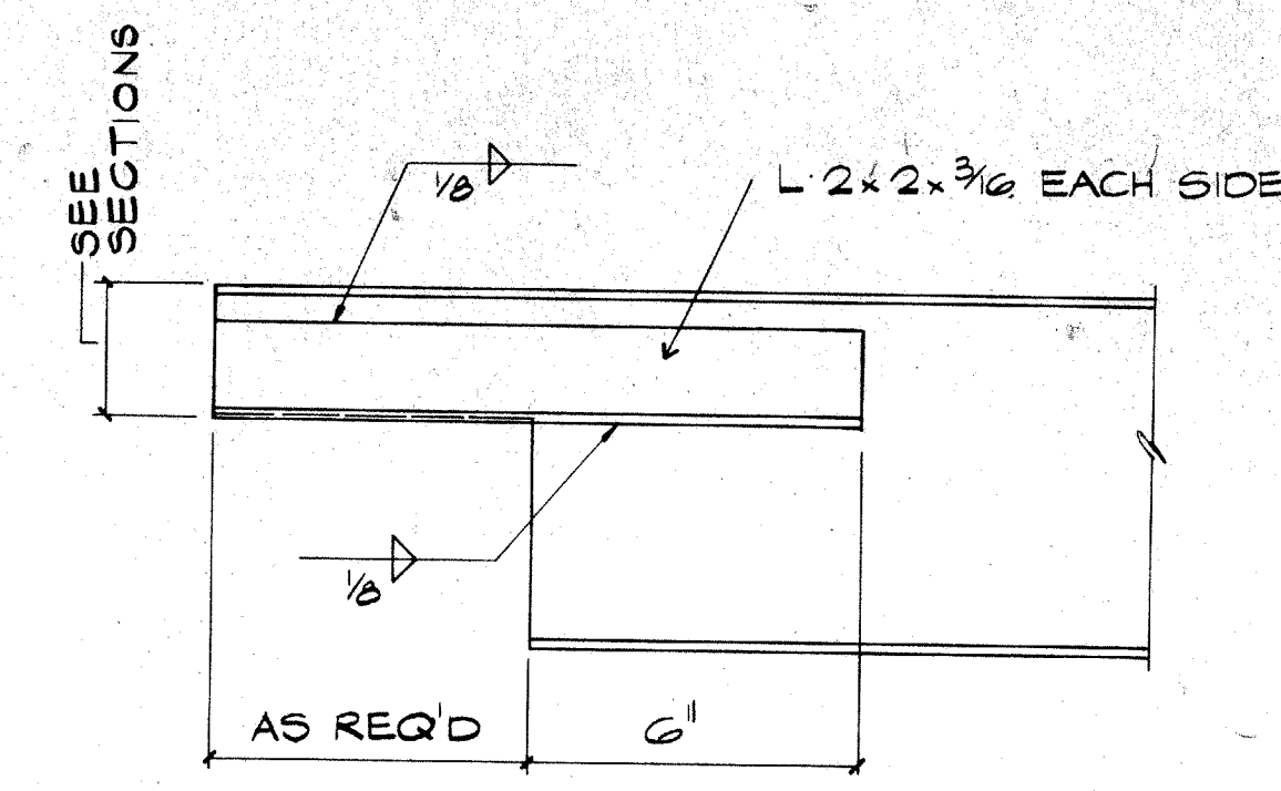
04 TYPICAL COPED CHANNEL OR BEAM NO SCALE 05108
