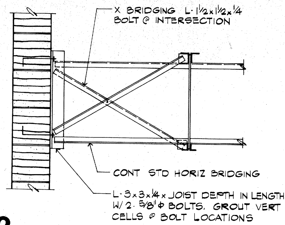
02 TYPICAL BRIDGING CONNECTION NO SCALE 05241
