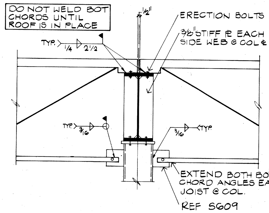
08 TYPICAL JOIST CONNECTION NO SCALE 05221
