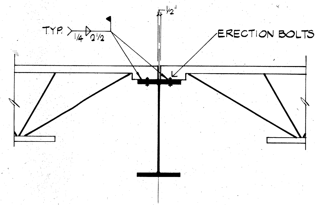
01 TYPICAL BRIDGING CONNECTION NO SCALE 05242
