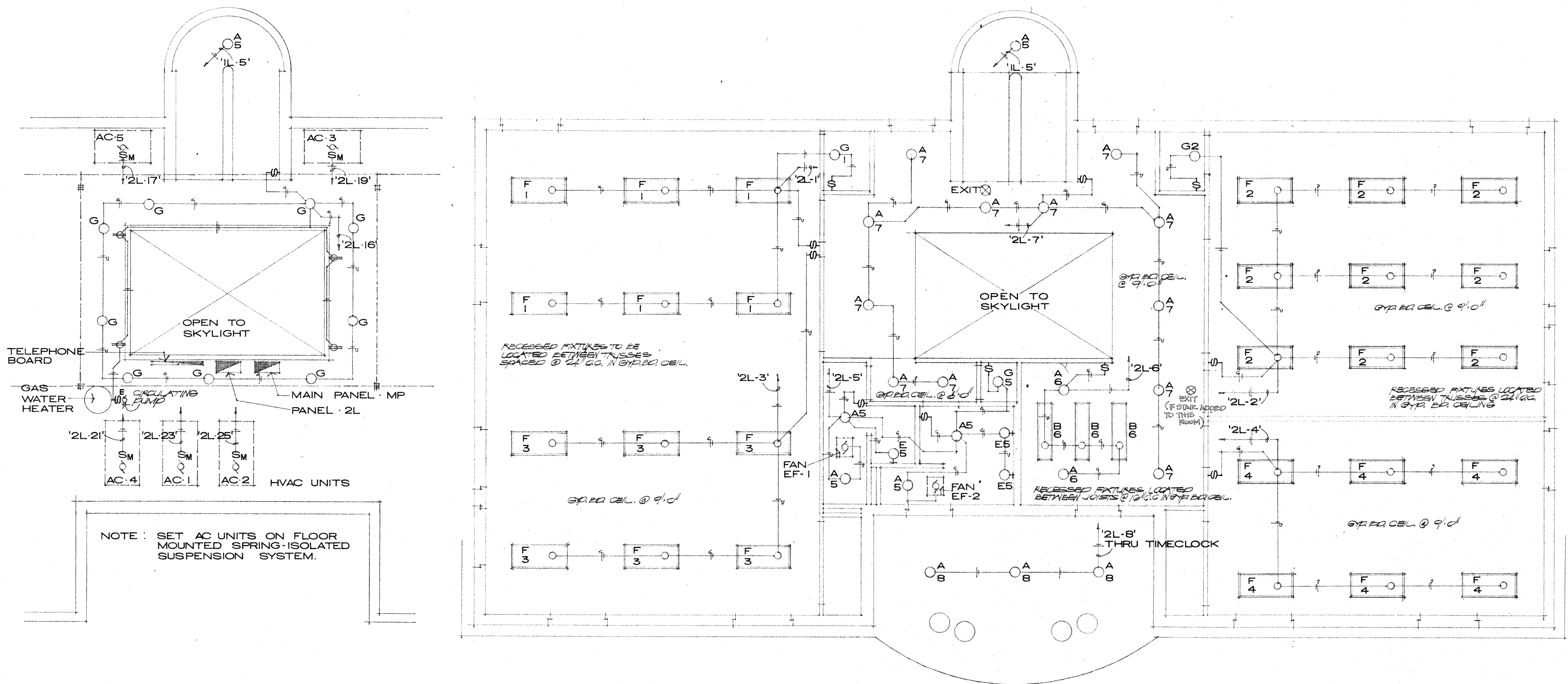
02 ATTIC LIGHTING/POWER FLOOR PLAN 1/4" = 1' - 0"
