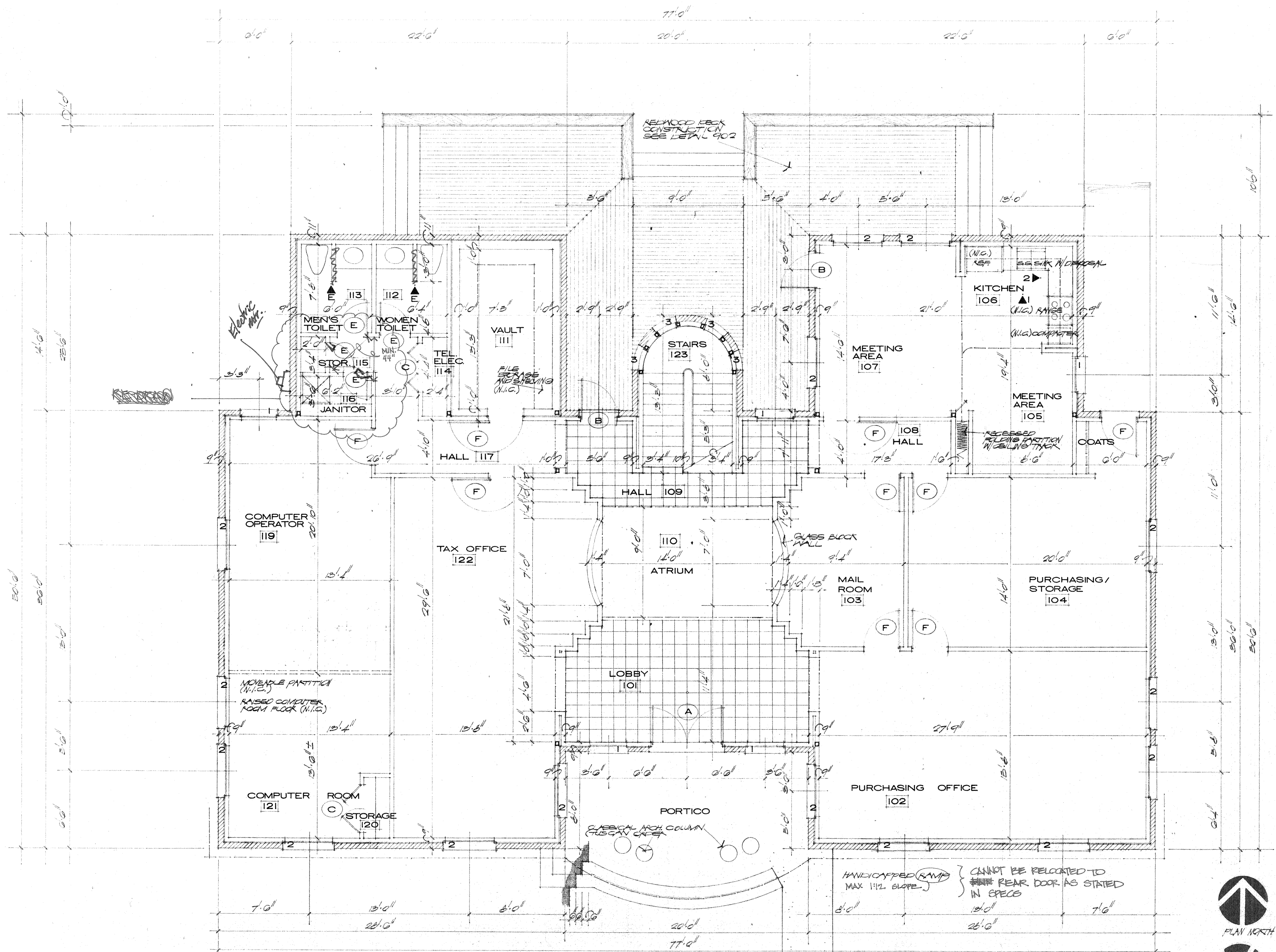
01 FIRST FLOOR PLAN SCALE 1/4" = 1' - 0"
