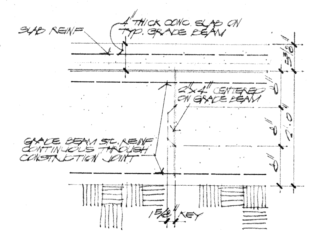
10 ELEVATION TYPICAL GRADE BEAM CONSTRUCTION JOINT DETAIL
