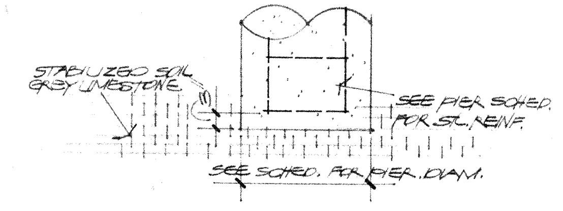
11 DETAIL TYPICAL EXTERIOR PIER CONST.
