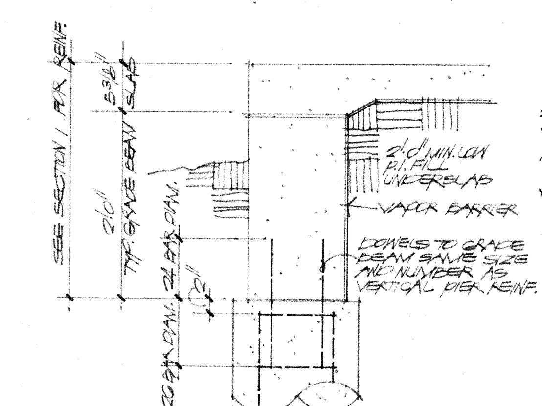
10 ELEVATION TYPICAL GRADE BEAM CONSTRUCTION JOINT DETAIL
