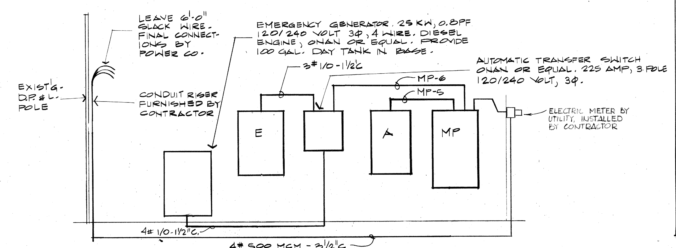
E103 ELECTRICAL RISER DIAGRAM NOT TO SCALE
