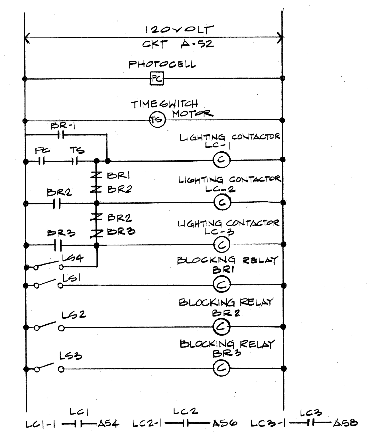
E104 EXTERIOR LIGHTING CONTROL DIAGRAM SCHEMATIC ONLY
