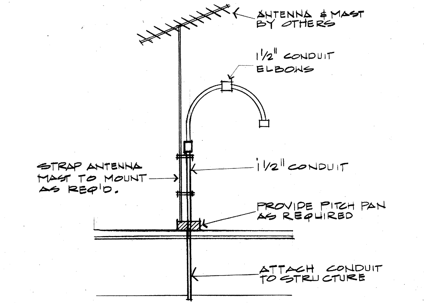
E102 ANTENNA MAST SUPPORT DETAIL NOT TO SCALE NOTES 1. INSTALL ON ROOF AT LOCATION SELECTED BY ARCHITECT
