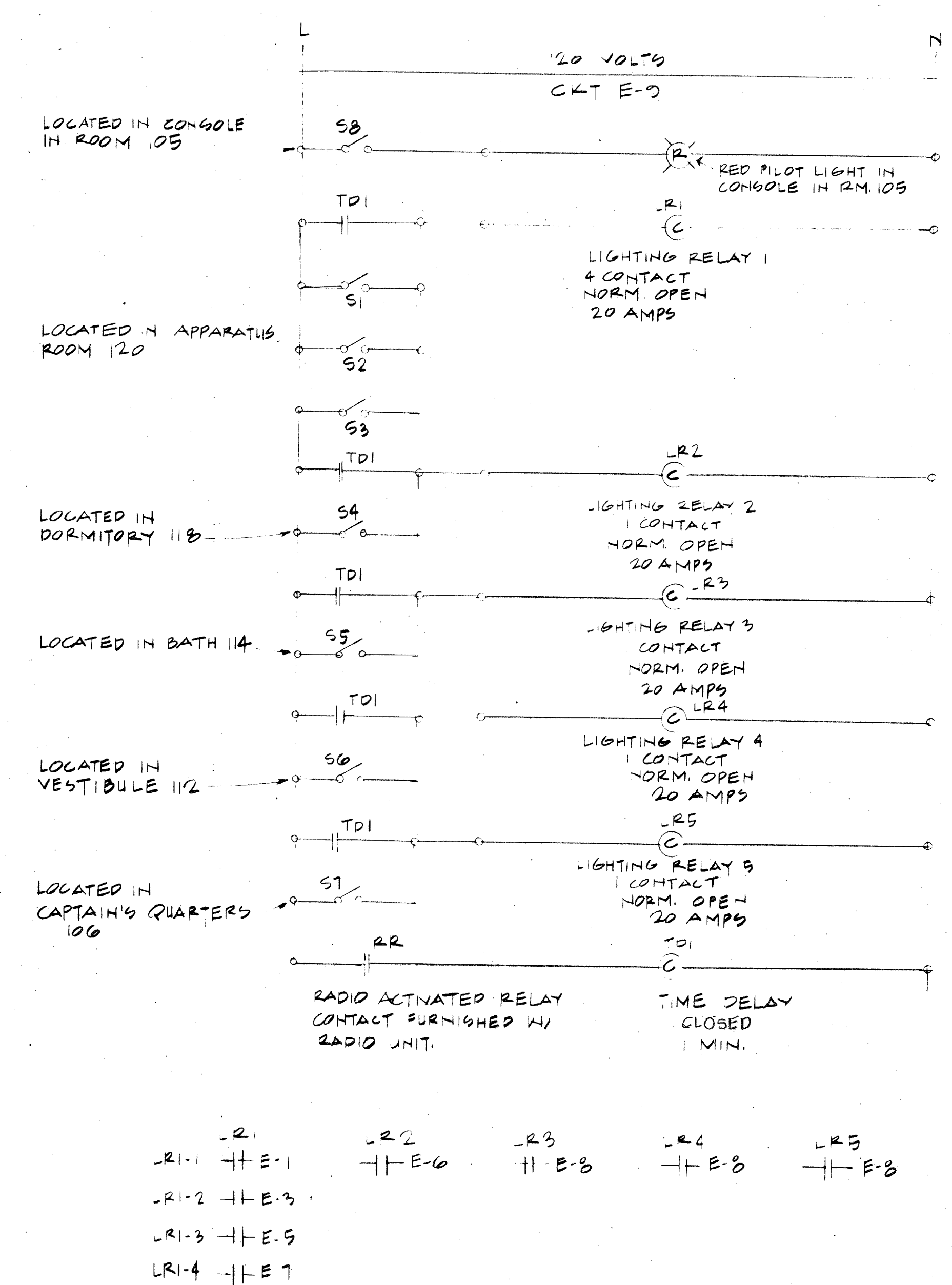
INTERIOR LIGHTING CONTROL DIAGRAM NO SCALE
