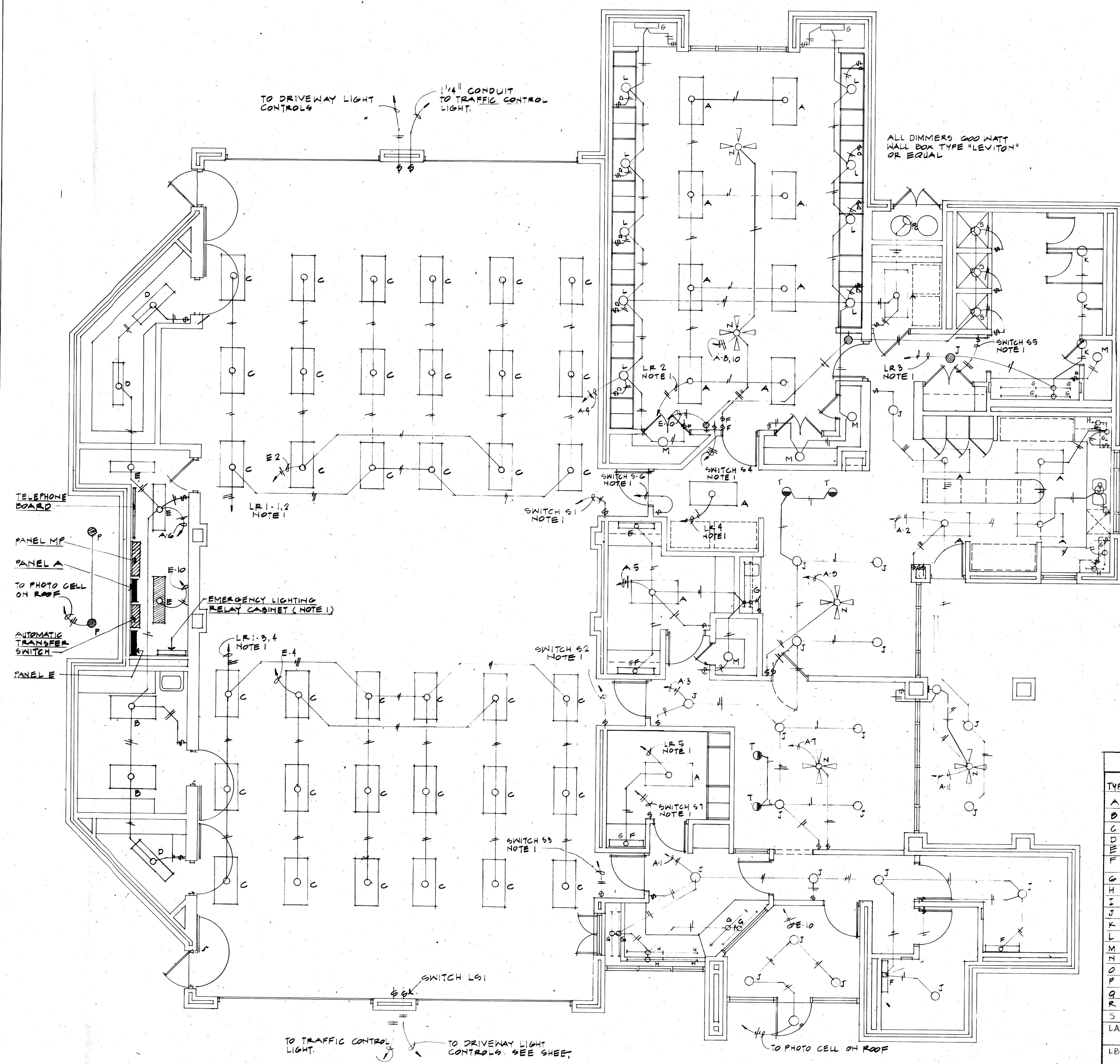
E301 LIGHTING PLAN SC-1/4"=1'-0"
