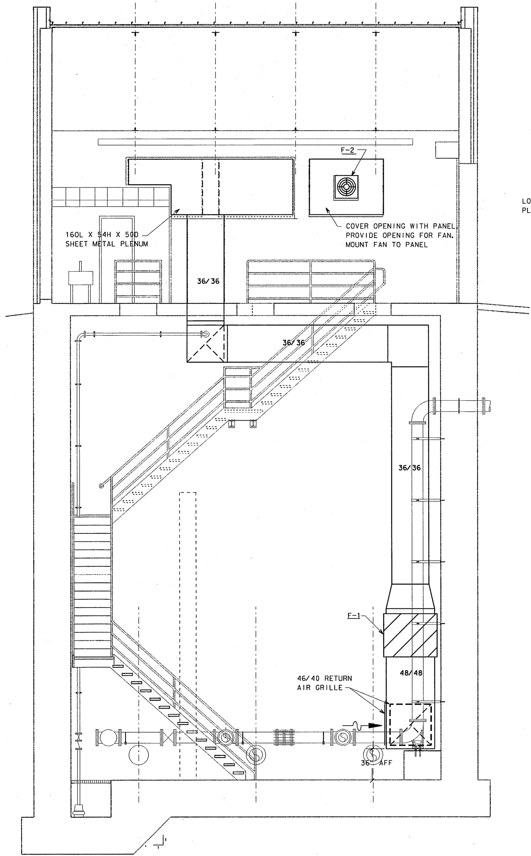
SECTION A 1/4" = 1'-0"
