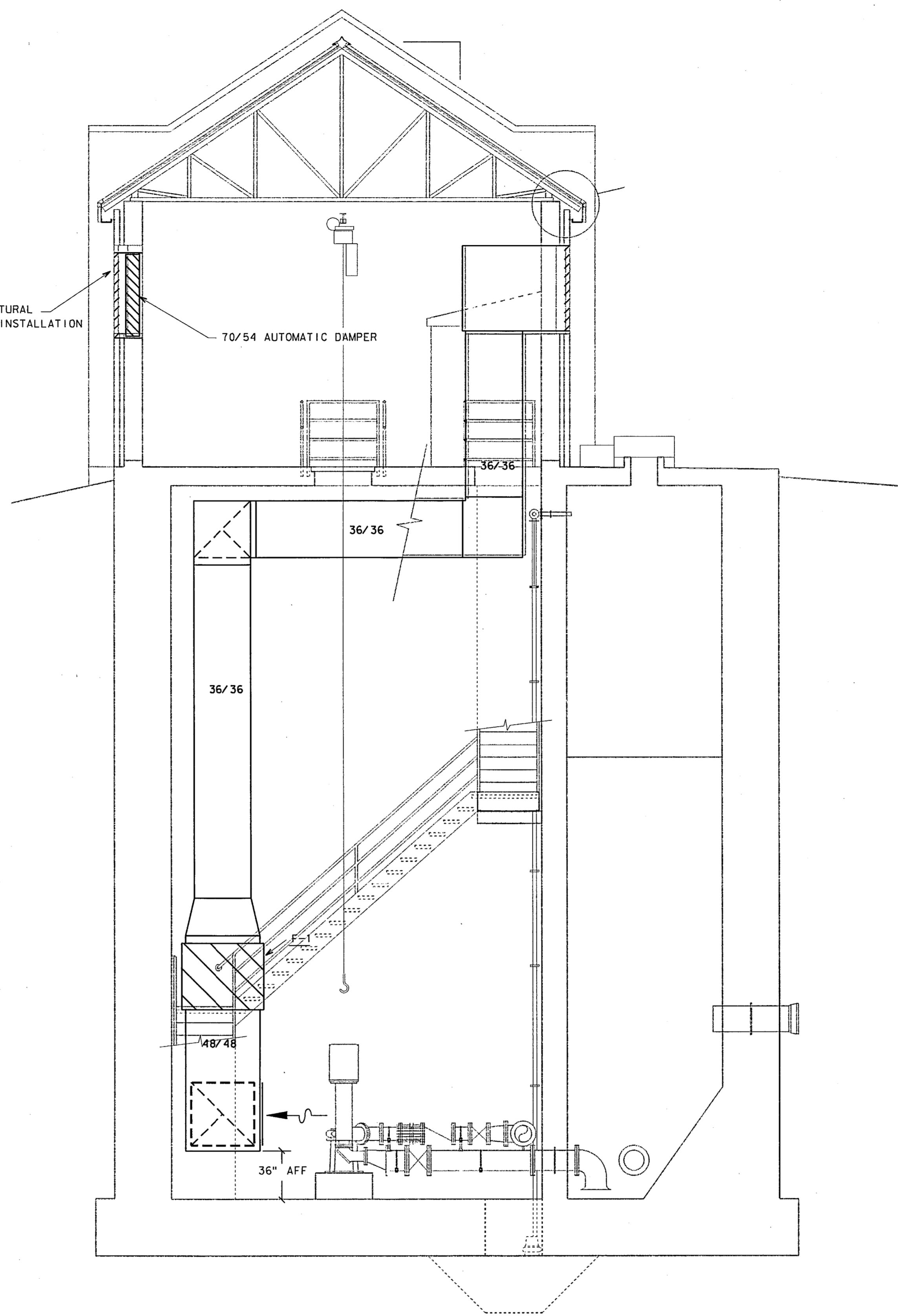
SECTION B 1/4" = 1'-0"
