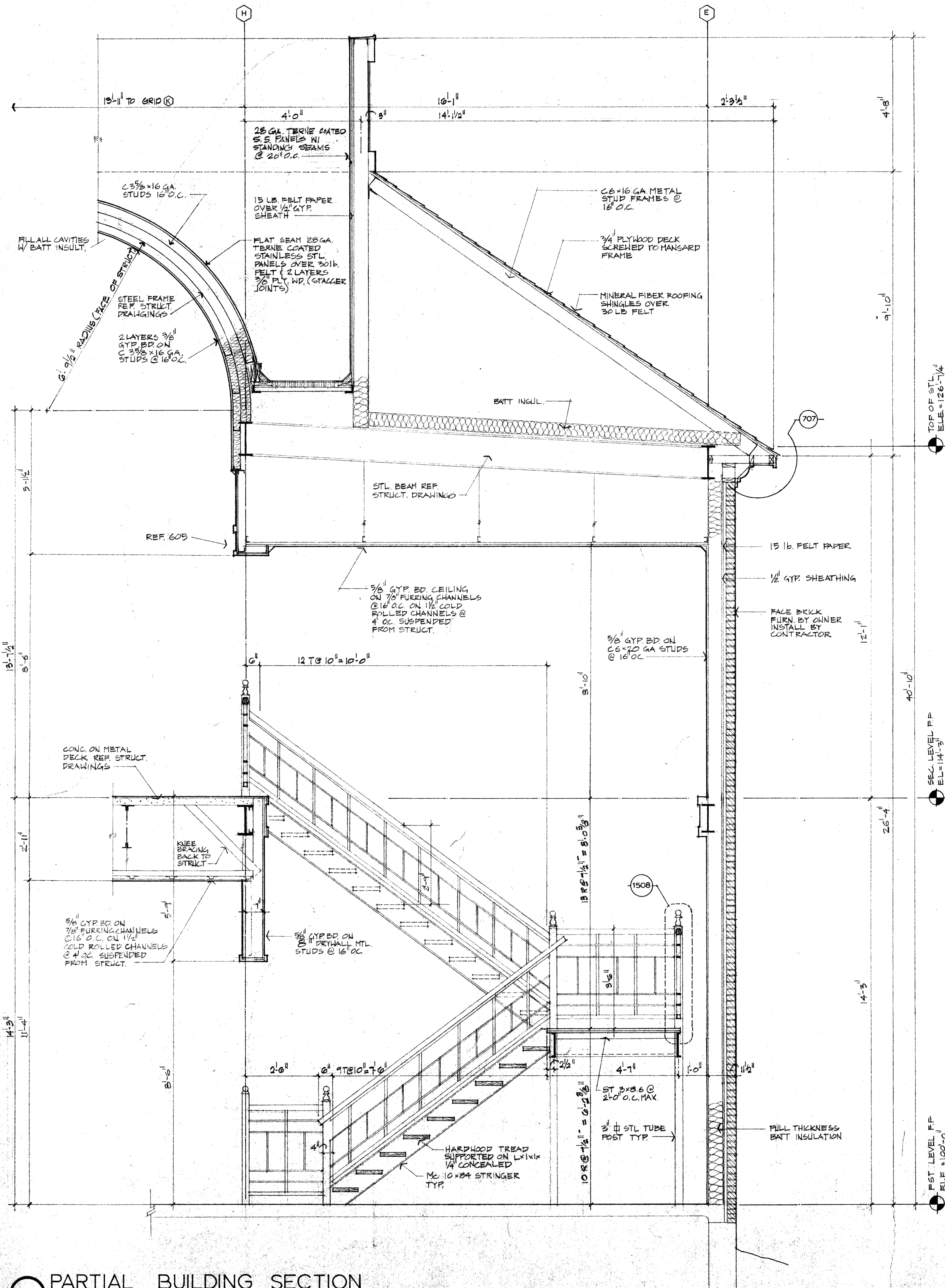
1107 PARTIAL BUILDING SECTION SCALE: 1/2"=1'-0" REF. 1001, 1002
