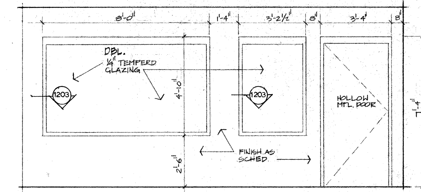
1105 FIRING RANGE 181 SCALE: 3/8"=1'-0" REF. 201
