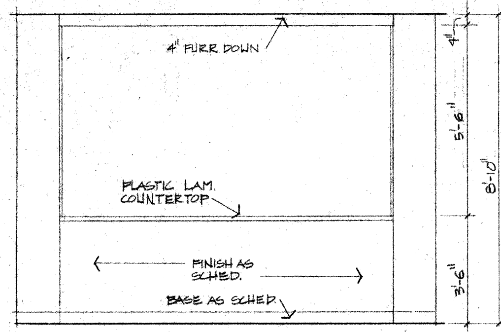
1103 RECORDS 112 SCALE: 3/8"=1'-0" REF. 201
