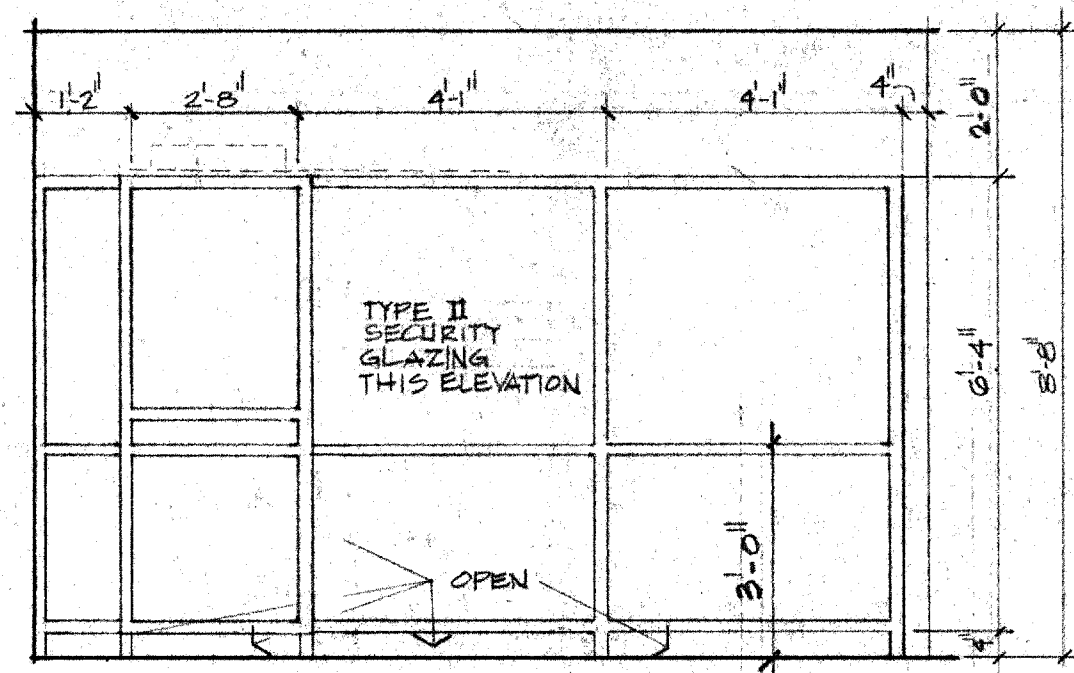
1101 LOBBY 150 SCALE: 3/8"=1'-0" REF. 201
