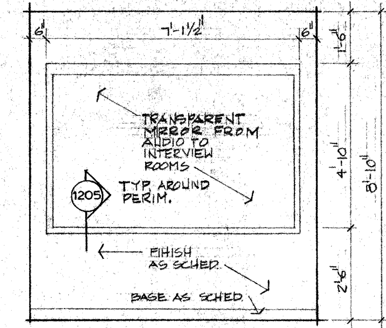
1106 AUDIO 161 SCALE: 3/8"=1'-0" REF. 201
