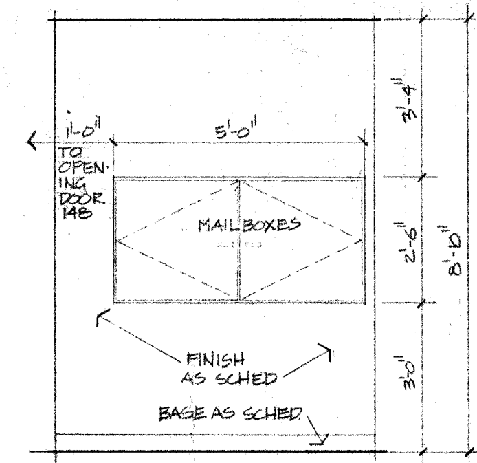
1104 RECORDS 112 SCALE: 3/8"=1'-0" REF. 201
