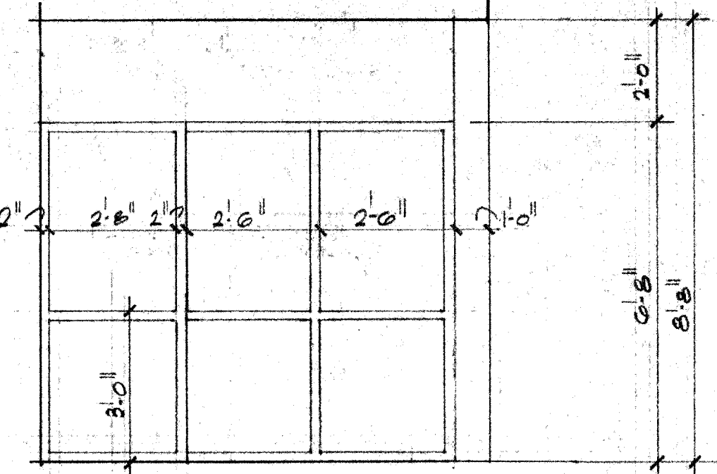
1102 ALCOVE 152 SCALE: 3/8"=1'-0" REF. 201
