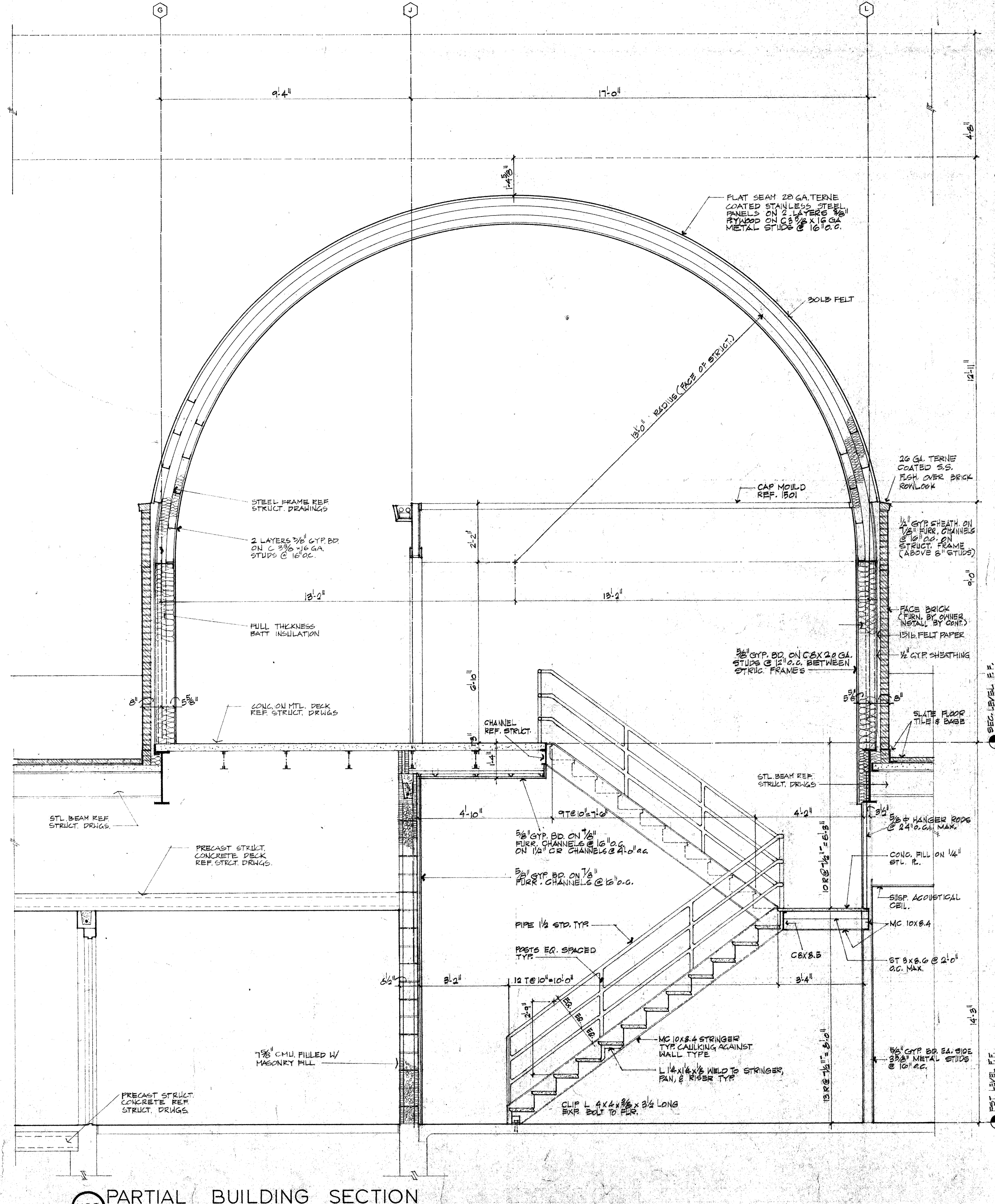
1108 PARTIAL BUILDING SECTION SCALE: 1/2"=1'-0" REF. 901, 902
