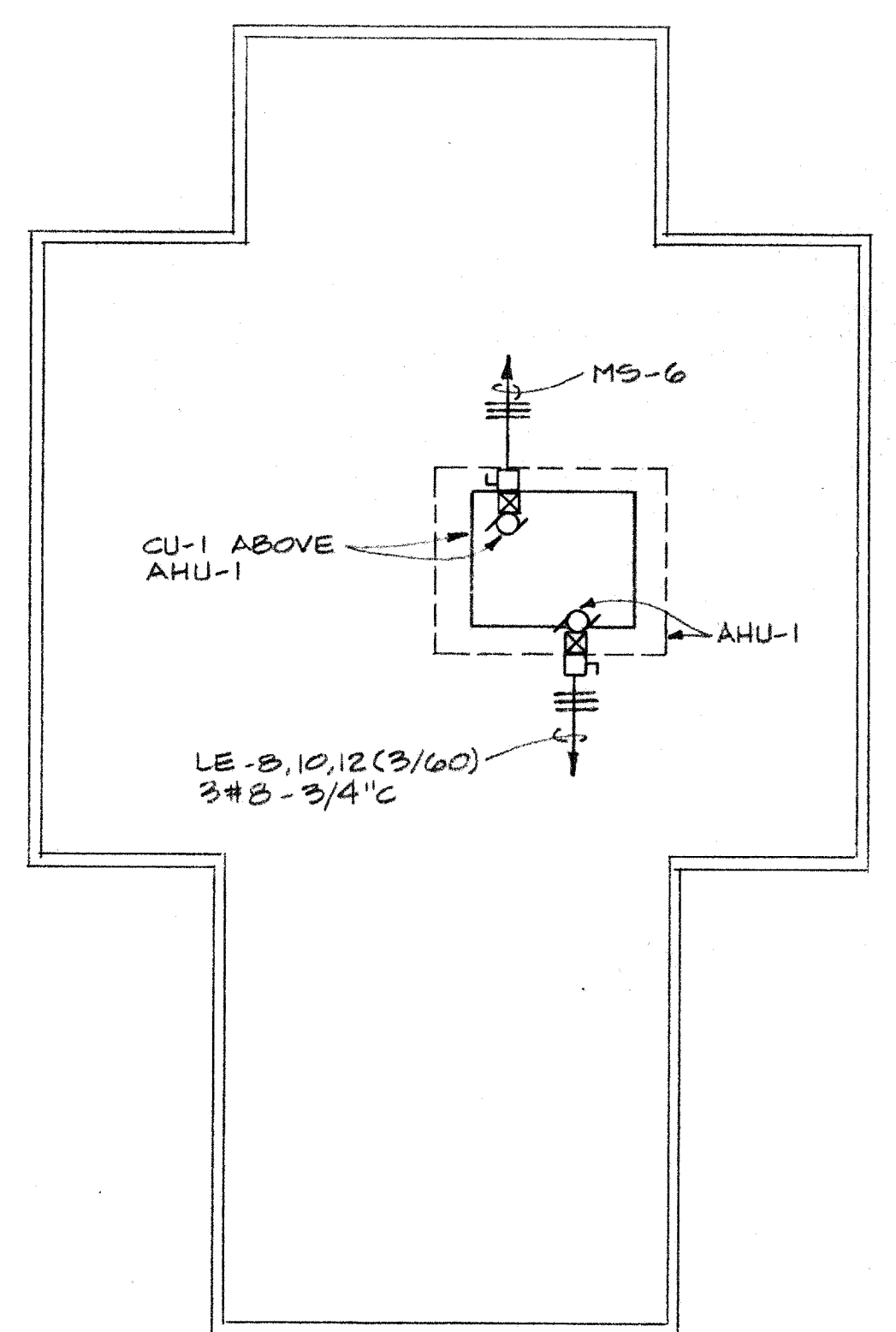
SECOND LEVEL ROOF PLAN SCALE 1/8" = 1'-0"
