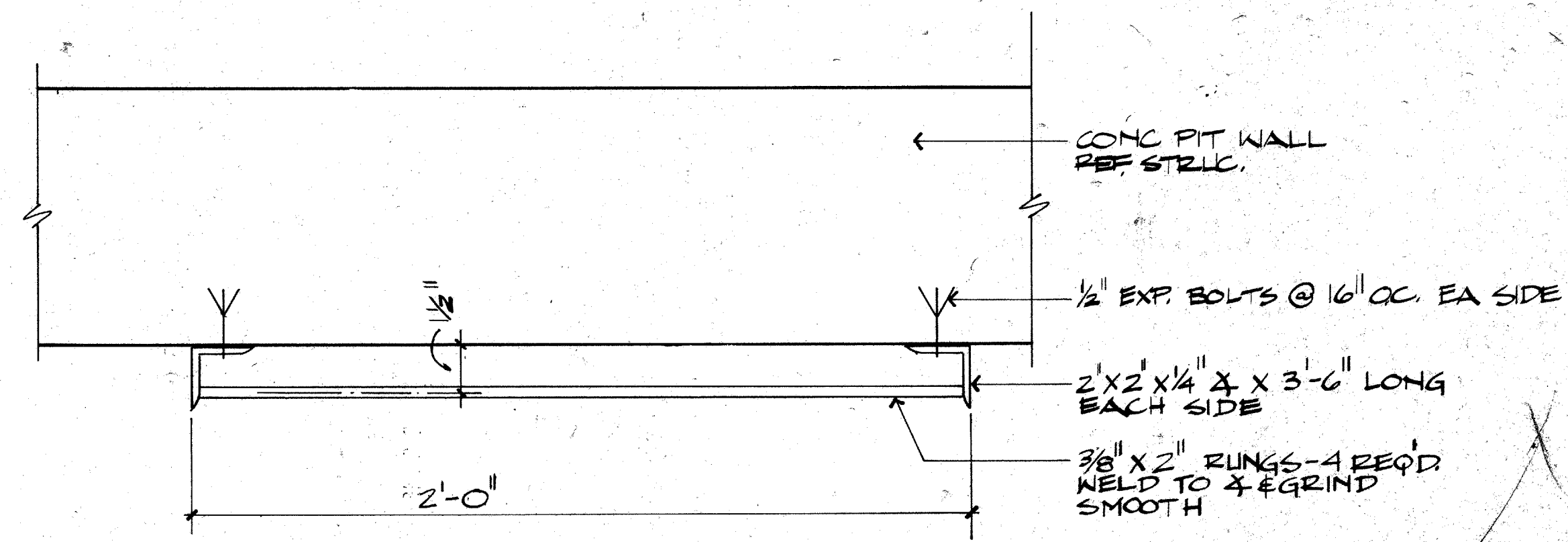
02 PLAN DETAIL @ PIT LADDER A6.1 3" = 1'-0"
