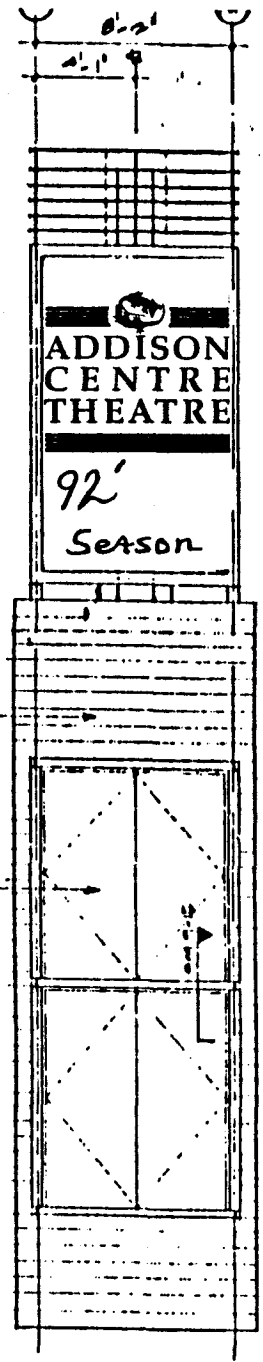
⑧ STAIR ELEVATION 4'-0" x 10'-0"
