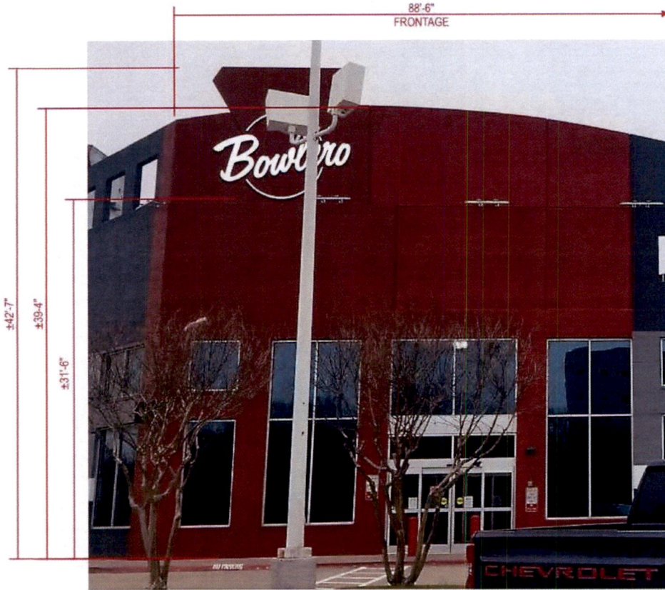
PROPOSED SIGN SOUTHEAST ELEVATION SCALE: 1/8"=1'-0"
