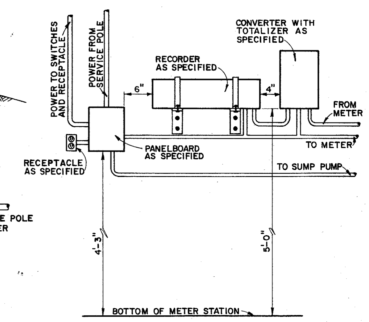
EQUIPMENT LAYOUT NO SCALE
