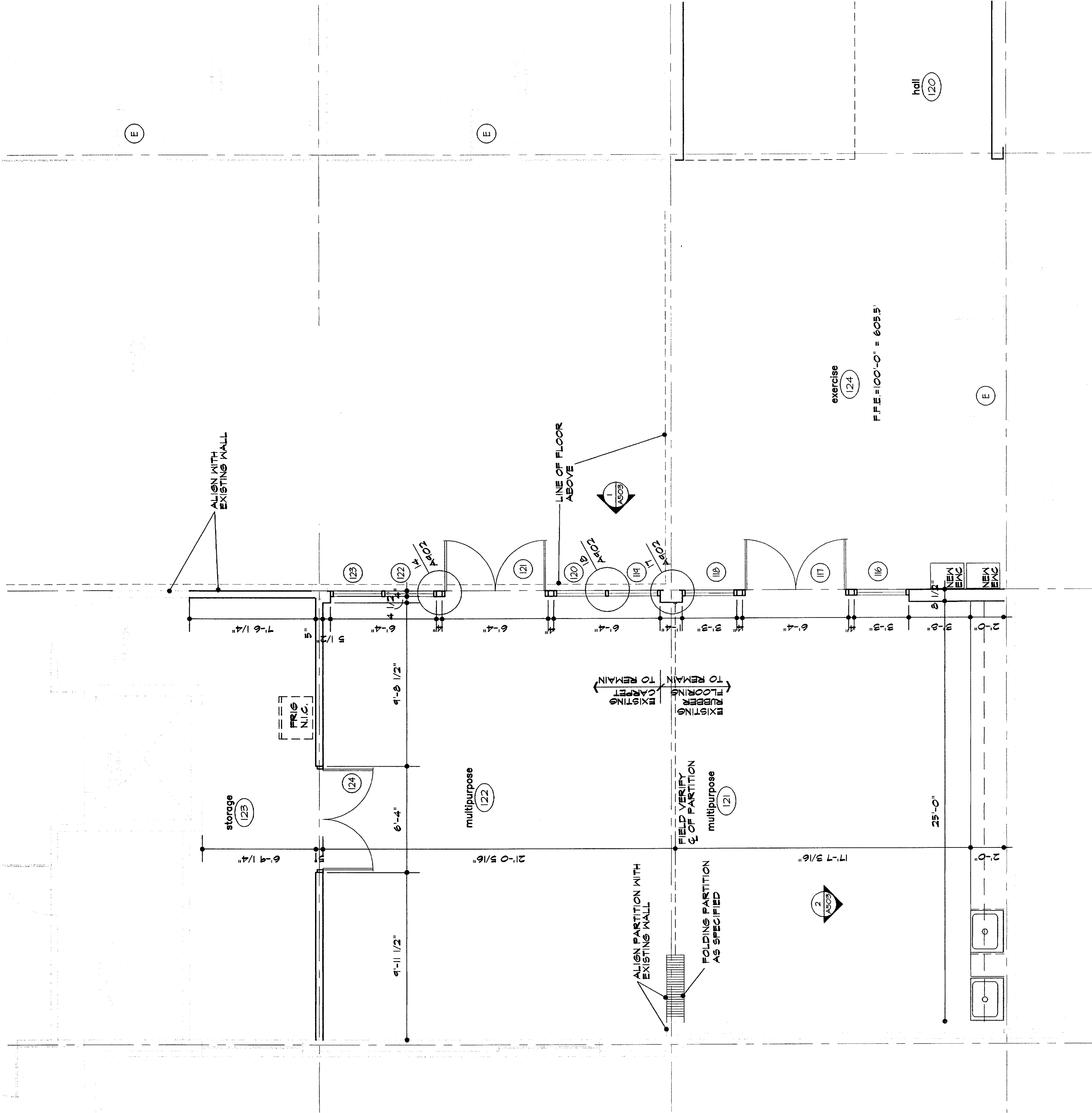
2 detail floor plan 1/4"=1'-0"
