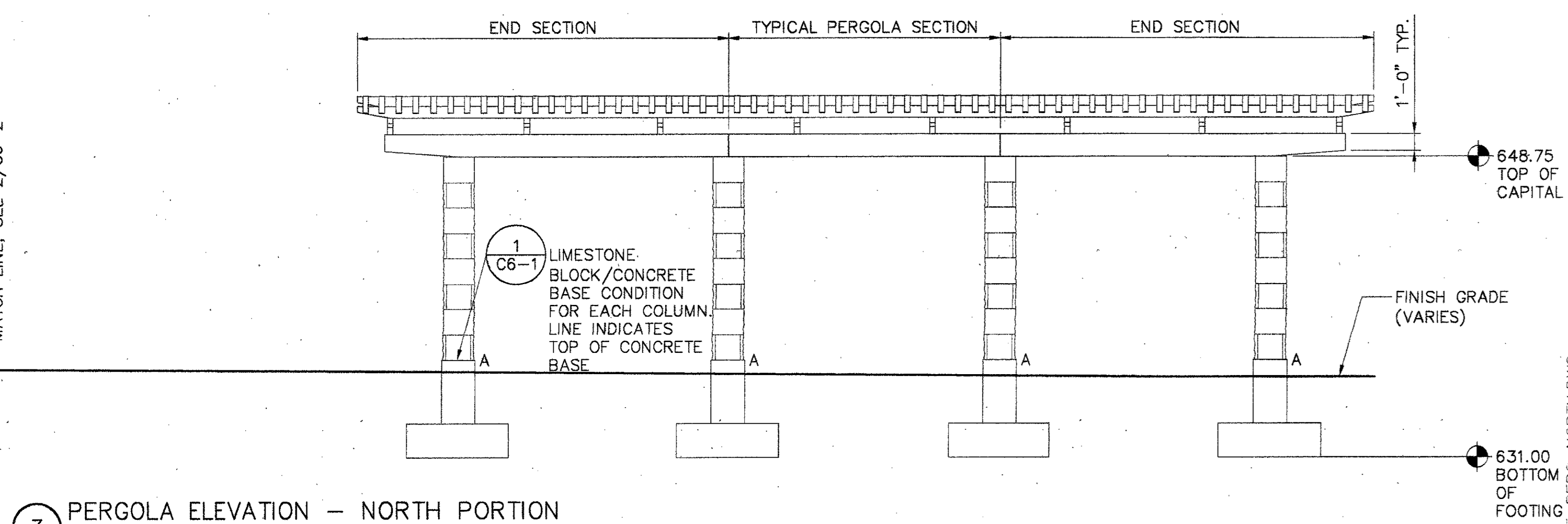
3 PERGOLA ELEVATION - NORTH PORTION
