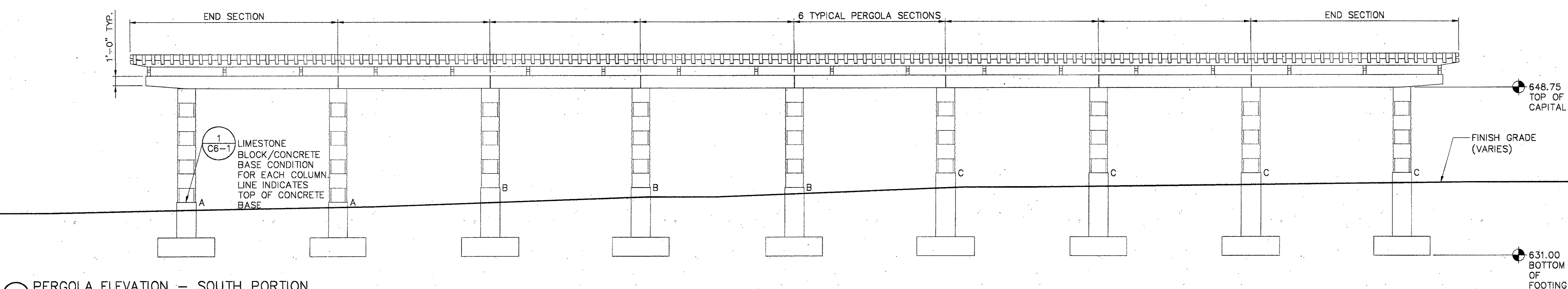
1 PERGOLA ELEVATION - SOUTH PORTION
