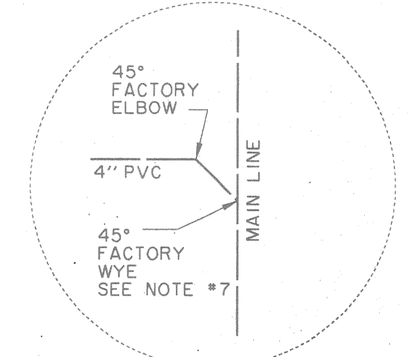
TYPICAL DRAIN CONNECTION
