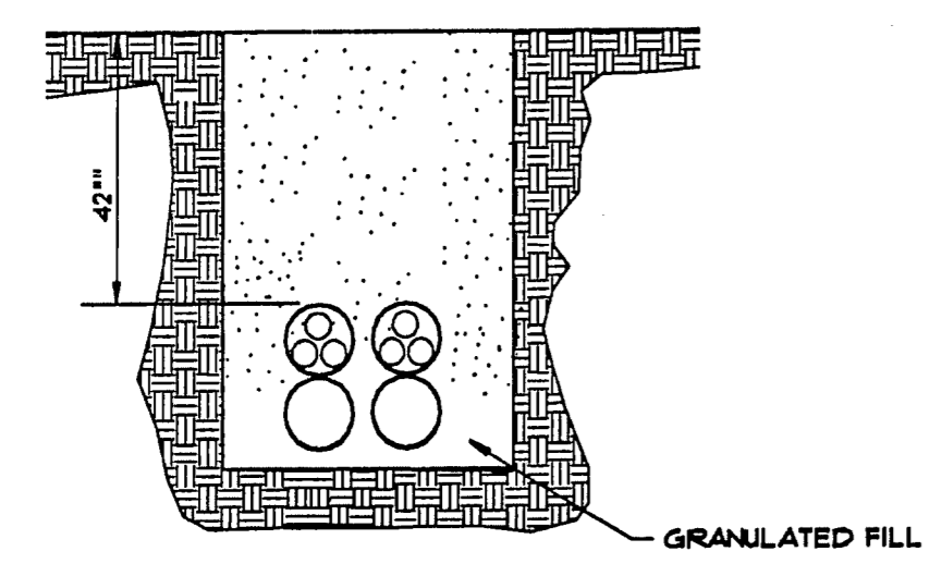
TYPICAL CONDUIT NOT TO SCALE
