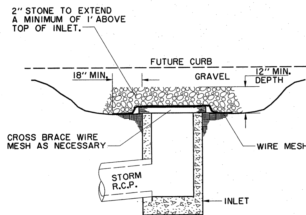
CROSS-SECTION
