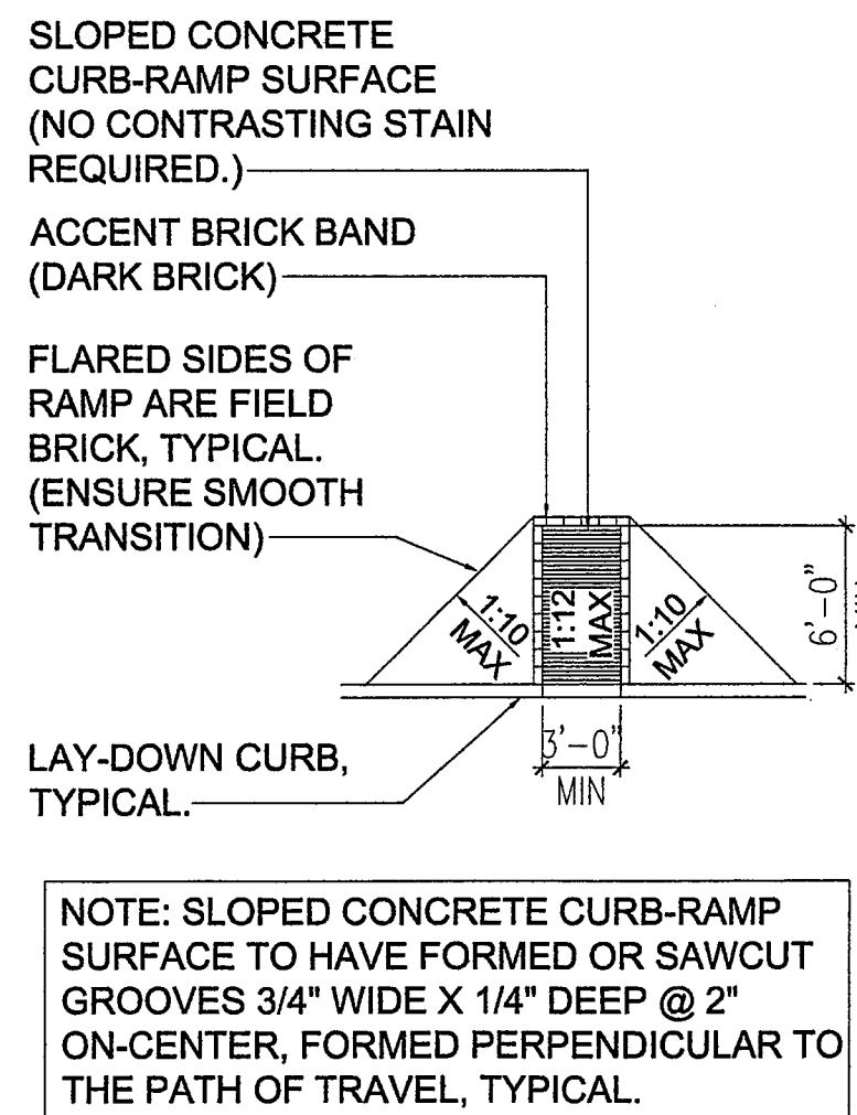
03 TYPICAL CURB RAMP DETAILS SCALE: 1/8"=1'-0"
