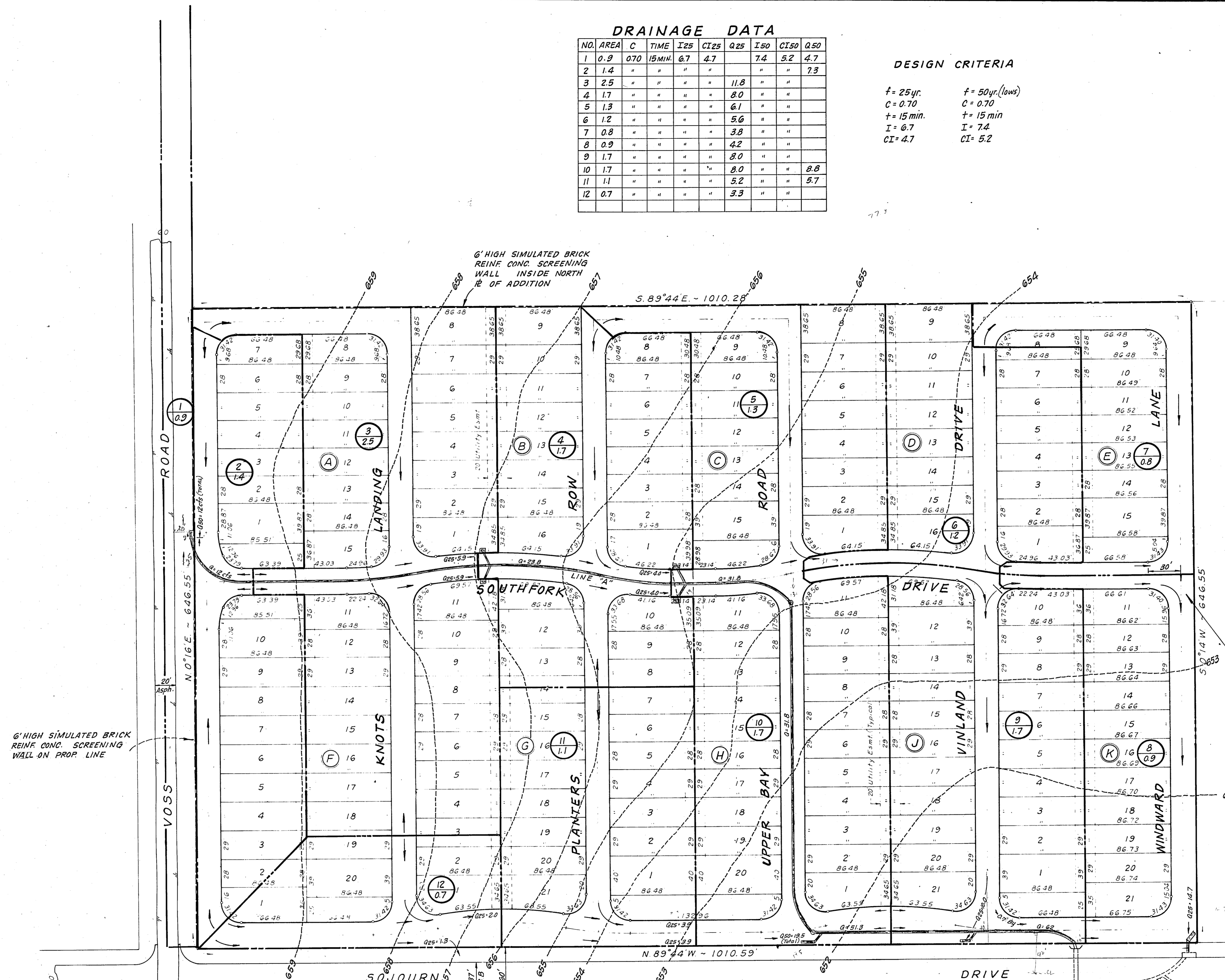
AREA DRAINAGE MAP
