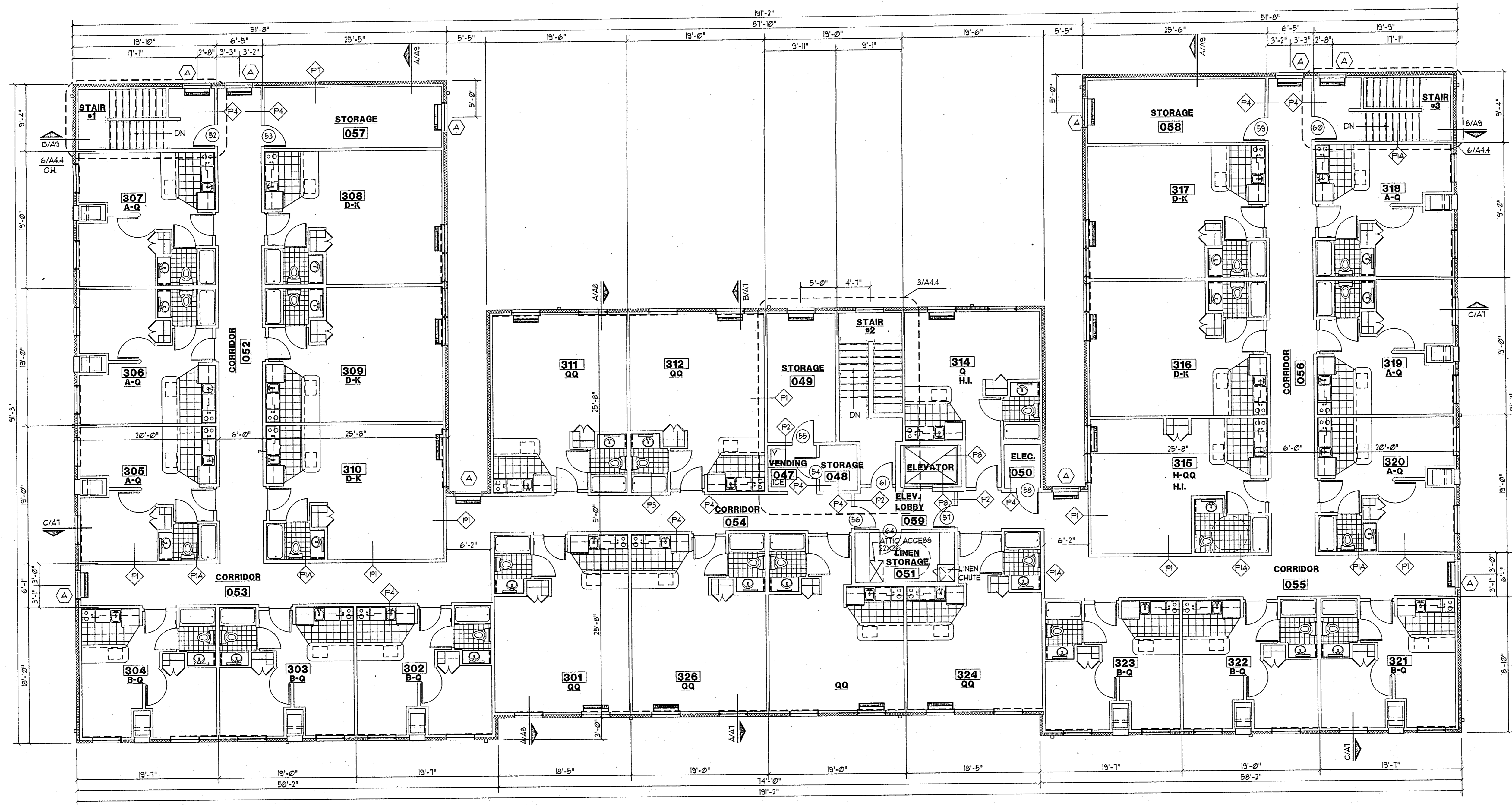
1 THIRD FLOOR PLAN SCALE: 1/8" = 1'-0"
