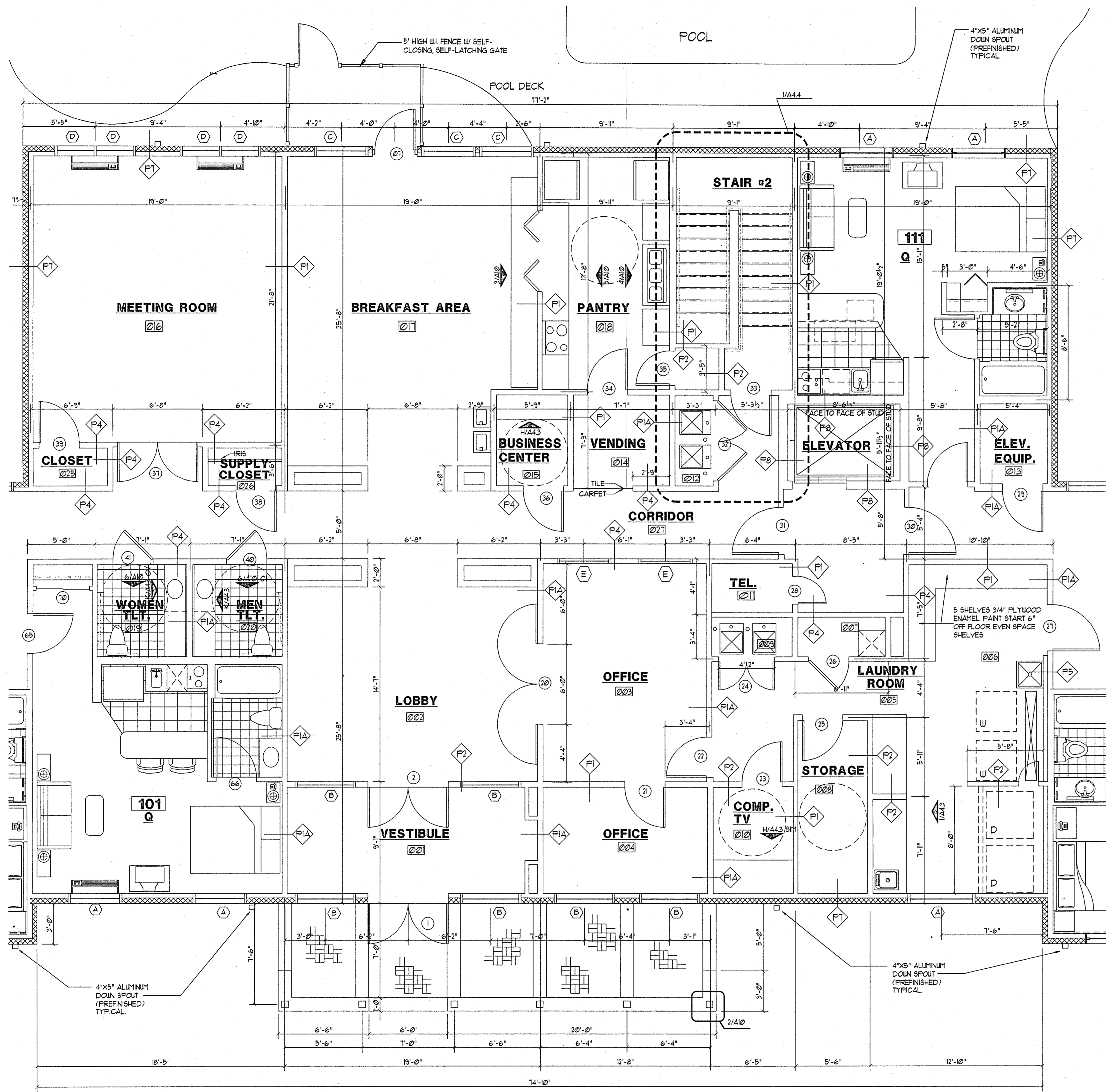
A LOBBY / COMMON AREA PLAN SCALE: 1/4" = 1'-0"
