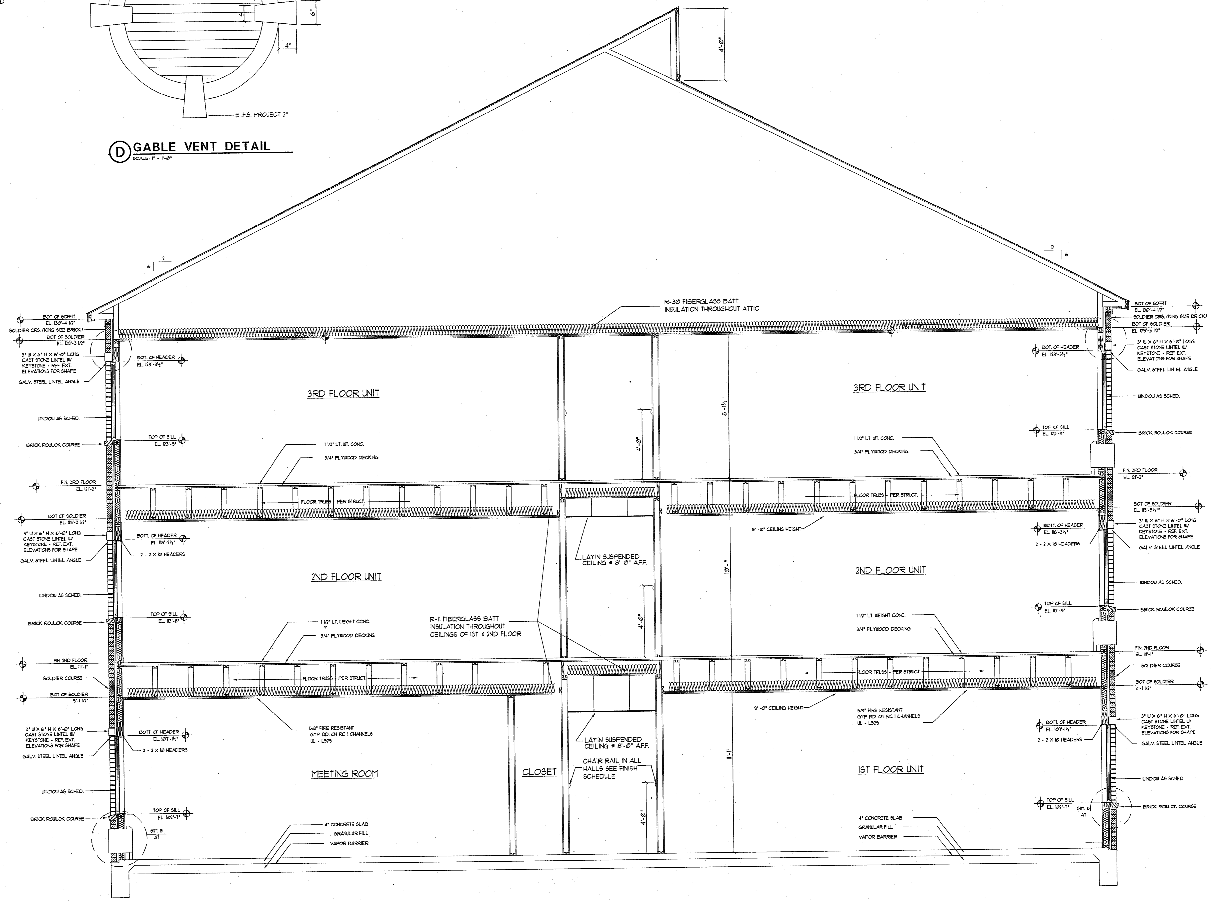
A BUILDING SECTION SCALE: 3/8" = 1'-0"
