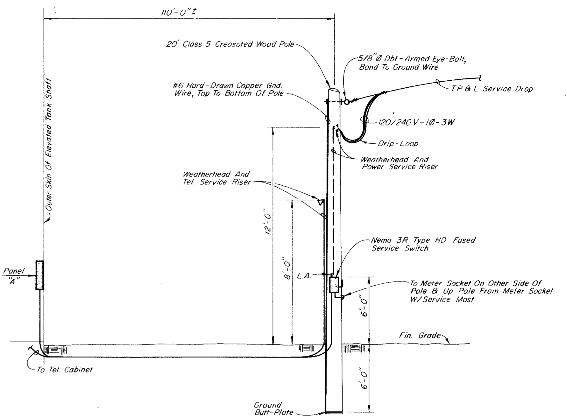
SERVICE ENTRANCE DETAIL No Scale
