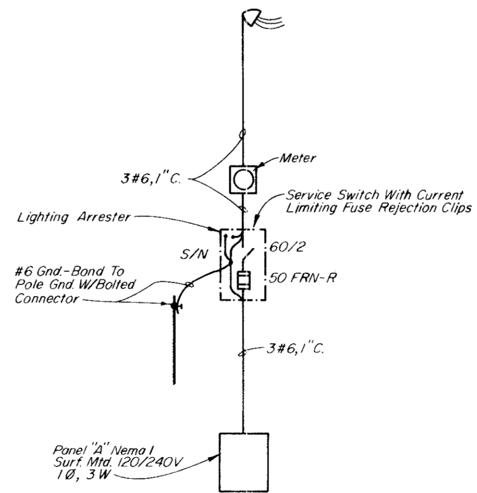
POWER RISER DIAGRAM No Scale
