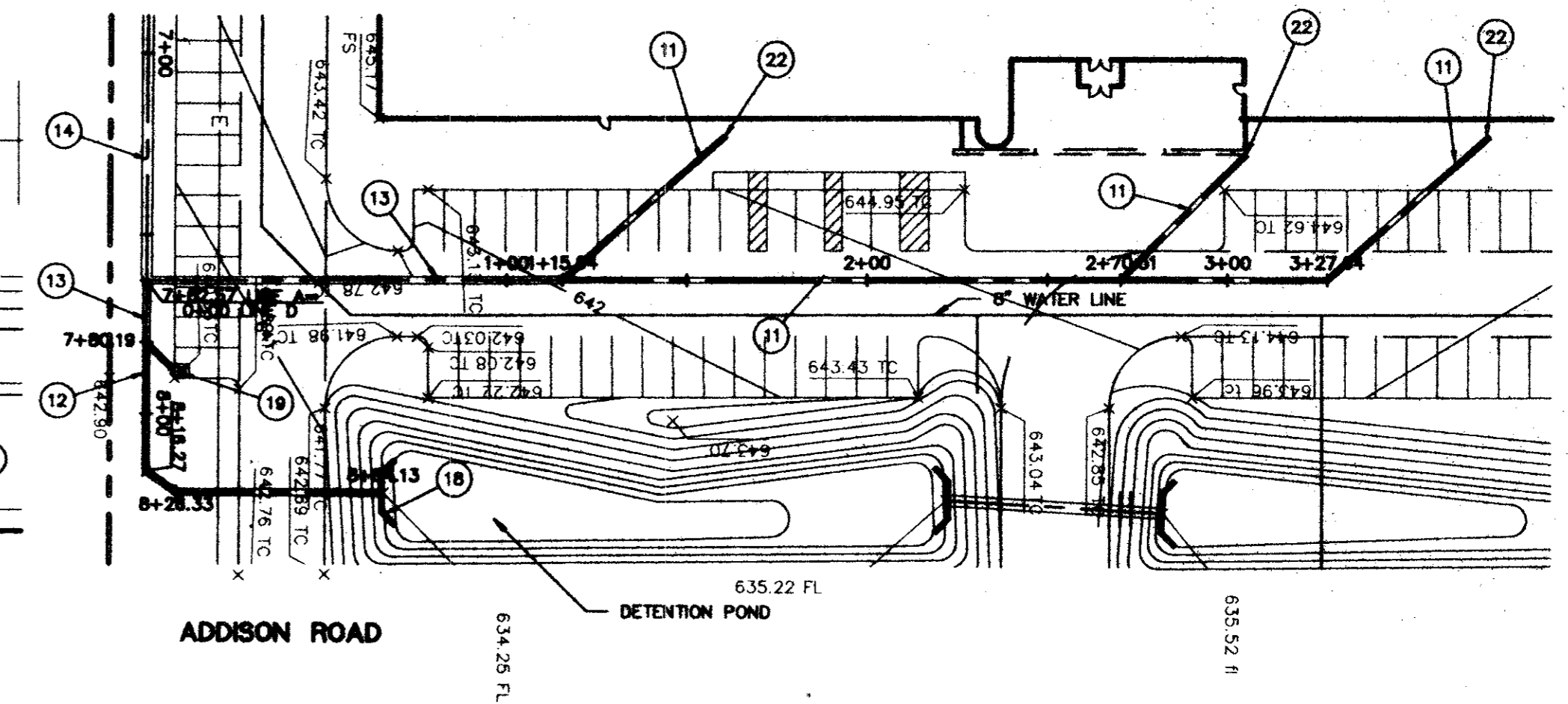
STORM DRAIN LINE "D"
