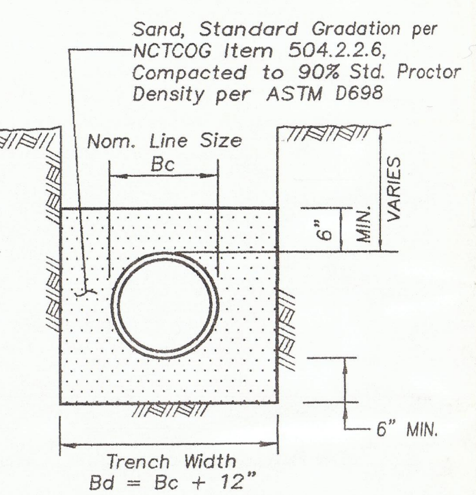
01 WATER MAIN EMBEDMENT NOT TO SCALE
