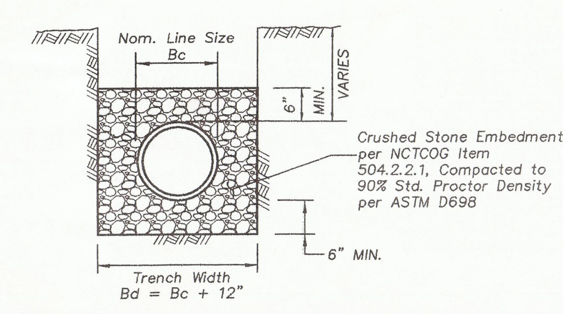
02 SANITARY SEWER EMBEDMENT NOT TO SCALE
