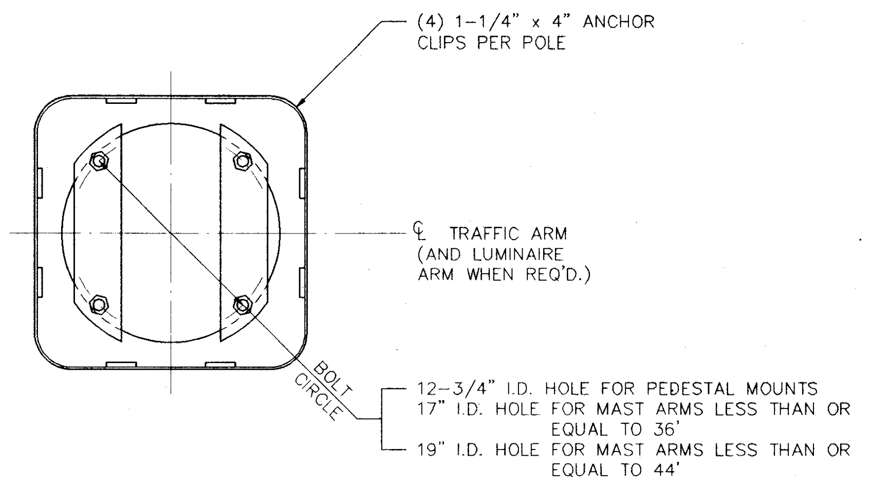
SECTION A
