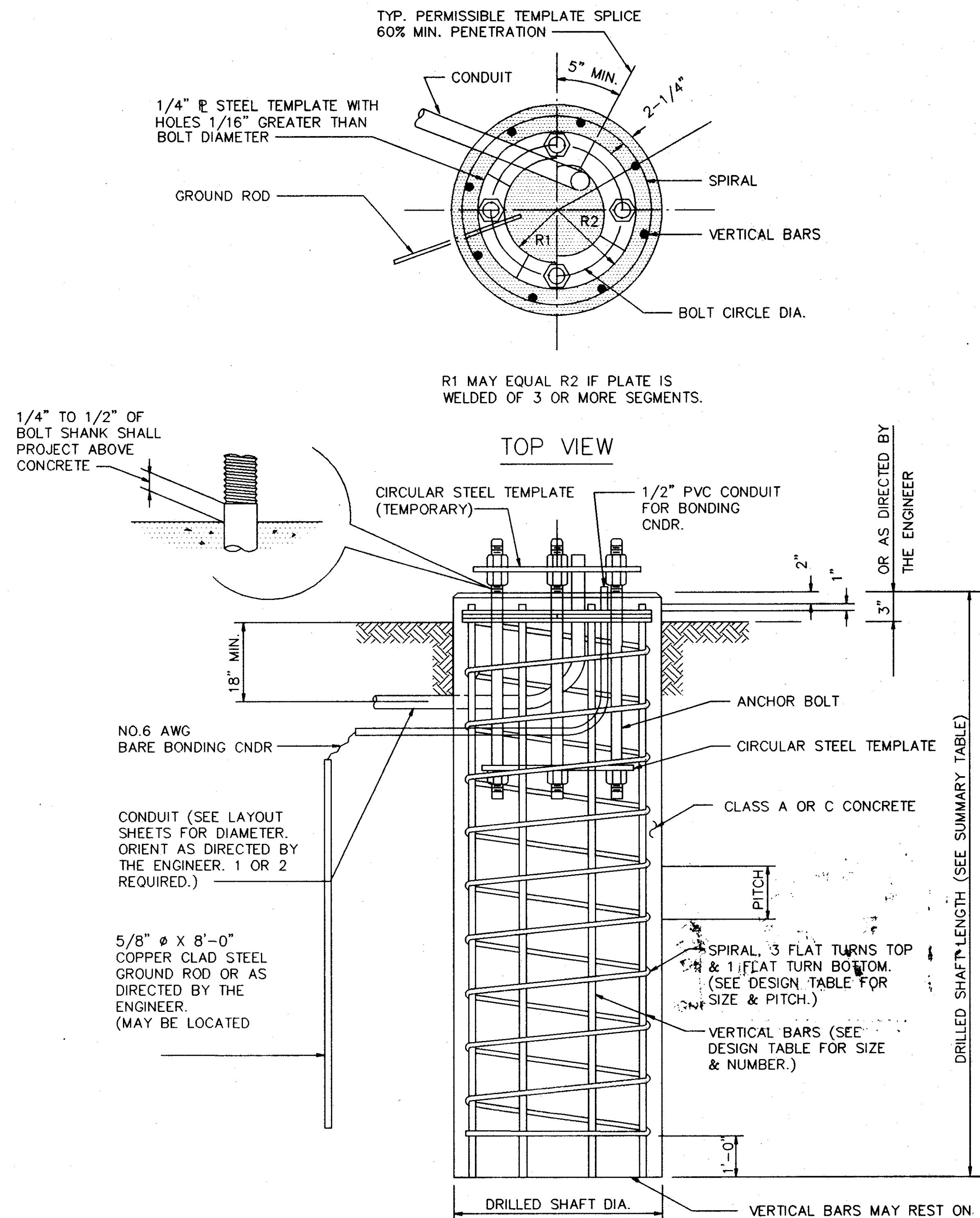
FOUNDATION DETAILS
