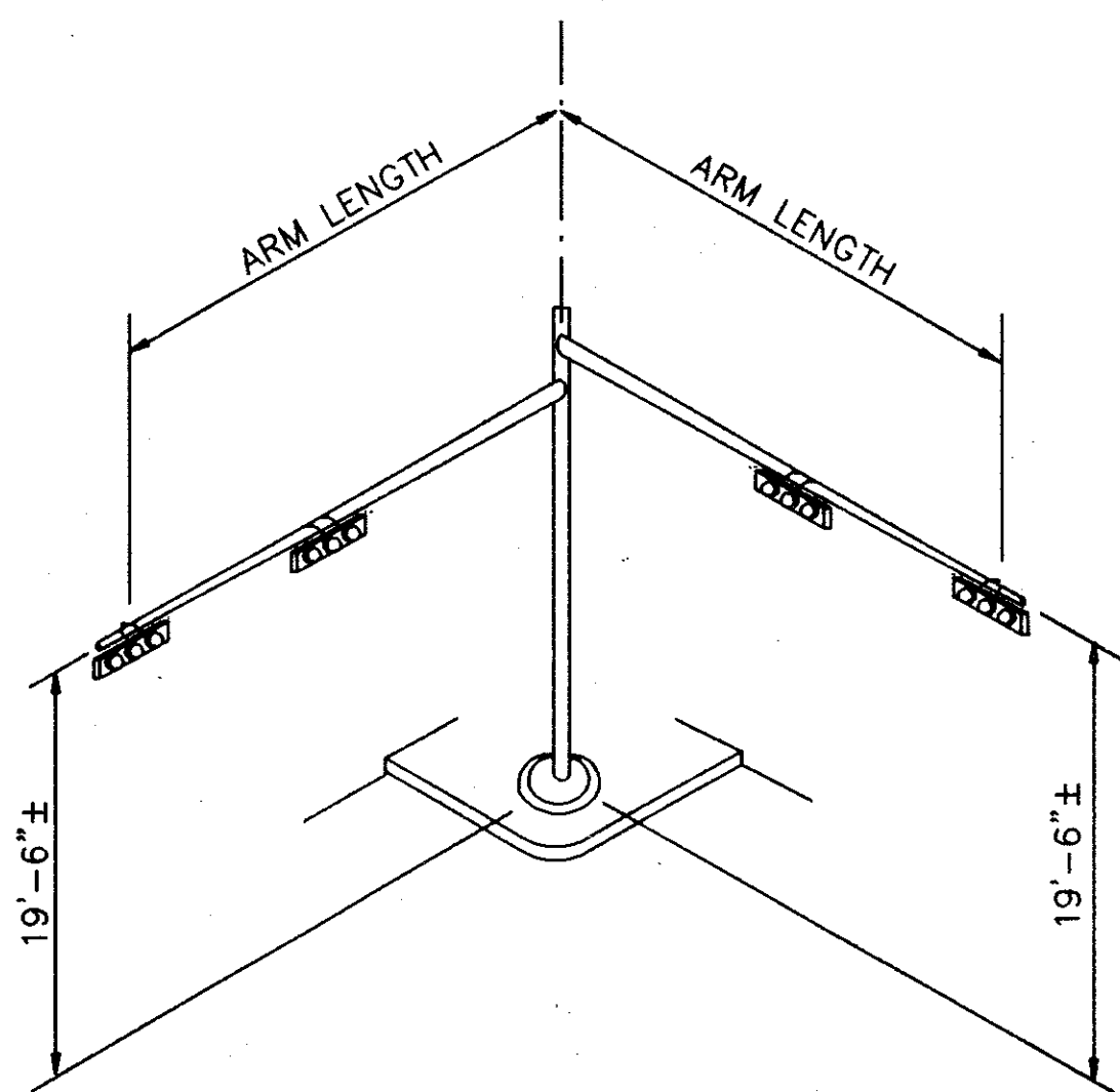
TYPICAL MAST ARM ASSEMBLY
