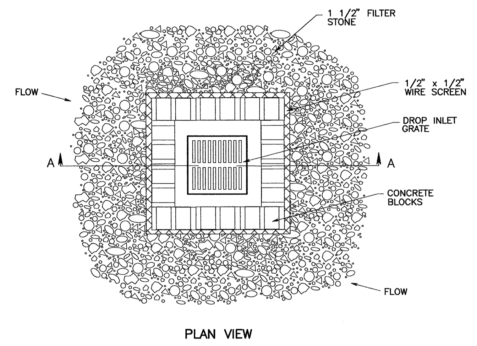
BLOCK/GRAVEL DROP INLET PROTECTION NTS
