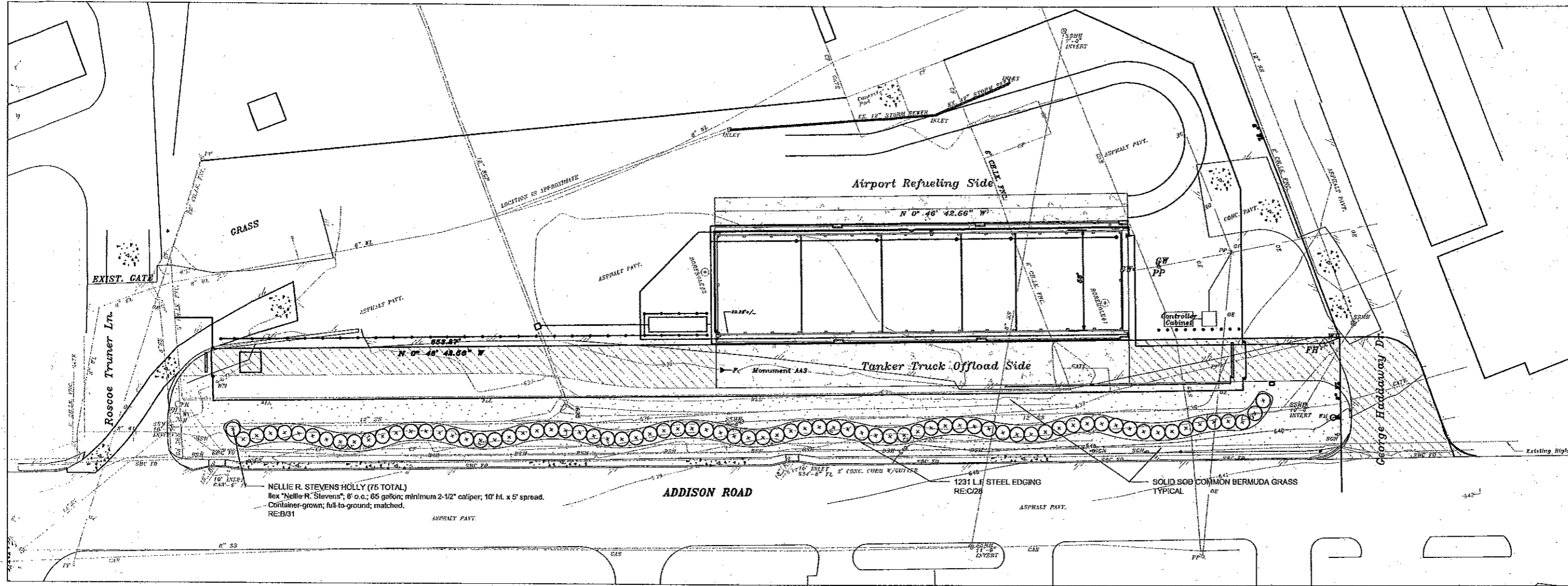
A LANDSCAPE PLAN SCALE: 1"=30'-0" 1 inch = 30ft.
